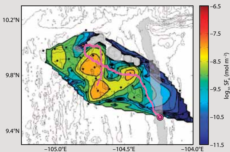
Figure B-1. Vertically integrated SF 6 concentrations ranging from 3.2 \times 10^{-7} to 3.2 \times 10^{-12} mol m -2 measured at conductivity, temperature, depth (CTD) stations (black dots) 42 to 52 days after the SF 6 was released on the ridge at 9.5°N (purple circle). The superimposed trajectory (purple) is a model estimate of the center of mass of the SF 6 over time. The East Pacific Rise and Lamont Seamounts are highlighted in gray.
