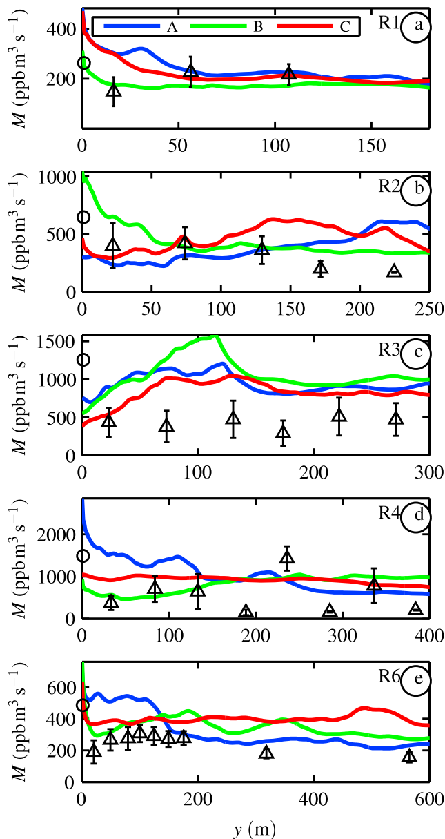
Figure 5. Modeled M^{(A,B,C)} (colored curved) and observed M^{(\text{obs})} (open black triangles with error bars) alongshore tracer transport (2) versus y , for releases (a) R1, (b) R2, (c) R3, (d) R4, and (e) R6. The observed dye release rate is estimated by the open black circle at y = 0 .
