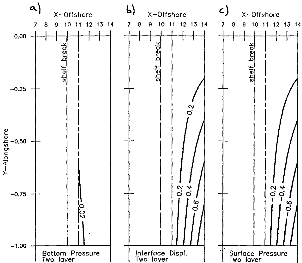
Figure 3-15: Solution for deep ocean forcing for a large value of R . ( R = 10, \delta_{rel} = 0.3, \Delta_s = 0, s_{rel} = 0.1, \Gamma' = 0 ). The interface intersects the continental slope. a) Very weak bottom flow, only contour is 0.02. b) Interface displacement. c) Isobars of upper layer pressure.
