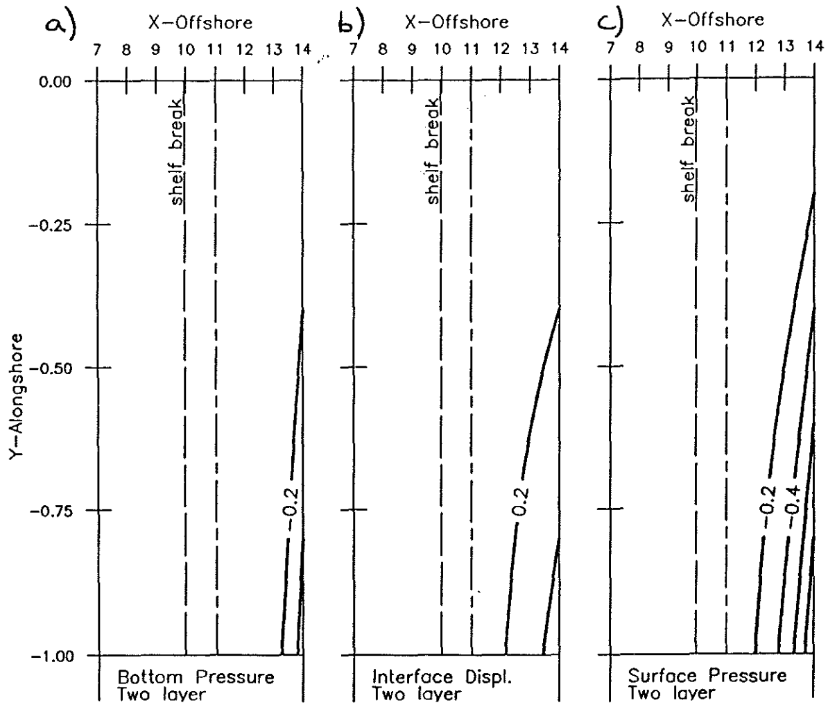
Figure 3-6: Flow induced by a baroclinic deep ocean when lower layer forcing is one half the strength of upper layer forcing ( R = 1.8 , \Delta_s = 0.1 , s_{rel} = 10 , \delta E_E^{rel} = 0.3 , \Gamma' = 0.5 ). Contour spacing is 0.2. a) Bottom layer pressure, minimum value -0.5 . b) Interface displacement. c) Upper layer pressure, minimum value -1.0 .
