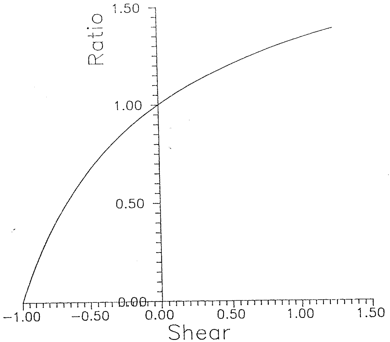
Figure A-2: Ratio which determines the degree of shelf penetration of the flow flow, plotted against the degree of shear in the flow's horizontal velocity ( Kh_0 ). The penetration of a barotropic flow is assumed to be unity. High ratios indicate more effective penetration of the shelf. If Kh_0 > 0 , the flow is more effective than a barotropic flow and if Kh_0 < 0 , it is less effective. The geostrophic velocity profile for different ranges of shear is shown schematically. The degree of flow penetration is zero when Kh_0 = -1 , corresponding to flow with zero near bottom velocities.
