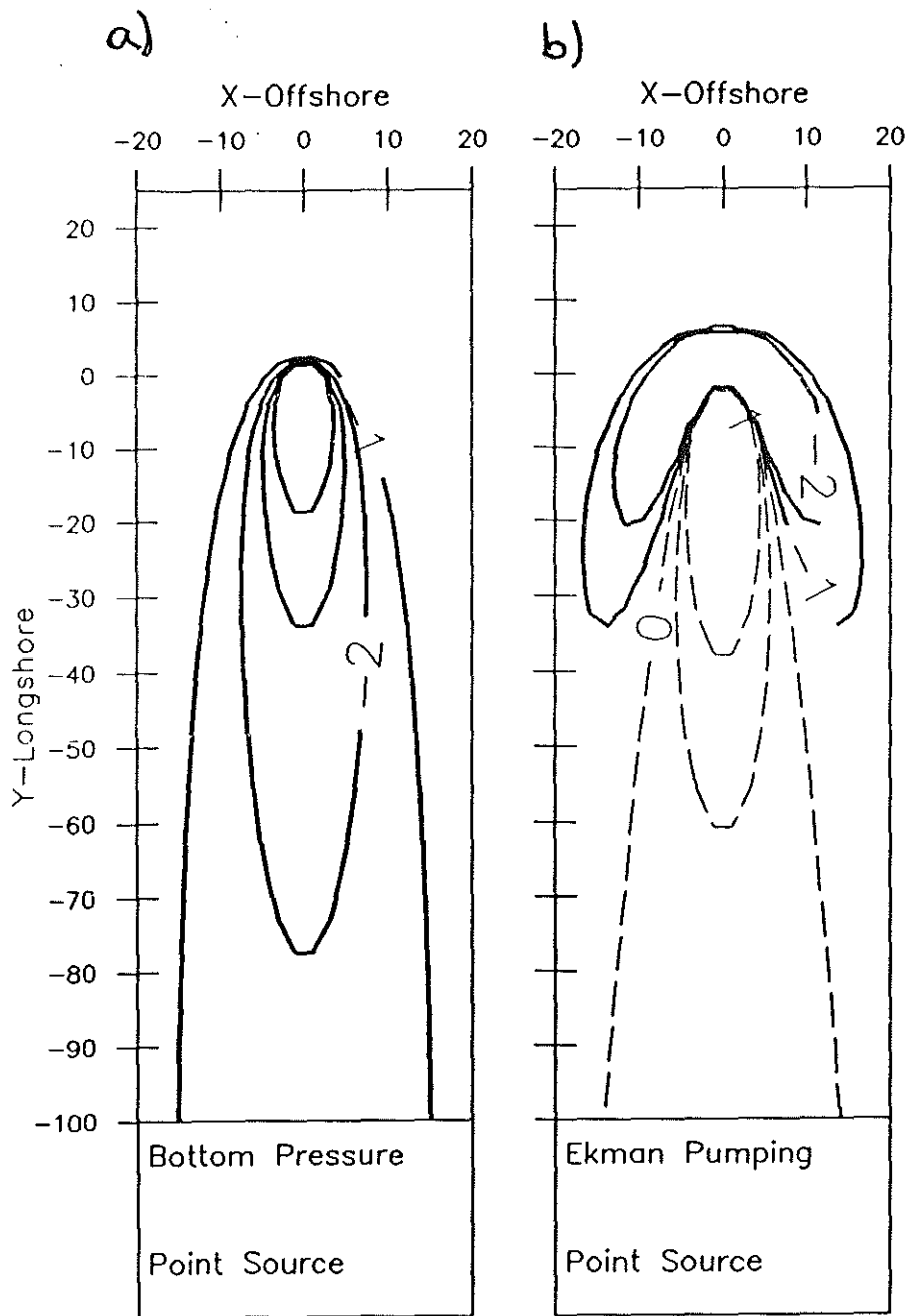
Figure 3-2: Isobars of bottom pressure for a point source in the lowest geostrophic layer (the Green's function solution to (3.30)). a) Solid contour spacing is 1 and pressure decreases monotonically towards the origin. Isobars are also flow lines for geostrophic flow in the lowest layer. b) Contours of Ekman pumping velocity. Contour spacing is 1. Solid contours are negative values, dashed contours, positive values. Ekman pumping velocity for the point source is downward in regions of upslope geostrophic flow and upward in regions of downslope flow. Contours near the origin are omitted because the solution is singular there.
