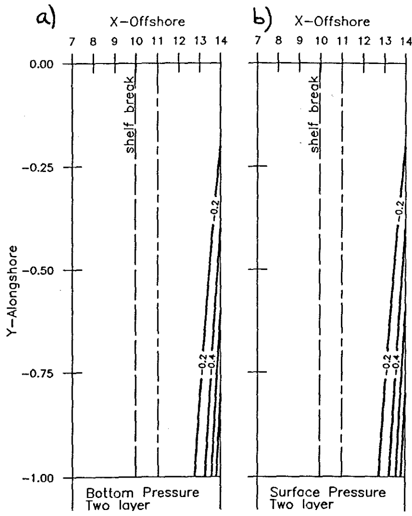
Figure 3-5: Pressure pattern in two-layer model due to barotropic deep ocean forcing of the shelf/slope ( R = 1.8 , \delta_E^{rel} = 0.3 , \Delta_s = 0.1 , s_{rel} = 0.1 , \Gamma' = 1 ). Contour spacing is 0.2, minimum value is -1 . Pressure contours are also flow lines for geostrophic flow in the layer cores. The labeled dashed line is the shelf break and the unlabeled chain dashed line is where the single interface intersects the bottom. a) Lower layer isobars. b) Upper layer isobars. The interface displacement is not plotted as it is zero for this barotropic flow.
