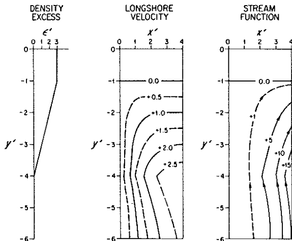
FIG. 1. (a) One-ramp alongshore density distribution, monotonically increasing northward. (b) Pattern of the longshore velocity v_b . (c) Pattern of the transport streamfunction \psi . Dimensionless units are discussed in Table 1.
