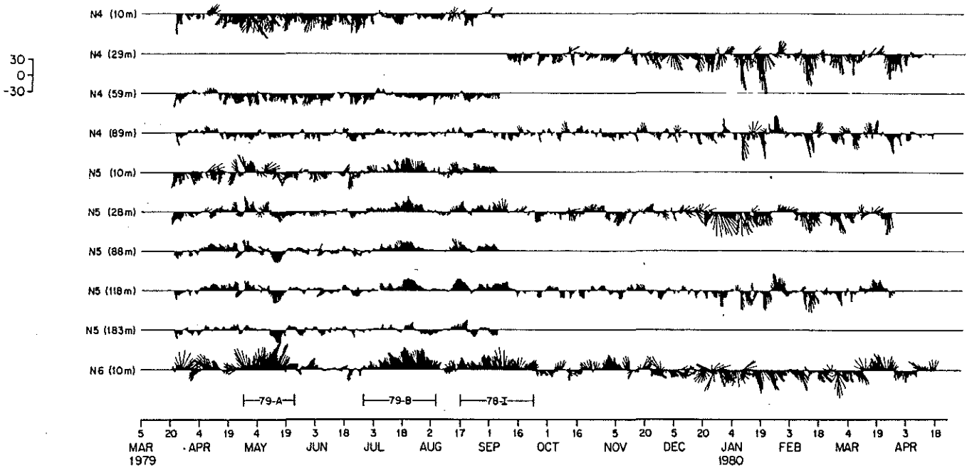
FIG. 8. Composite vector plots of the low-frequency NLS wind stress and currents measured in NSFE79. The positive alongshelf component of wind stress (oriented toward 77°T) and the positive alongshelf component of current (oriented towards 107°T) are both plotted up. All time series have been filtered with a low-pass filter with a half-amplitude period of 33 hours and subsampled every 6 hours.
