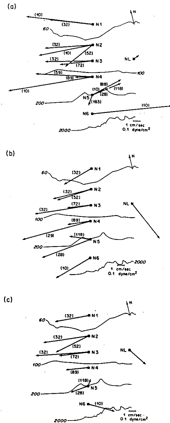
FIG. 10. Mean currents and wind stress computed over the (a) summer, (b) winter and (c) one-year periods. Instrument depth in meters is indicated in parentheses by the corresponding current vector, and the velocity and wind-stress scales are shown in the lower right of each panel. The 60, 100, 200, and 2000 m depth contours are also shown. Mean currents and stresses are tabulated in Table 3.
