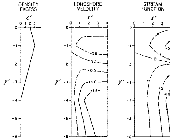
FIG. 2. (a) Two-ramp alongshore densities distribution with \beta' = -1 for -1 \leq y' \leq 0 . (b) Pattern of the longshore velocity v_b . (c) Pattern of the transport streamfunction \psi . Dimensionless units are discussed in Table 1.
