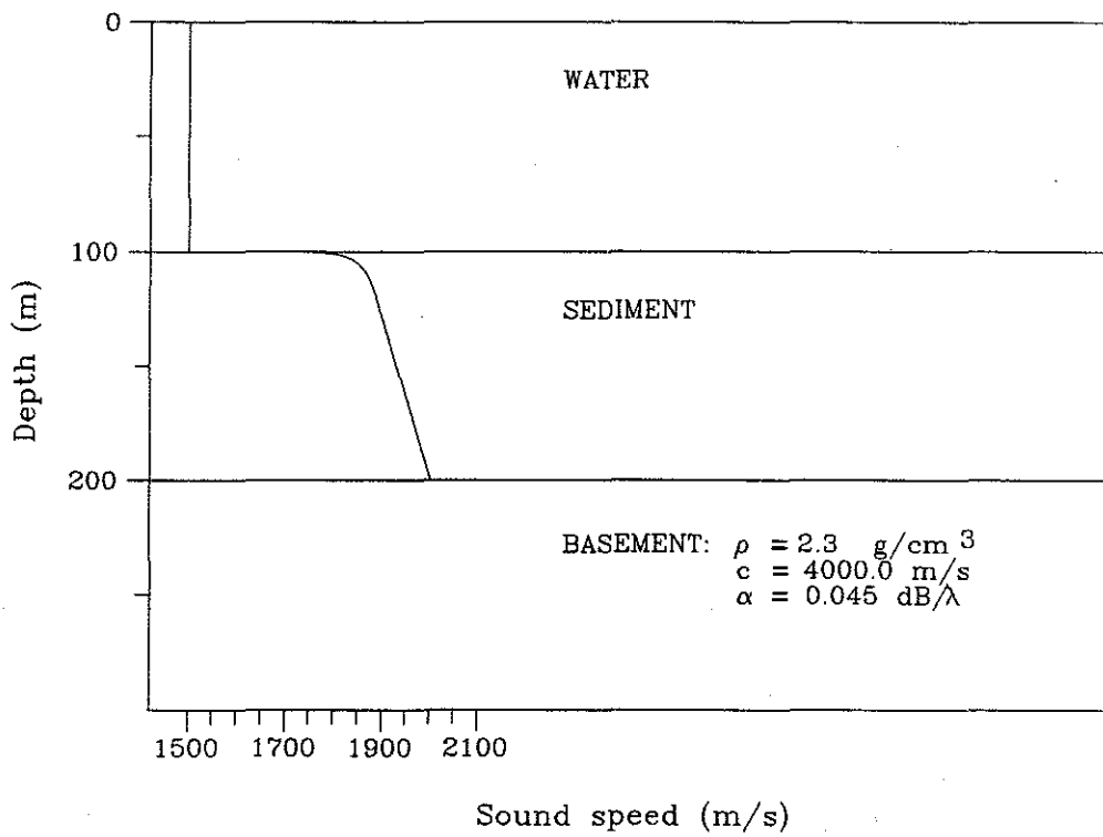
Figure 4-9: The shallow water waveguide model with a fine sand bottom.
