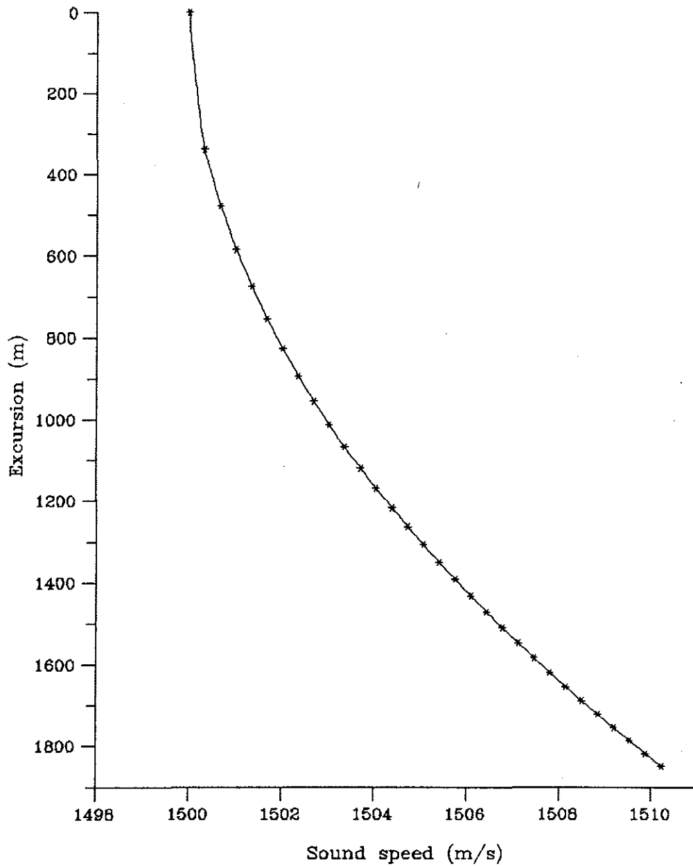
Figure 3-10: The excursion for the parabolic profile computed using inversion method 2. The excursion is the distance between points of equal sound speed on the two branches of the sound speed profile.
