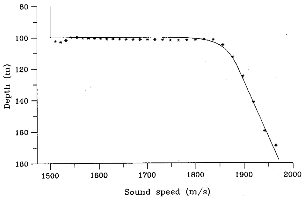
Figure 4-16: Inversion results for waveguide model 2 using inversion method 2 (smoothing splines).
