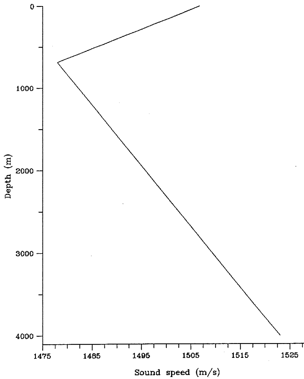
Figure 3-12: The bilinear sound speed profile model.
