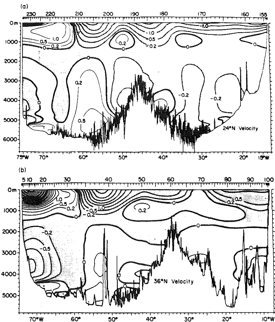
Fig. 9. (a) Horizontally smoothed geostrophic velocity ( cm\ s^{-1} ) at 24°N from 1981 data, based on the reference level calculation with constraints on total transport only. Southward velocities are shaded. The western end is on the left. (b) Same as (a) for 36°N.
