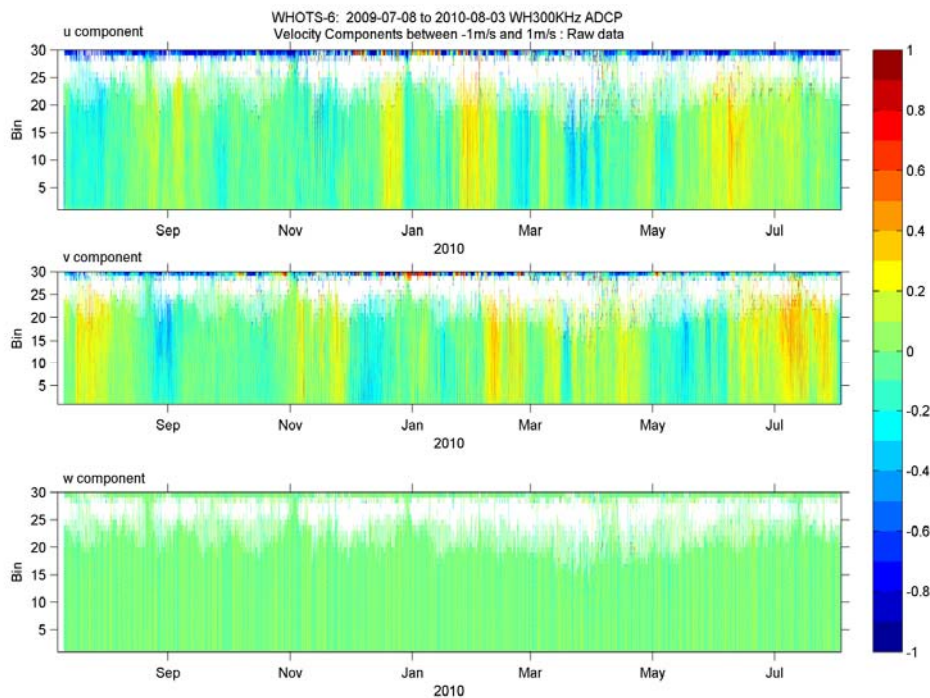
Figure 5-5: Time-series of eastward, northward and upward velocity components versus bin number measured by the ADCP at 125 m depth on the WHOTS-6 mooring. Height in meters above the transducer is approximately 4 times the bin number.
