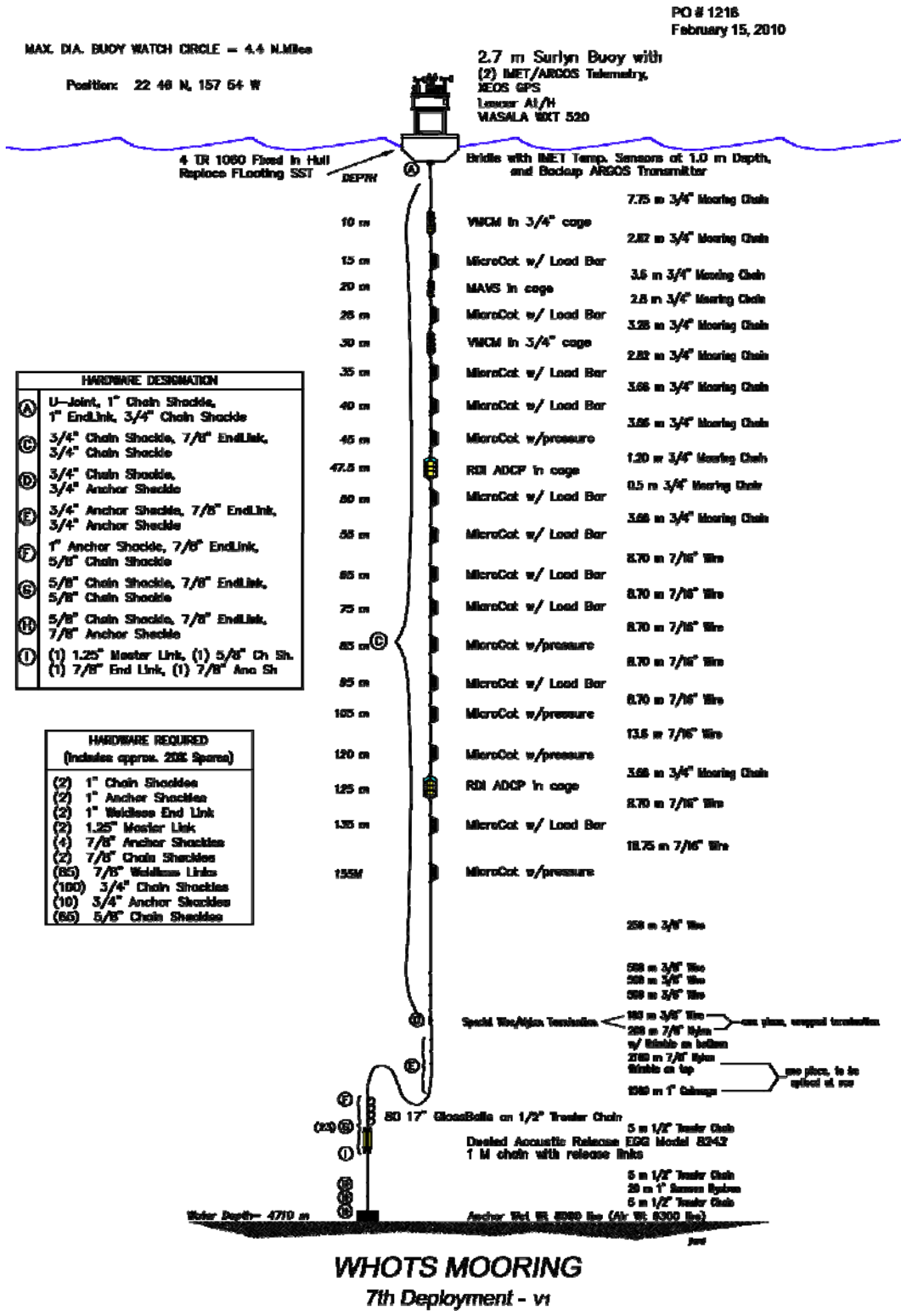
Figure 3-1: WHOTS 7 Mooring Design
