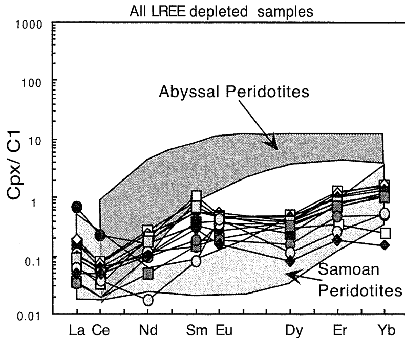
Figure 2-13. Summary of trace element abundances of LREE depleted samples. Fields for Samoan peridotites (Hauri and Hart, 1994) and abyssal peridotites (Johnson et al., 1990) are shown for comparison.
