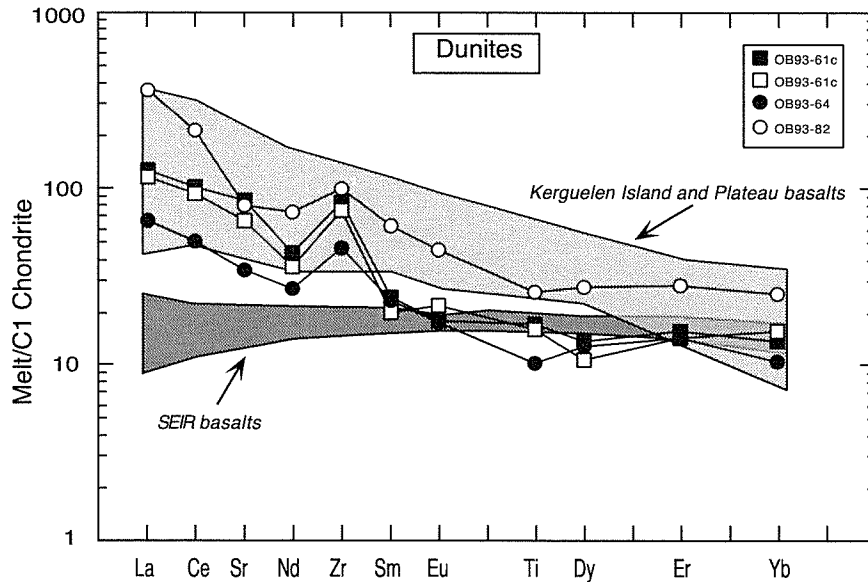
Figure 2-11. Chondrite-normalized REE abundances of melts in equilibrium with clinopyroxenes from lherzolite OB93-52 and from the wehrlitic-dunites. Abundances in Kerguelen basalts are shaded light gray, those from the SEIR are darker gray. Fields based on data from: (Davies et al., 1989; Alibert, 1991; Gautier et al., 1990; Weis et al., 1993; Yang et al., 1998a; Michard et al., 1986; Dosso et al., 1988).
