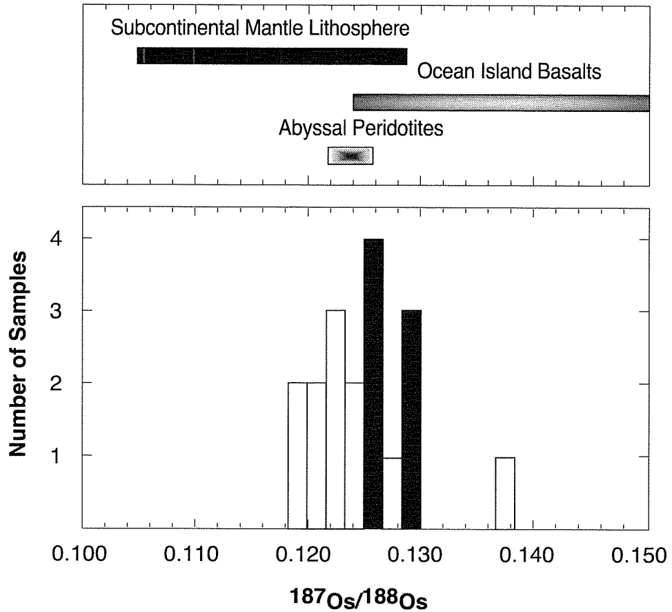
Figure 3-2. Histogram of the Os isotopic composition of the Kerguelen Islands peridotite xenoliths by location. Most samples from the Lac Superieur locality (black) are more radiogenic than most of those from the Mont Trapeze locality (white). The typical error is less than the width of a bar. Shown for comparison, is the range of initial Os isotopic compositions of other rock types from around the world (16, 19-24, 26, 27). Only data for abyssal peridotites that are not contaminated with seawater Os are shown.
