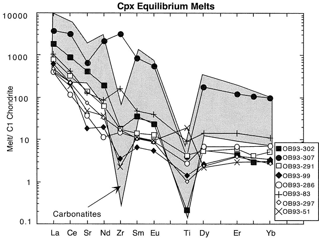
Figure 2-12. REE patterns of hypothetical melts that are similar to REE abundances observed in carbonatites (gray field; Nelson et al., 1988).
