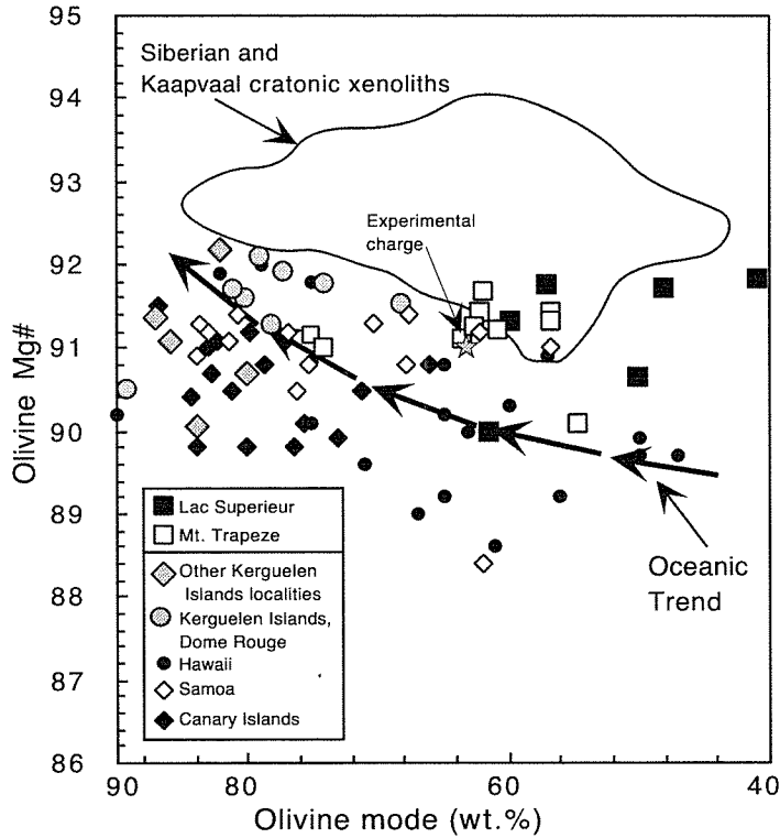
Figure 2–3. Oceanic trend diagram (after Boyd, 1989). Kerguelen samples of this study (Lac Superieur locality: filled squares, Mt. Trapeze open squares, and other Southeastern Province samples (Dome Rouge: gray circles and others: gray diamonds) are shown along with other oceanic samples (Hawaii: small filled circles, Samoa, small open diamonds, and the Canary Islands: small filled diamonds). The lherzolite (Lac Superieur sample OB93-52) plots on the oceanic trend, as do three of the Mt. Trapeze samples (OB93-287, OB93-289, OB93-297). The remaining samples of this study, and some samples from the Southeast Province, Hawaii, Samoa, and one from the Canary Islands lie above the oceanic trend, some even extending into the field defined by Siberian and Kaapvaal cratonic xenoliths. Fields and data from Boyd (1989), Boyd et al. (1997), Kelemen et al. (1998), Grègoire (1994), Hauri and Hart (1994), Sen (1988), and Wulff-Pedersen et al. (1996).
