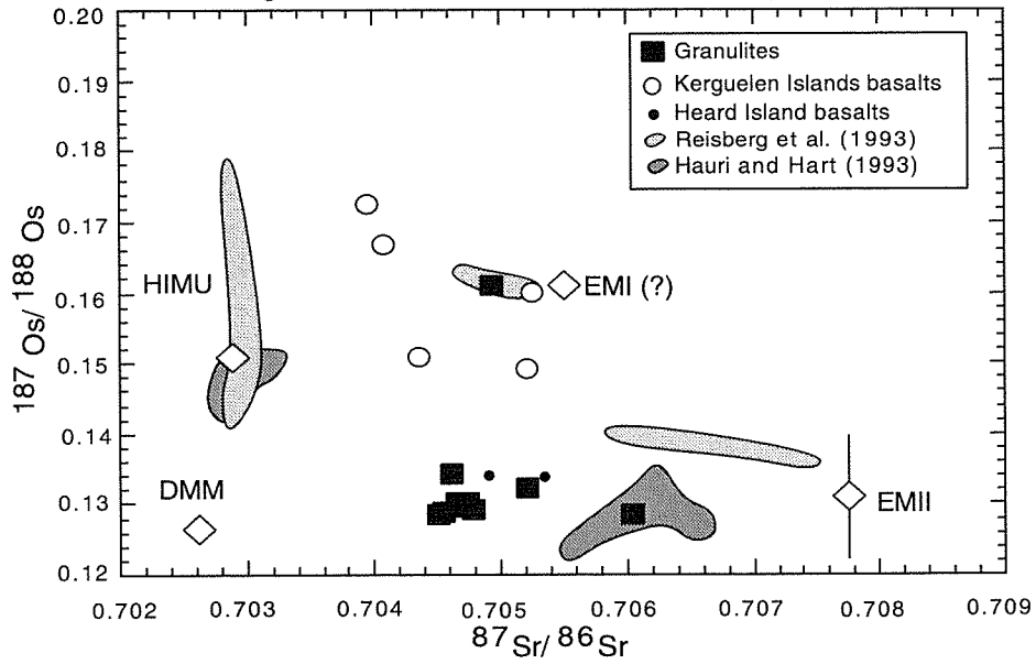
Kerguelen Granulites and basalts, eruption-age corrected
