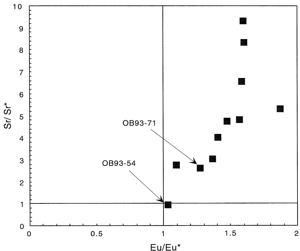
Figure 4-13. Granulite whole rock Sr/Sr^* v Eu/Eu^* . Sr^* and Eu^* are interpolated from the concentrations (in ppm) of the neighboring trace elements ( Sr^* = (Nd + Sm)/2 and Eu^* = (Sm + Gd)/2 ). All samples, except OB93-54 have both Sr^* and Eu^* > 1 , indicating a cumulate protolith. Sample OB93-54 is also interpreted as a cumulate, as discussed in the text.
