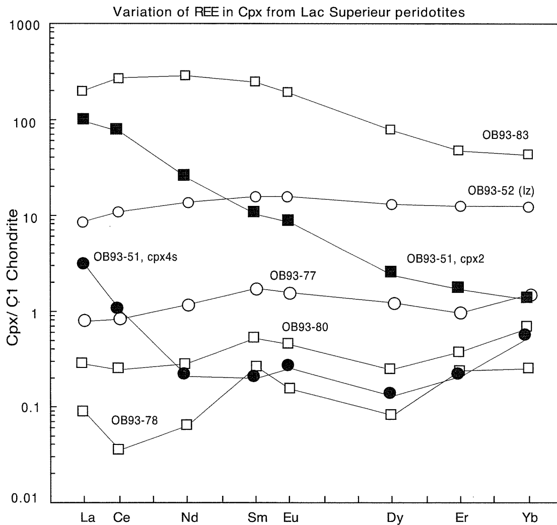
Figure 2-6. Range of clinopyroxene REE compositions from the Lac Superior locality. Open symbols represent grains from individual rocks, closed symbols are from a single xenolith (OB93-51).
