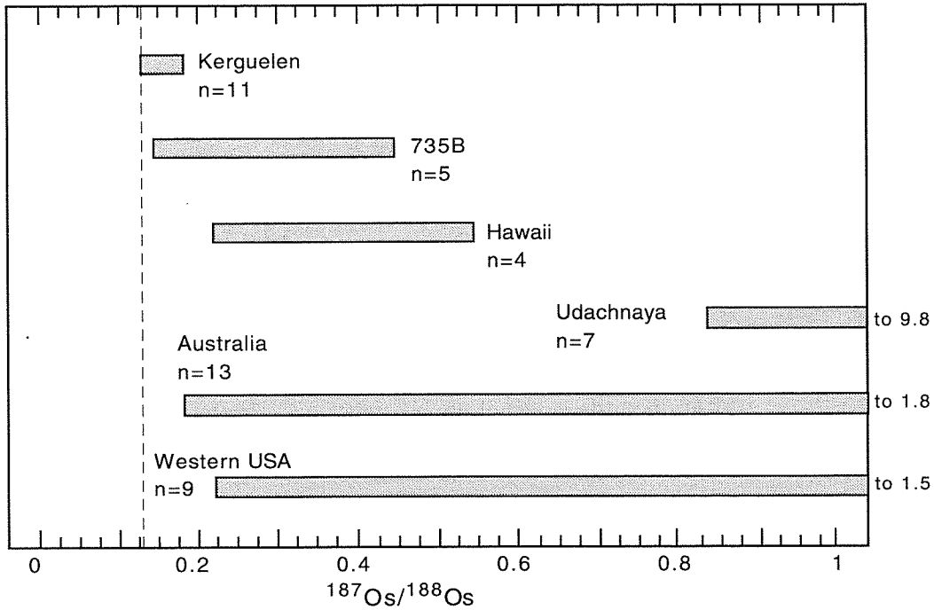
Figure 4–20. Comparison of the present day values of the ^{187}\text{Os}/^{188}\text{Os} and ^{187}\text{Re}/^{188}\text{Os} of all lower crustal xenoliths analyzed to date. The location and number of samples in each dataset are noted next to each bar. Present-day primitive mantle values are shown as a broken line in each panel. The Kerguelen granulites have a limited range of these values, especially ^{187}\text{Re}/^{188}\text{Os} , relative to the other analyzed samples. Comparison data are from Hart et al. (1999), Lassiter et al. (1998), Pearson et al. (1995), Saal et al. (1998), and Esperança et al. (1997).
