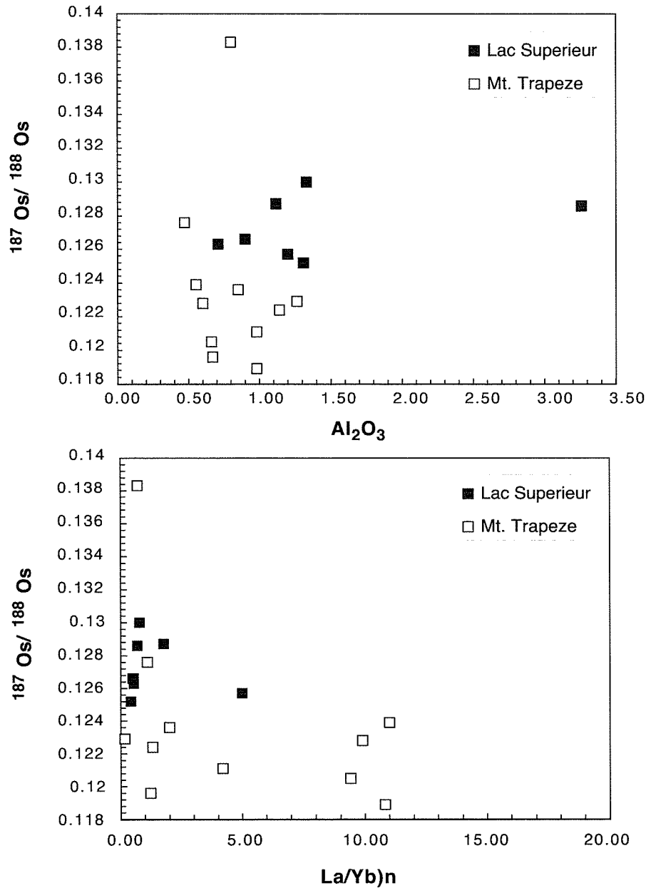
Figure 2-21. Whole rock Os isotopic compositions v. whole rock \text{Al}_2\text{O}_3 (upper panel) and clinopyroxene [\text{La/Yb}]_n (lower panel). No correlations are present among these parameters, indicating that metasomatism did not affect the Os isotopes.
