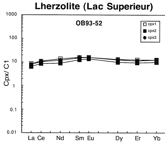
Figure 2-16. Normalized REE patterns of the Iherzolite.
