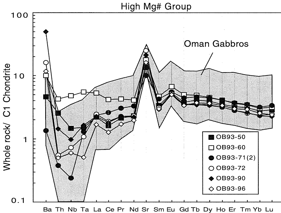
Figure 4-11. C1 chondrite normalized REE abundances of clinopyroxenes and bulk rocks. Whole rock patterns (filled squares) are shown along with clinopyroxene patterns. Each
