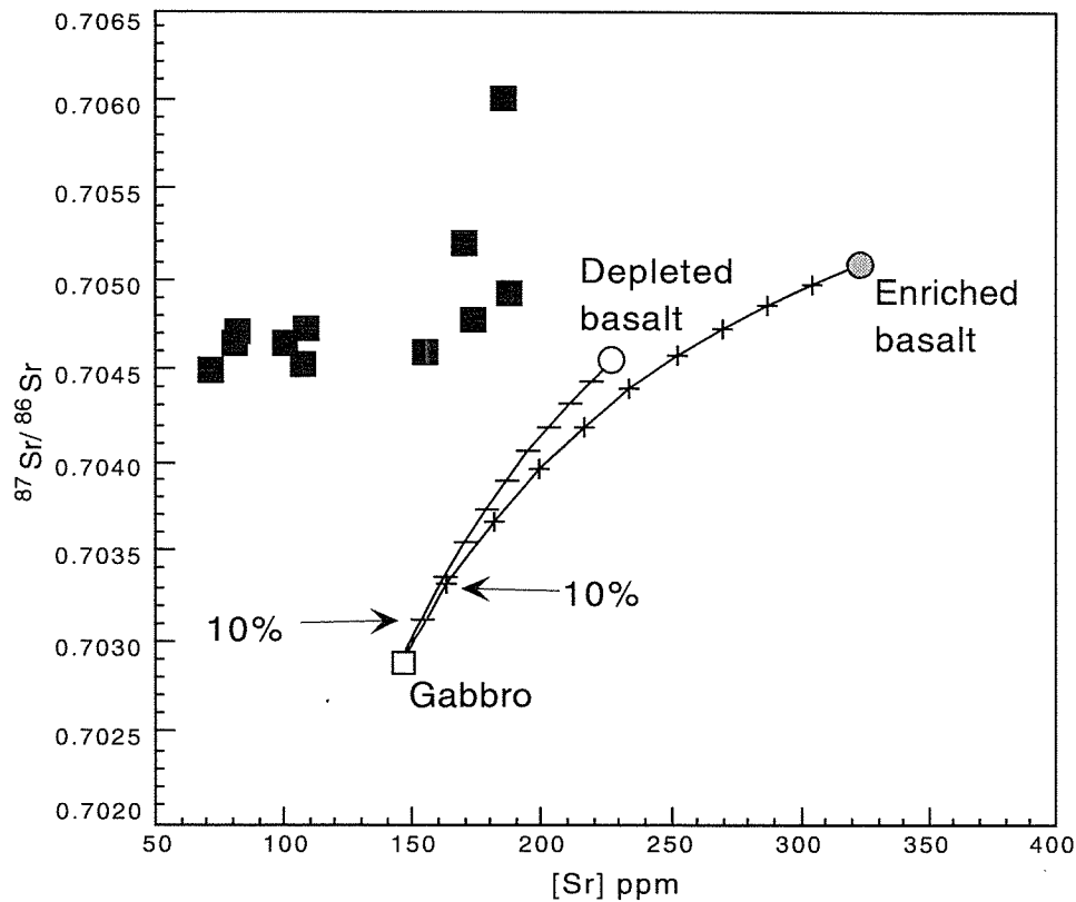
Figure 4-14. Strontium isotopic composition v. [Sr] (ppm). Bulk rock compositions of granulites are compared to those of two component mixtures of a calculated SEIR basalt equilibrium gabbro and two Kerguelen Islands basalts. The possibility of an oceanic olivine gabbro adcumulate (open square) impregnated with Kerguelen OIB (open and gray circles) as a protolith for the granulites (filled squares) is illustrated in this figure. Mixtures of the gabbro with a REE depleted basalt (-) and REE enriched basalt (+) are shown. Symbols mark the melt fraction in 10% increments. On the basis of this calculation, the granulites could not have originally been a mixture of lower oceanic crust and Kerguelen OIB. The basalt data is from Yang et al. (1998). The gabbro data is calculated from a SEIR basalt from Dosso et al. (1988) using gabbro modes of 13.5% olivine, 31.5% clinopyroxene and 55% plagioclase, and Sr partition coefficients from Dunn and Sen (1994) and Hart and Dunn (Hart and Dunn, 1993).
