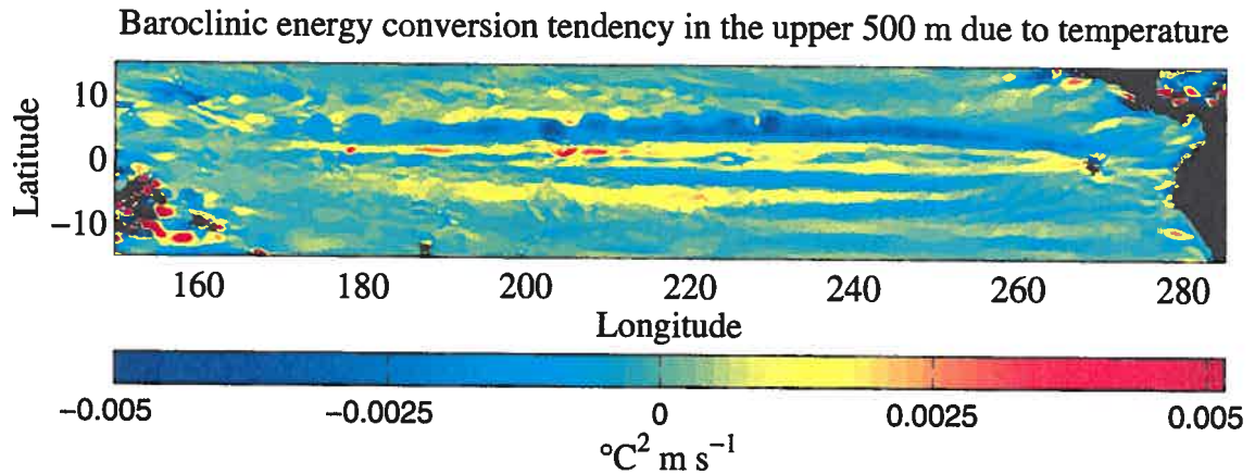
Figure 4.26: Eddy potential energy conversion tendency due to temperature, estimated by the depth integral of \overline{\mathbf{v}'\theta'} \cdot \nabla\bar{\theta} over the upper 500 meters. Negative values correspond to a conversion of mean flow energy to eddy potential energy, and positive values indicate a conversion of eddy potential energy to the mean flow energy.
