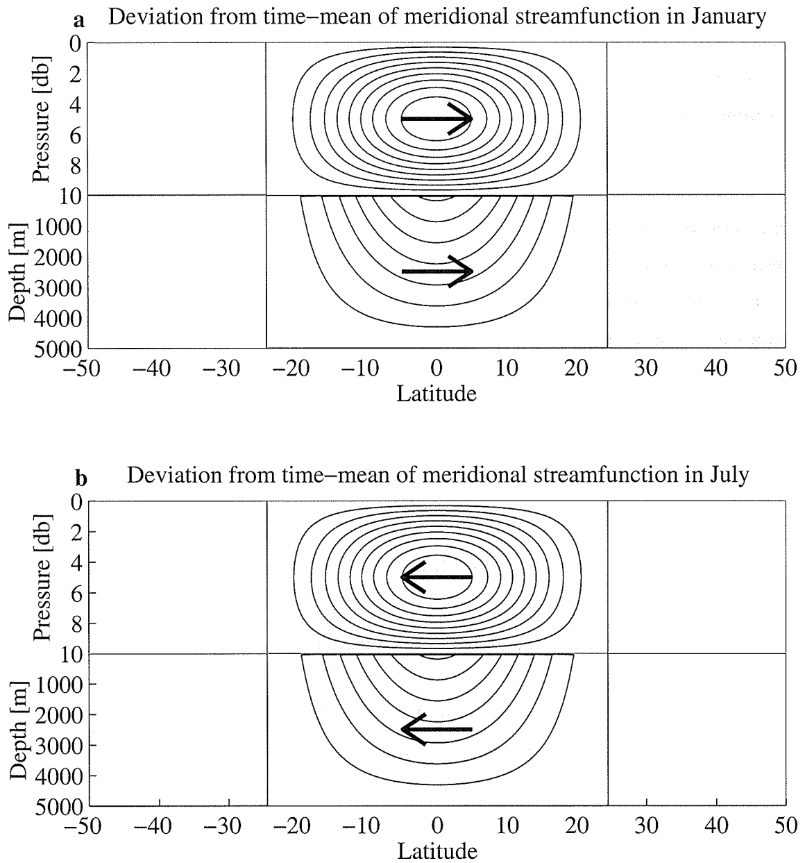
Figure 3.20: (a) The zonally-averaged meridional streamfunction for the atmosphere (upper half of the panel) and the zonally-averaged meridional streamfunction for the ocean (lower panel) for the January anomaly from the time-mean of the tropical atmospheric ocean circulation, (b) The same, but for July anomaly. The arrow indicates the direction of the total atmospheric energy transport and ocean heat transport. Negative values of the streamfunction are shaded gray and indicate counterclockwise overturning.
