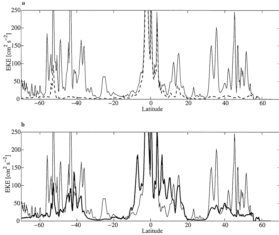
Figure 2.2: EKE along 200^{\circ}\text{E} for forcing with (a) once per 3 days uninterpolated wind stress (thin solid line) and with once per 3 days linearly interpolated forcing (dashed line) and (b) once per day linearly interpolated forcing (heavy solid line). EKE is in \text{cm}^2\text{s}^{-2} .
