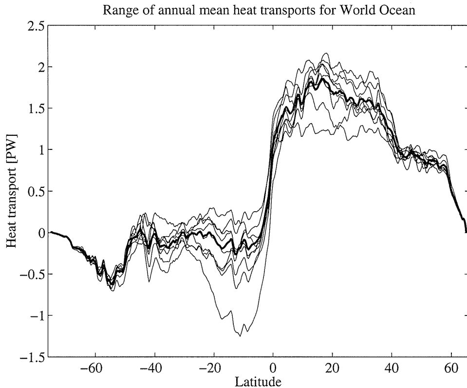
Figure 4.2: Annual mean heat transport for each year between 1988–1996 (thin solid lines) and mean of annual means (heavy solid lines).
