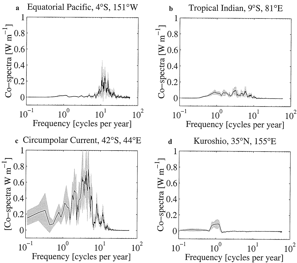
Figure 4.27: Co-spectra of temperature and velocity at 4 selected locations: (a) Equatorial Pacific Ocean, (b) Tropical Indian Ocean, (c) Antarctic Circumpolar Current, and (d) the Kuroshio Current.
