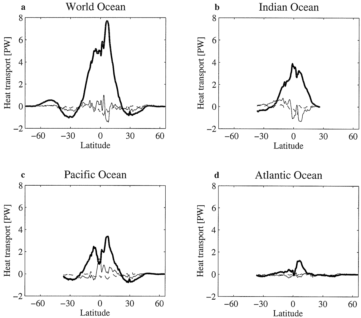
Figure 4.12: Annual cycle of heat transport associated with gyre circulation (dashed line), Ekman circulation (heavy solid line) and baroclinic shear flow (thin solid line) for the World Ocean, and the 3 ocean basins.
