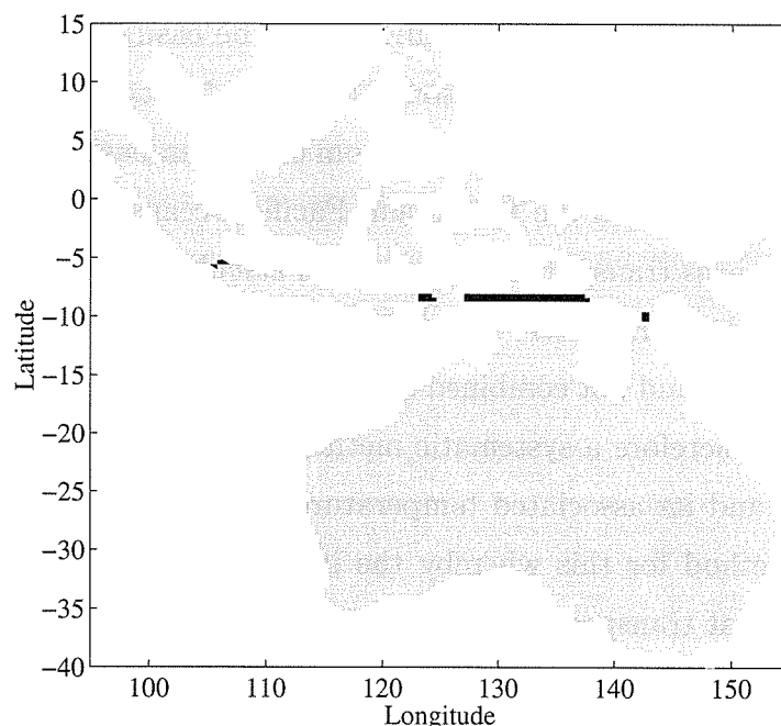
Figure 3.15: Geographical view of the Indonesian throughflow for POCM 1/4° resolution model. The 4 gaps which the throughflow was calculated are shown in black.
