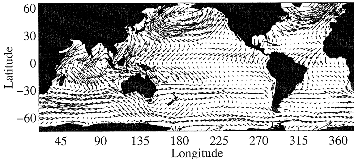
Seasonal cycle of the wind stress (January – July)
