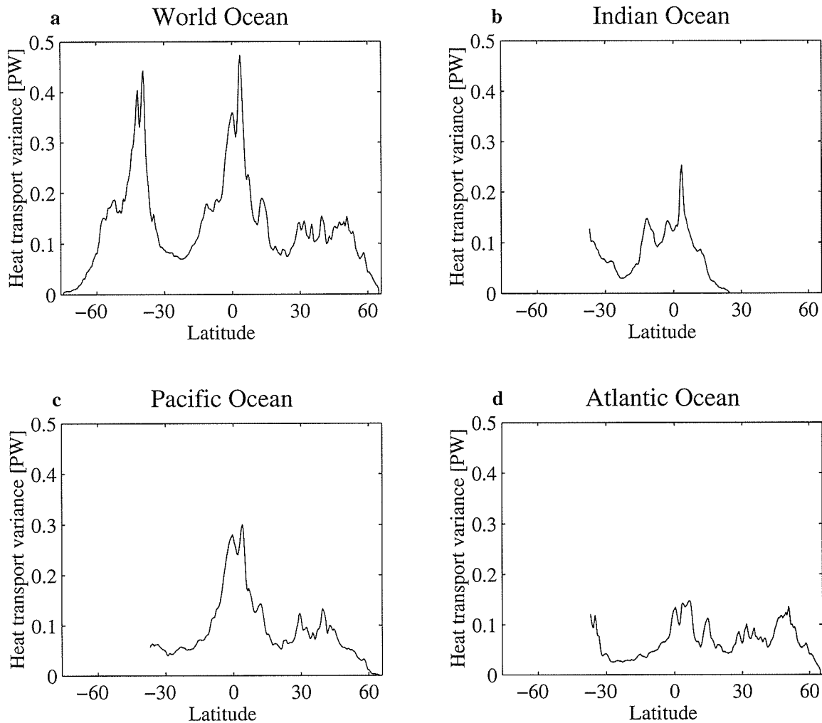
Figure 4.14: Root-mean-square variability of heat transport due to temporal changes in internal structure for (a) the World Ocean, (b) the Indian Ocean, (c) the Pacific Ocean and (d) the Atlantic Ocean. The square root of the variance is in units of petawatts.
