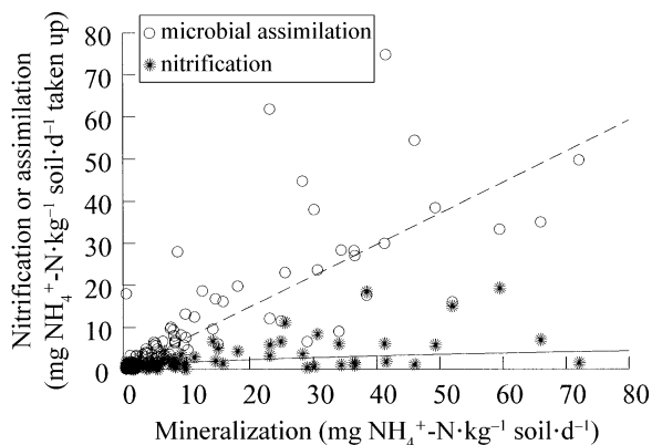
FIG. 6. Relationships of nitrification and microbial \text{NH}_4^+ assimilation to N mineralization in untransformed data. Trendline equations: \text{NH}_4^+ assimilation = 0.706 \times (\text{mineralization})^{1.03} , R^2 = 0.86 , P < 0.001 ; nitrification = 0.628 \times (\text{mineralization})^{0.49} , R^2 = 0.36 , P < 0.001 .
