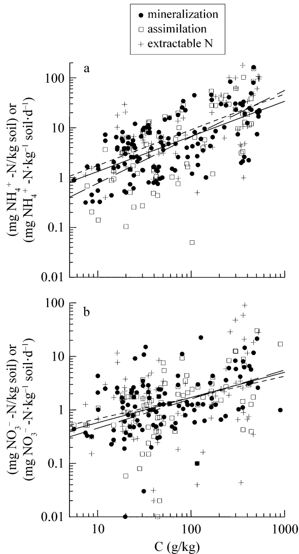
FIG. 4. For \text{NH}_4^+ and \text{NO}_3^- , the relationships of production (circles, solid line), assimilation (squares, large dashed line), and extractable inorganic N (crosses, small dashed line) to soil C. See Table 3 for regression equations and statistics.
