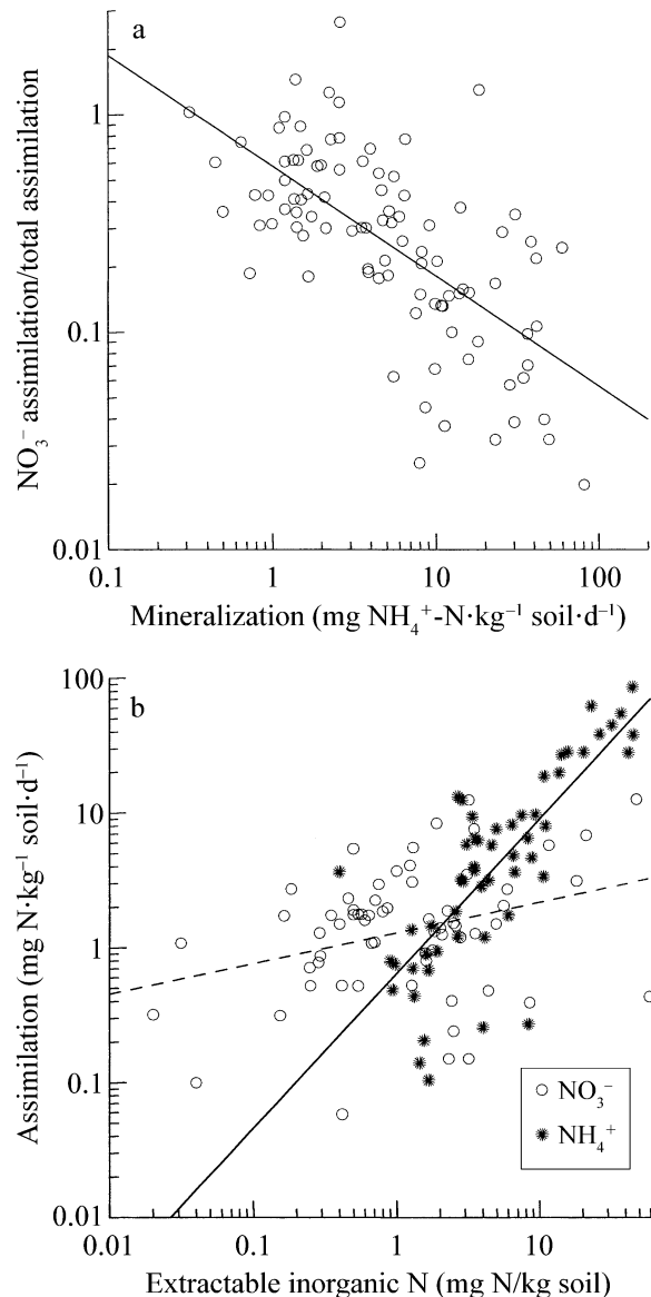
FIG. 5. (a) The relationship between the proportion of total assimilation comprised by \text{NO}_3^- assimilation and mineralization [ \log(\text{NO}_3^- \text{ assimilation}/\text{total assimilation}) = -0.51 \times \log \text{mineralization} - 0.23 ; n = 96 , R^2 = 0.43 , P < 0.00001 ] and (b) the relationship between assimilation and inorganic N concentration (as \text{NH}_4^+ or \text{NO}_3^- , respectively), in mineral and organic soil.
