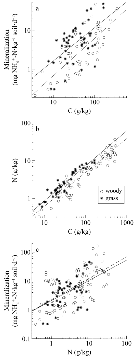
FIG. 9. The relationships between (a) mineralization and soil C, (b) N and soil C, and (c) mineralization and soil N for mineral soil from grassland and woodland ecosystems.
