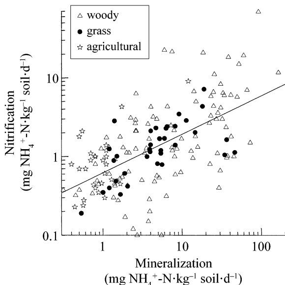
FIG. 2. Relationship of nitrification to N mineralization in mineral and organic soil layers from agricultural, grassland, and woodland ecosystems. See Table 3 for regression equations and statistics.
