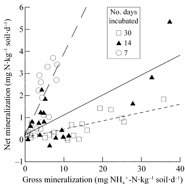
FIG. 7. The relationship between net and gross N mineralization rates for net mineralization studies with incubations of 7 (long dashed line), 14 (solid line), or 28–30 d (short dashed line). Gross rates incubations lasted 24, 48, or 120 h. Because incubation period for net mineralization was partially confounded with vegetation type, slopes were not statistically compared.
