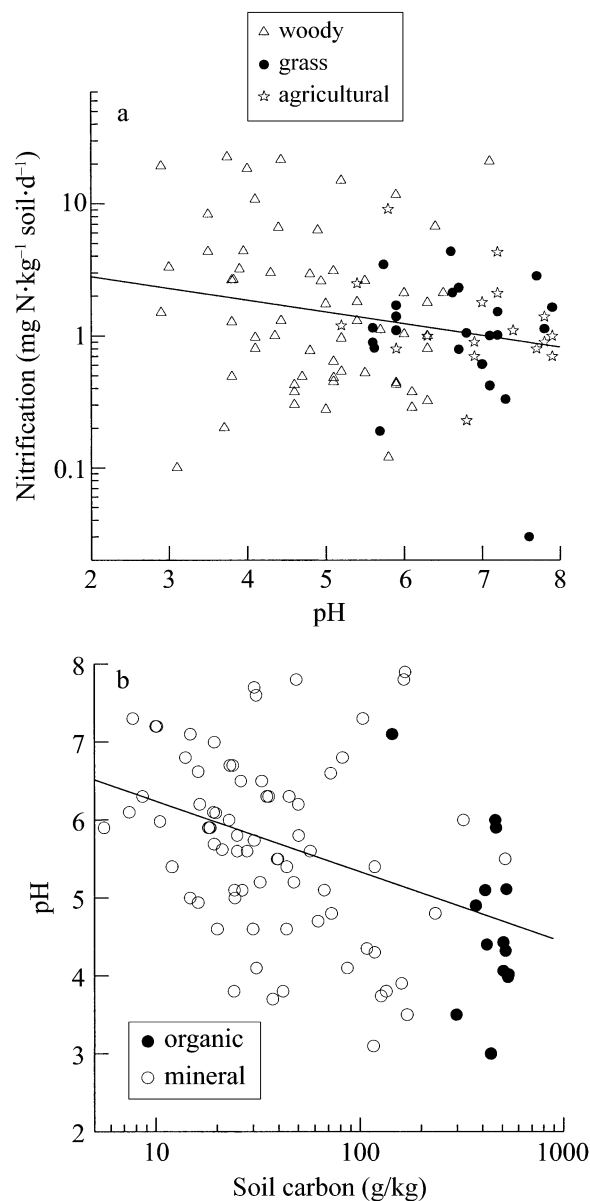
FIG. 3. (a) Relationship of nitrification to pH in mineral and organic soil layers from agricultural, grassland, and woodland ecosystems. See Table 3 for regression equations and statistics. (b) Relationship of pH to soil C concentration.
