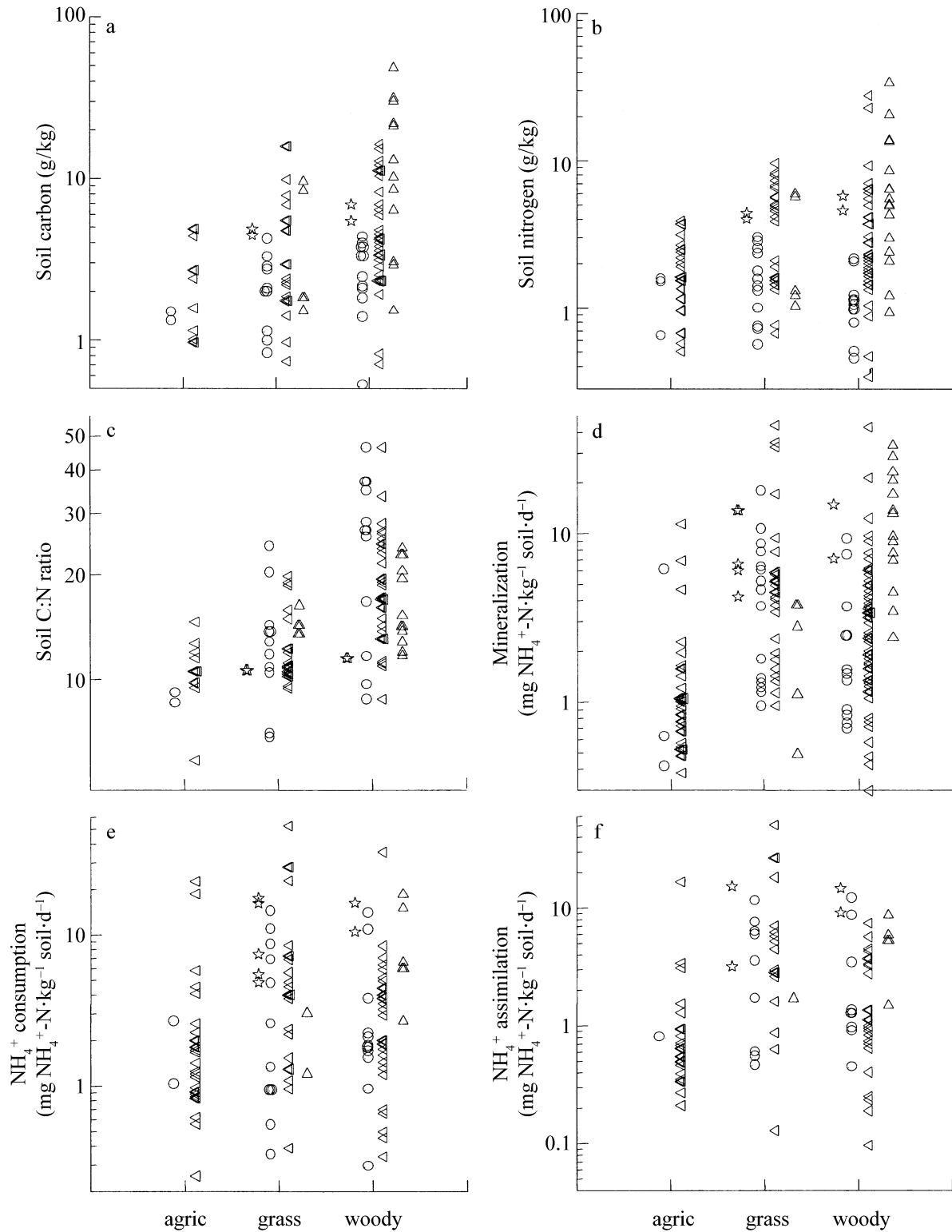
FIG. 8. Comparison of soil characteristics and gross rates in mineral soils of agricultural, grassland, and woodland ecosystems. Data from tropical forest soils were included to illustrate the range of values for forest soils of different climates but were not used in statistical comparisons among vegetation types.
