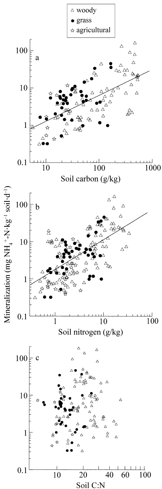
FIG. 1. Relationships of gross N mineralization to: (a) total carbon concentration, (b) total nitrogen concentration, and (c) C:N ratio, in mineral and organic soil layers from agricultural, grassland, and woodland ecosystems. See Table 3 for regression equations and statistics.
