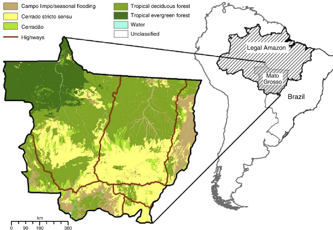
FIG. 1. Mato Grosso study area in Brazil, shown with potential natural vegetation classes (after Mello [2007] and derived from state government records [SEPLAN-MT 2007]).
