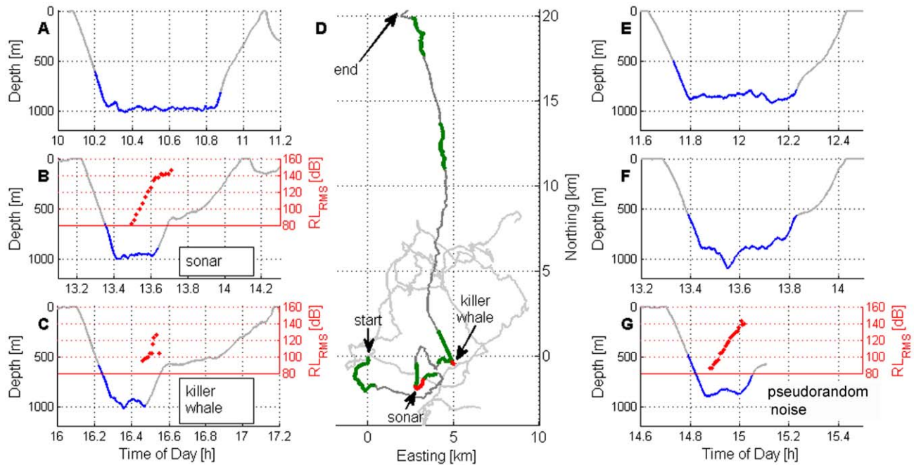
Figure 4. Whale acoustic activity and dive behavior before, during and after sound playback experiments. Deep foraging dives of one beaked whale tagged in 2007 (A–C) and another beaked whale tagged in 2008 (E–G) with the time of each dive indicated on the x-axis. The segment of the dive when the whale was clicking is indicated by coloring the dive profile blue. (A) This first dive after tagging was a pre-exposure dive. (B) This second dive after tagging involved playback of the MFA sonar stimulus, with slowly increasing level of playback. The red dots mark the received sound pressure level of the playback signal as recorded on the whale (in dB RMS re 1 \mu Pa averaged over a 200 msec window). (C) This third dive involved playback of killer whale (ORCA) sounds. The received level of the ORCA playback signal indicated by the red dots is the third octave band with the most energy averaged over a 200 msec. (D) The horizontal component of the motion of the tagged whale exposed to playbacks in 2007 is plotted in the dark gray and colored lines. Deep foraging dives are marked in green, and playback sound exposure is indicated in red. Tracks of three other beaked whales tagged during baseline conditions when no sonar was transmitting are shown in light gray for comparison. All tracks are presented with respect to the same arbitrary start position at (0, 0). Note that none of the baseline tracks contain segments as linear as the avoidance response of the whale after playback of killer whale sounds. (E–F) These first two dives after tagging in 2008 were pre-exposure dives. (G) The third dive after tagging in 2008 involved playback of the PRN sound stimulus, with slowly increasing level of playback. The red dots mark the increasing received sound pressure level of the playback signal (in dB RMS re 1 \mu Pa averaged over a 200 msec window). doi:10.1371/journal.pone.0017009.g004
