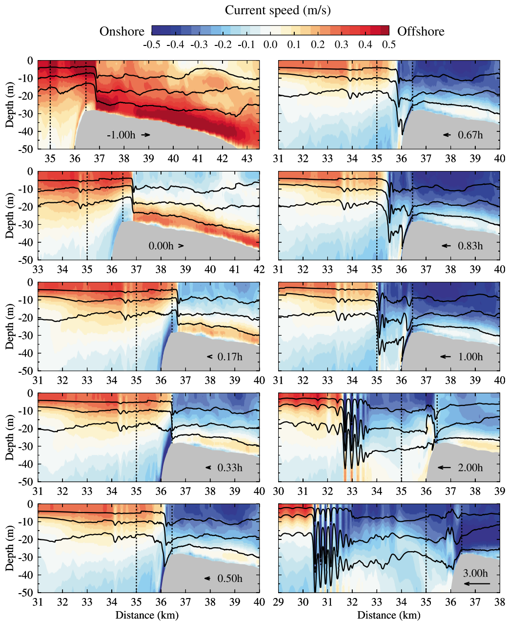
Figure 5. Snapshots of the cross-bank distribution of density contours \sigma_t = 22.5, 23.5, \text{ and } 24.5 and cross-bank currents at -1.00, 0, 0.17, 0.33, 0.50, 0.67, 0.83, 1.00, 2.00, \text{ and } 3.00 h relative to the ebb-flood transition for the standard stratification case driven by the spring tidal forcing. The negative sign indicates the ebb period. The ebb-flood transition is defined as the time of low tide at the open boundary. The area bounded by the two vertical dashed lines is the internal wave generation region during the flood tide.
