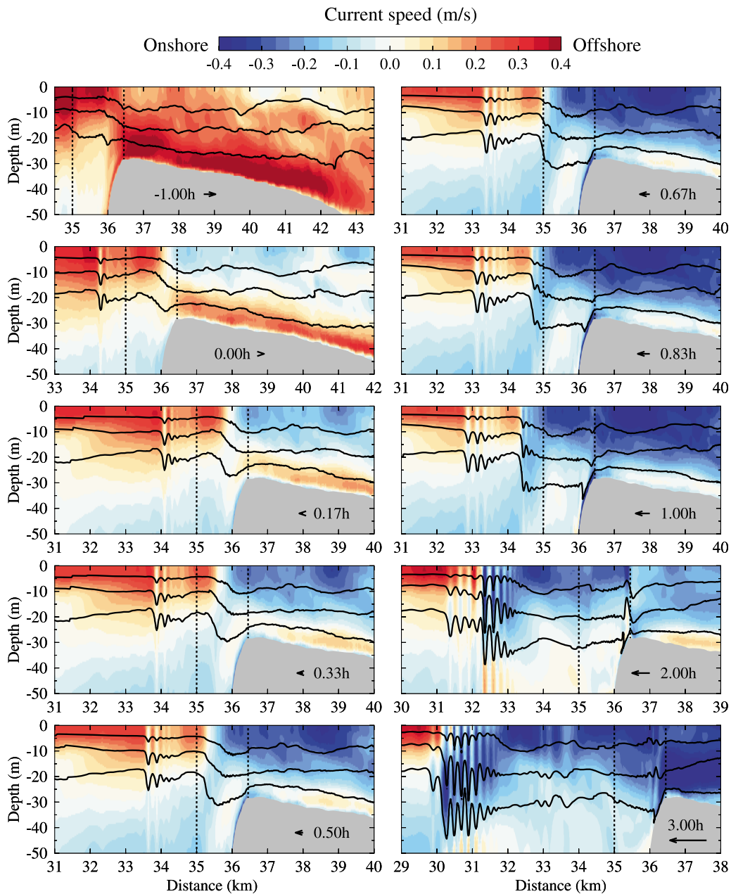
Figure 8. Snapshots of the cross-bank distribution of density contours \sigma_t = 22.5, 23.5, and 24.5 and cross-bank currents at select times relative to the ebb-flood transition for the standard stratification case driven by the mean tidal forcing. The selected hours and definition of ebb-flood transition are the same as those shown in Figure 5.
