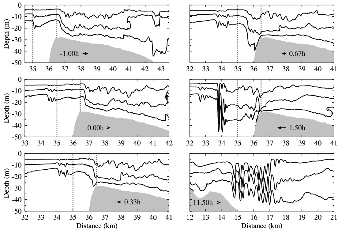
Figure 15. Snapshots of the cross-bank distribution of density contours \sigma_t = 22.5, 23.5, and 24.5 at the selected hours relative to the ebb-flood transition for the standard stratification and spring tidal case with no bottom friction. All time labels have the same definitions as those shown in Figure 5.
