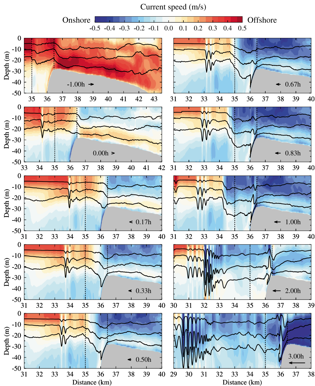
Figure 14. Snapshots of the cross-bank distribution of density contours \sigma_t = 22.5, 23.5, and 24.5 and cross-bank currents at the selected hours relative to the ebb-flood transition for the standard stratification and spring tidal case with inclusion of Earth's rotation. The selected hours and definition of ebb-flood transition are the same as those shown in Figure 5.
