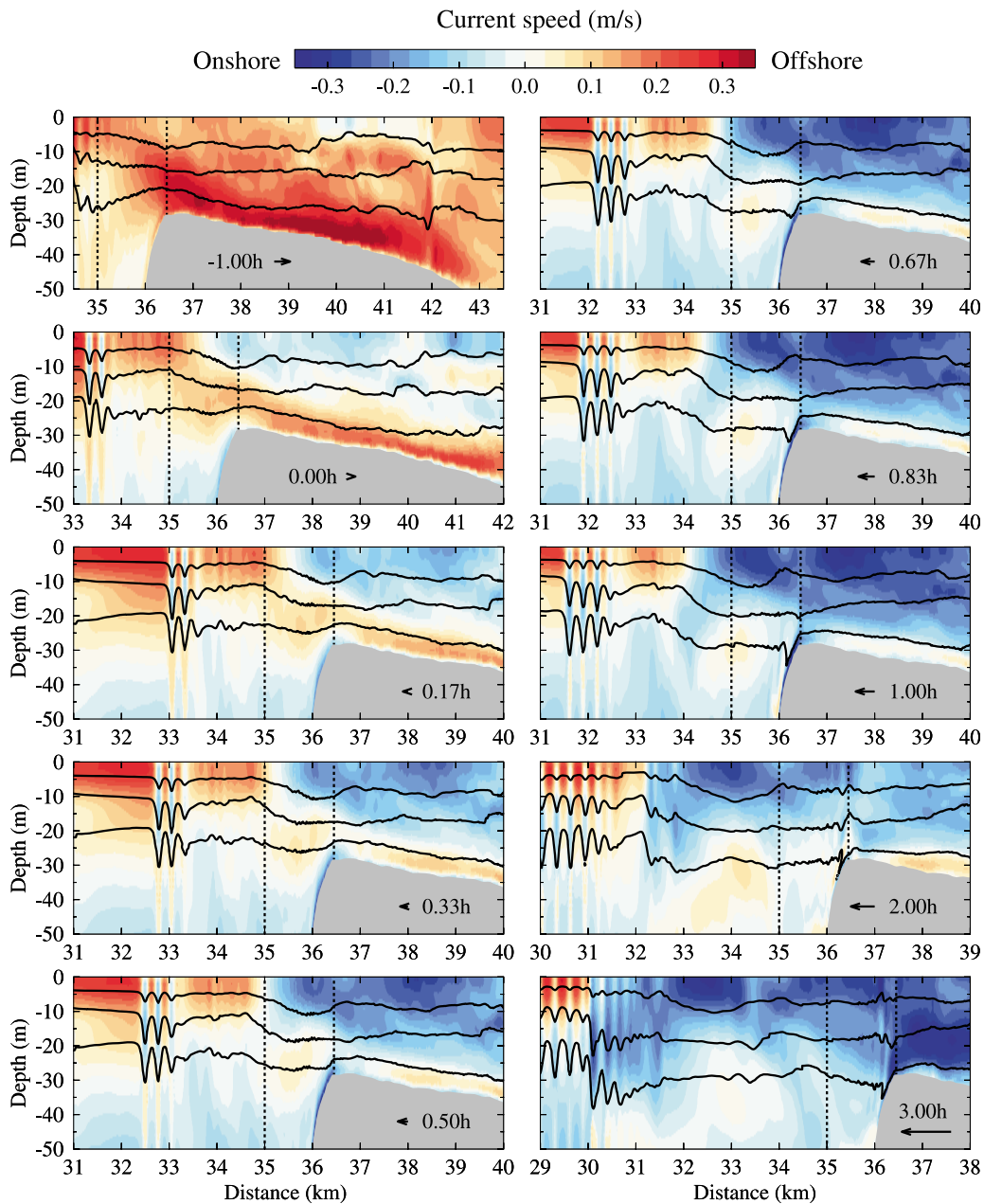
Figure 9. Snapshots of the cross-bank distribution of density contours \sigma_t = 22.5, 23.5, and 24.5 and cross-bank currents at select hours relative to the ebb-flood transition for the standard stratification case driven by the neap tidal forcing. The selected hours and definition of ebb-flood transition are the same as those shown in Figure 5.
