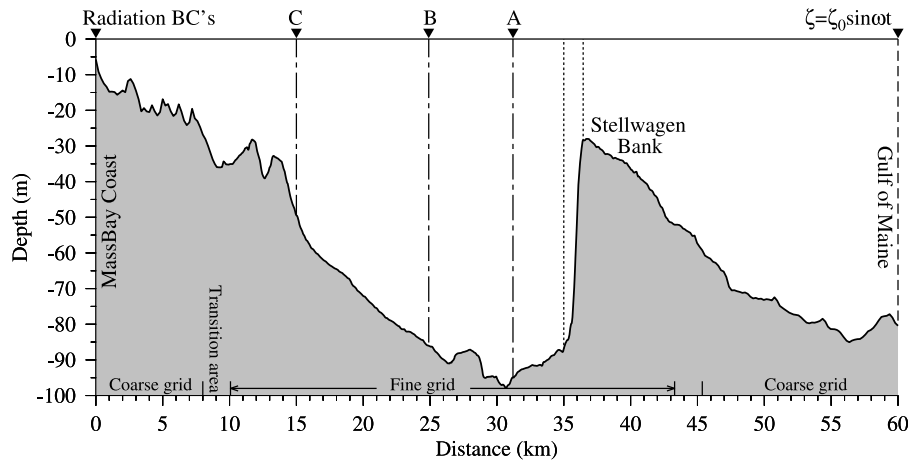
Figure 3. Bathymetry of FVCOM-NH model on the cross-bay transect shown in Figure 1. The model is driven by tidal forcing specified as \zeta = \zeta_o \sin \omega t at the open boundary. Here \zeta is the free surface elevation, and \zeta_o and \omega are the amplitude and frequency of the M_2 tide. The spring, mean, and neap tidal forcing are specified by adjusting \zeta_o . A gravity wave radiation boundary condition is specified on the shore side boundary under the assumption that zero energy reflects back into the interior from the coast. The computational domain features a nonuniform horizontal grid (see section 2 for details). A, B, and C are the locations of the MBIWE98 measurement sites (also shown in Figure 1).
