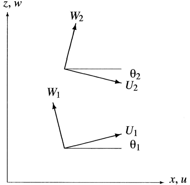
FIG. 1. Schematic illustrating the (2D) two-instrument geometry. The true coordinate system is given by x and z with velocities u and w , respectively. The two instruments measure velocities (U_1, W_1) and (U_2, W_2) oriented at small angles \theta_1 and \theta_2 , respectively, to the true coordinate system. The magnitudes of \theta_1 and \theta_2 are exaggerated for display purposes.
