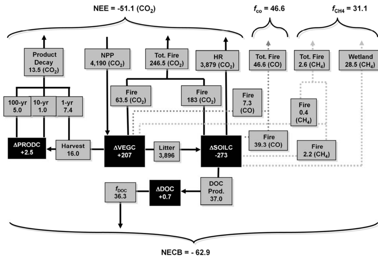
Figure 2. Simulated carbon stock changes and fluxes (Tg C yr -1 ) of the terrestrial component of the Arctic Basin, 1997 to 2006.
