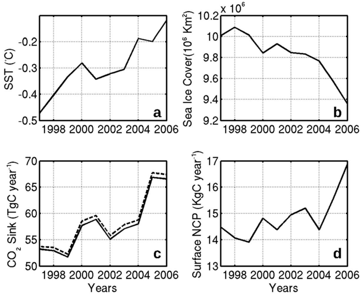
Figure 8. Annual mean (a) sea surface temperature, (b) sea-ice covered area, (c) \text{CO}_2 oceanic sink (solid line is for climatological DOC inputs and dashed line is for TEM DOC inputs), and (d) surface net community production (NCP) for the simulated period 1997-2006. Values are for the oceanic area north of 65^\circ \text{ N} .
