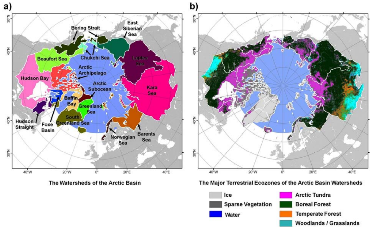
Figure 1. Maps showing a) the delineation of the terrestrial watersheds of the Arctic Basin and b) the spatial distribution of the major ecosystem types across these watersheds.
