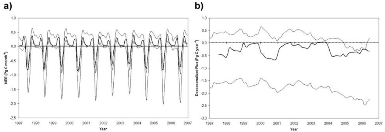
Figure 10. Comparison of a) monthly \text{CO}_2 flux ( \text{Pg C month}^{-1} ) and b) deseasonalized fluxes ( \text{Pg C yr}^{-1} ) based on the combined land and ocean NEE estimates from the model results of this study (thick lines) within the range of uncertainty in TransCom3 model estimates from the 104 station-data network (thin lines) aggregated for the Boreal North America, Boreal Asia, and Northern Ocean regions, over the 1997 – 2006 time period.
