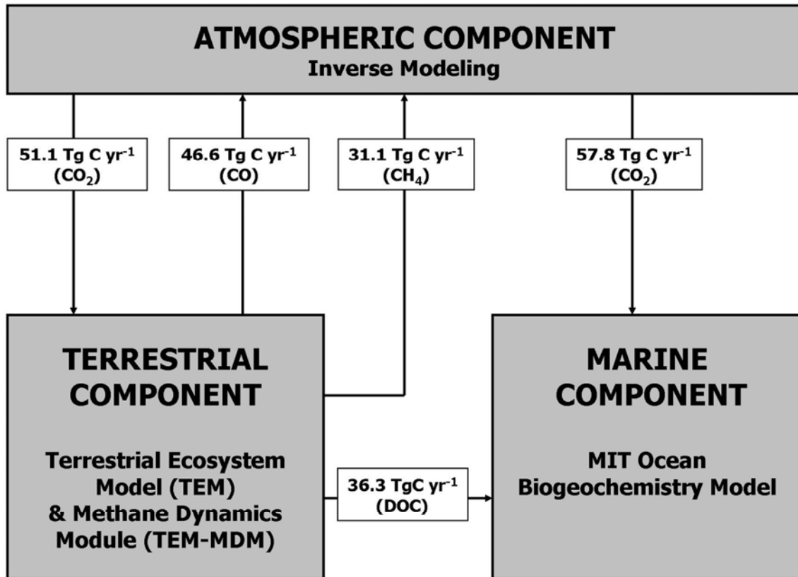
Figure 9. Overview of the results from this modeling study estimating the fluxes of C as CO 2 , CH 4 , of CO between the main components of the Arctic Basin system over the 1997 to 2006 time period.
