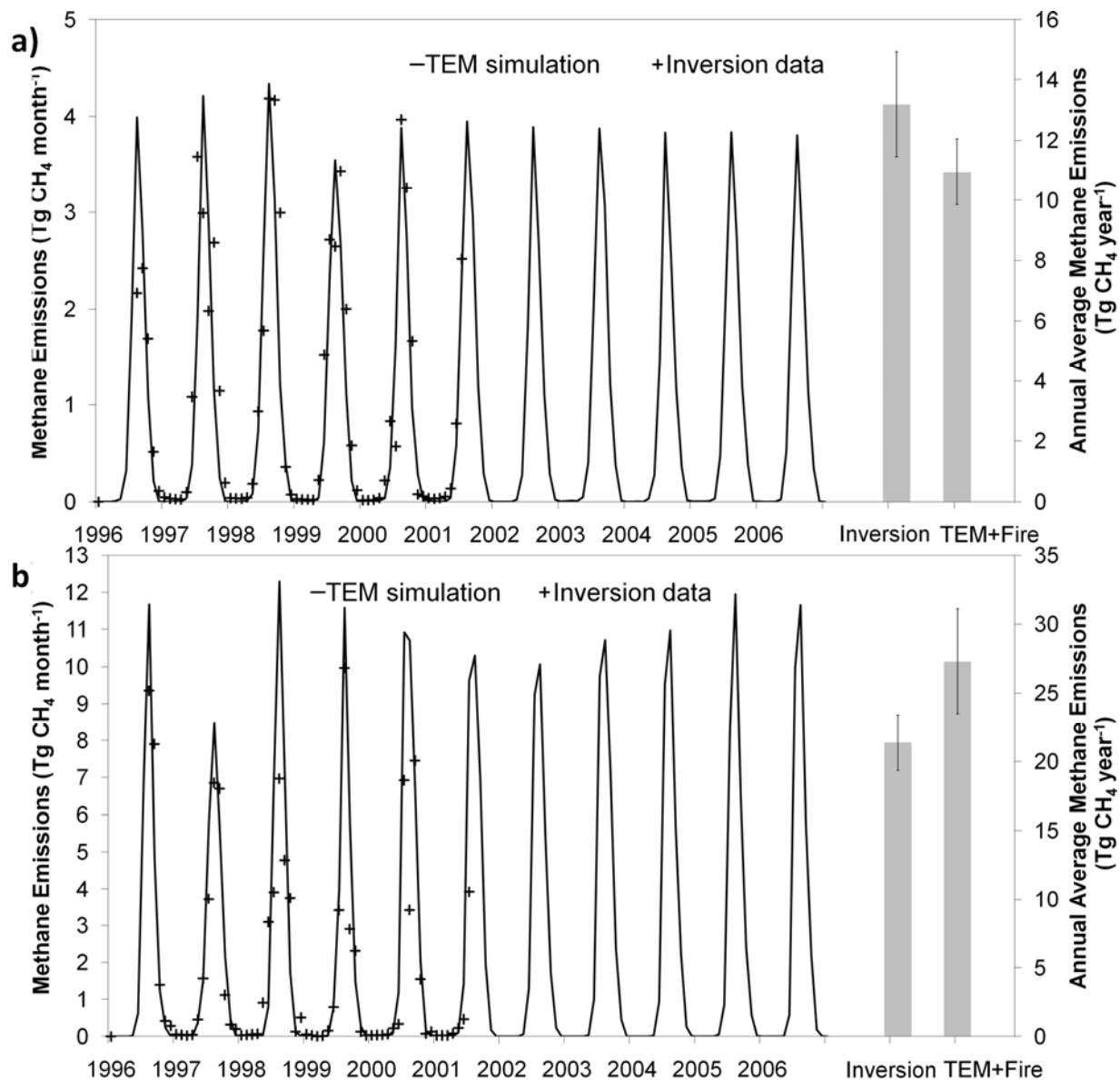
Figure 6. Comparison \text{CH}_4 exchange estimates between TEM and MATCH simulations in (a) Boreal North America and (b) Boreal Asia: Black solid lines show the seasonal dynamics of biogenic and pyrogenic \text{CH}_4 emissions estimates of TEM from 1996 to 2006 ( \text{Tg CH}_4 \text{ month}^{-1} ). Black crosses show the seasonal changes of net \text{CH}_4 emissions from biogenic and pyrogenic sources from 1996 to 2001 estimated by MATCH ( \text{Tg CH}_4 \text{ month}^{-1} ). Bars show the annual mean for MATCH simulations (1996-2001) and MDM-TEM simulations (1996-2006) as \text{Tg CH}_4 \text{ year}^{-1} . Error bars indicate standard deviation (interannual variability) for the time period of the inversion simulations (1996 – 2001).
