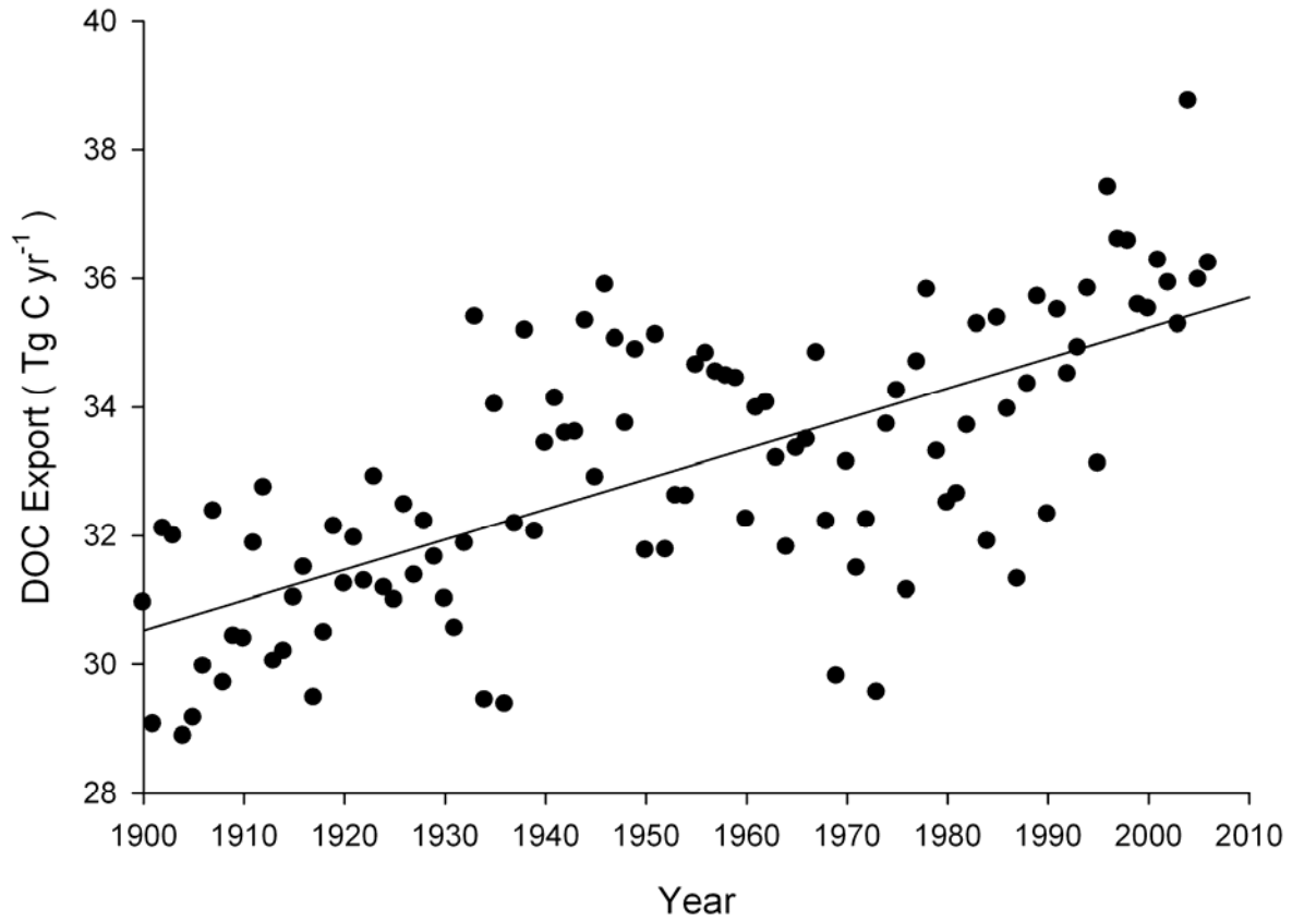
Figure 12. TEM estimates of DOC export to the Arctic Ocean from surrounding watersheds between 1900 and 2006.
