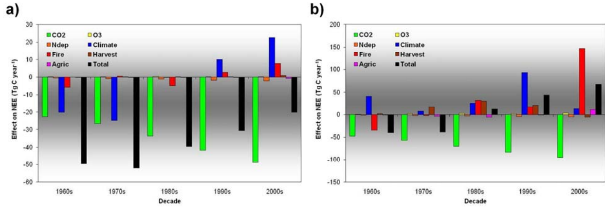
Figure 11. Total and individual average annual effects (Tg C yr -1 ) of temporal variability in atmospheric [CO 2 ], tropospheric O 3 levels, N deposition rates, climate, fire, forest harvest and agricultural establishment and abandonment on NEE for each decade since the 1960s across the Boreal Land Regions in a) arctic tundra and b) boreal forest ecosystems.
