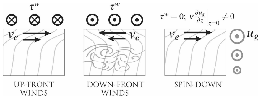
FIG. 1. Schematic illustrating frictional re-de-stratification at a baroclinic current in the upper ocean. (left) Up-front winds blowing against a baroclinic geostrophic flow u_g will drive an Ekman flow v_e that flattens isopycnals (gray) and hence restratifies the fluid via differential horizontal advection of buoyancy. (middle) When the wind is oriented down front, Ekman advection of buoyancy destabilizes the water column, driving convective mixing and a reduction of the stratification. (right) With no wind forcing, the frictional spindown of a baroclinic current arising from the mismatch of the geostrophic shear and the zero stress boundary condition induces a restratifying Ekman flow.
