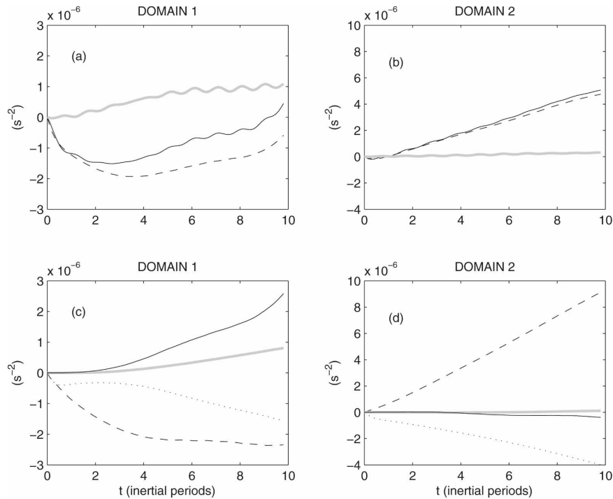
FIG. 6. Temporal change in the mean PV and stratification; and the processes that give rise to this change as diagnosed from run 4. (a), (b) The change in mean stratification, \Delta\bar{N}^2 (thin black) and PV, \Delta\bar{q}/f (dashed) are plotted along with the frontogenetic contribution to re-stratification, FRONT_i (thick gray), for domains 1 and 2, respectively. (c), (d) The change in PV due to vertical friction, FRIC_v (dashed), lateral friction, FRIC_l (thick gray), diabatic processes, DIA_i (dotted), and advection, ADV_i (thin black), are plotted for domains 1 and 2, respectively.
