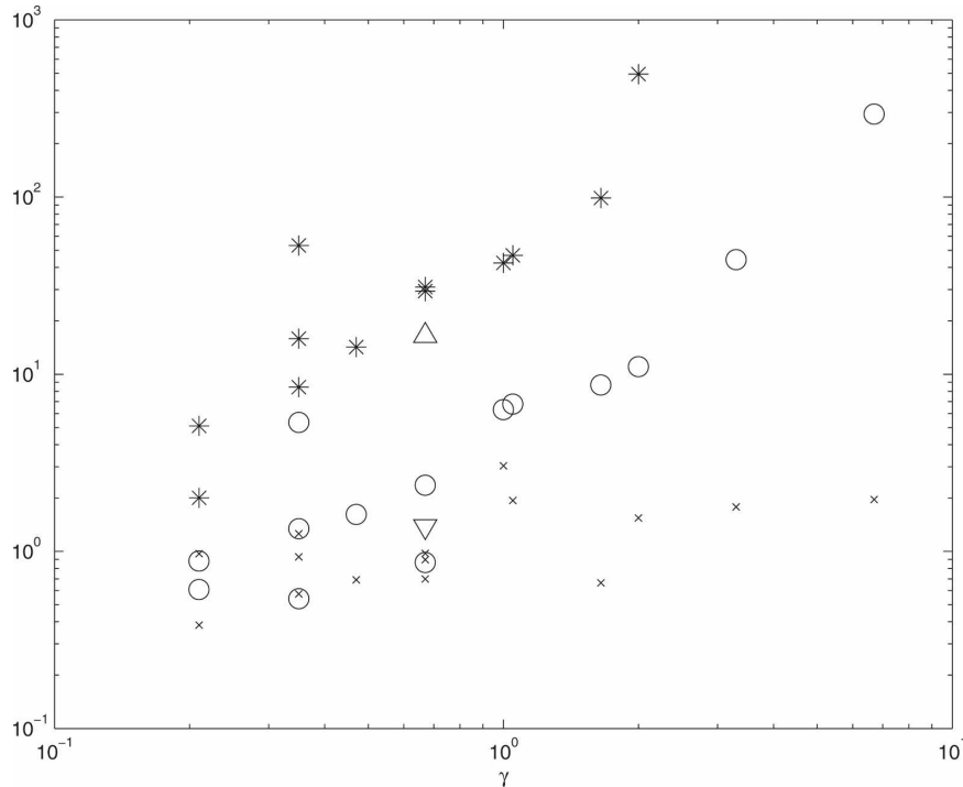
FIG. 9. The absolute value (y axis) of the ratio of term \text{FRIC}_v to \text{FRONT}_i averaged over the last two inertial periods of the experiment vs \gamma_{\text{wind}} = u_w^2 / \text{Ro} \Delta u_g for all of the runs forced by both winds and confluence. Asterisks and circles correspond to values taken from domains 2 and 1, respectively. Results from run 20, where the resolution was doubled, are given by the upward (domain 2) and downward (domain 1) triangles. The ratio of |\text{FRIC}_v| in domain 1 (averaged over the last two inertial periods) to the scaling for the upper bound on the restratification by frontogenesis \Delta \bar{N}_{\text{front}}^2 is denoted by the xs.
