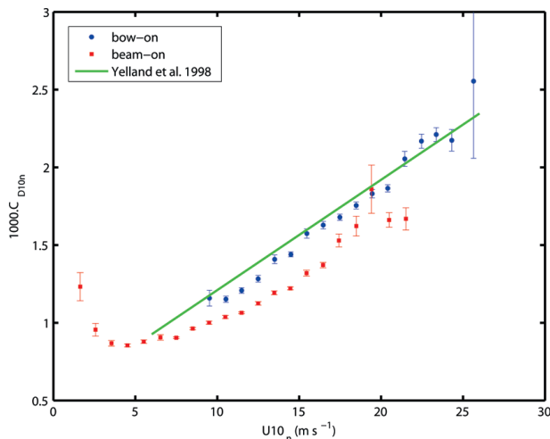
FIG. 9. Neutral drag coefficients determined from bow-on (blue) and beam-on (red) wind measurements on the Polarfront averaged in 1 \text{ m s}^{-1} wind speed bins; error bars indicate the standard error about the means. The relationship from Yelland et al. (1998) is shown for comparison. The beam-on results are very obviously biased low.
