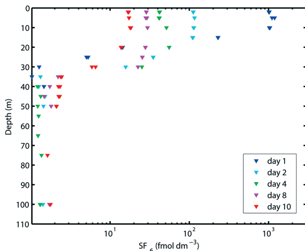
FIG. 3. Changes in SF_6 concentration in depth profiles from patch 2 in the days following the tracer release. Concentrations decrease rapidly as the patch spreads both horizontally and vertically and, to a lesser extent, as the gas diffuses across the air–sea interface. Note that background concentrations below the mixing layer are typically 1.5 fmol (i.e. 10^{-15} moles) per liter of seawater.
