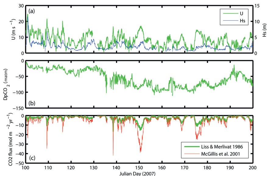
FIG. 10. A 100-day time series of HiWASE measurements on the Polarfront : (a) mean wind speed U and significant wave height H_s ; (b) air–sea difference in \text{pCO}_2 ; (c) bulk estimates of the \text{CO}_2 flux from parameterizations that span the range of published values for transfer velocity (Liss and Merlivat 1986; McGillis et al. 2001). The mean fluxes over the 100 days are -2.77 (Liss and Merlivat 1986) and -5.05 \mu\text{mol m}^{-2} \text{ yr}^{-1} (McGillis et al. 2001).
