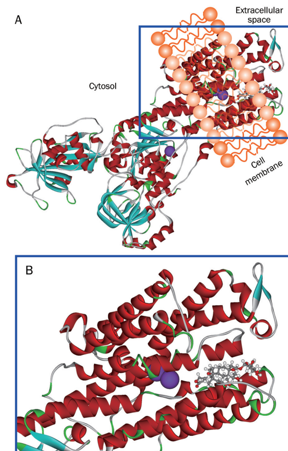
Figure 1. (A) Crystal structure of ouabain binding to the extracellular pocket of shark rectal gland Na + /K + -ATPase (PDB code 3A3Y) α subunit [17] . Amino acid residues of Na + /K + -ATPase α subunit are shown in ribbon structure, and ouabain in scaled ball and stick. K + binding sites are shown in purple balls. (B) Enlarged diagram without the membrane bilayer shown in the blue box of (A).
