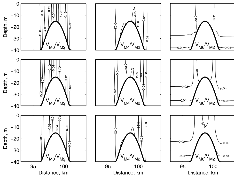
Figure 6. Effect of bottom roughness. Cross-section plots of the speed ratio of mean flow ( V_{M_0} ) and each overtide ( V_{M_4} , V_{M_6} ) to the semidiurnal tidal component speed ( V_{M_2} ), along transect BB' , corresponding to (top) case 1, (middle) case 2, and (bottom) case 3.
