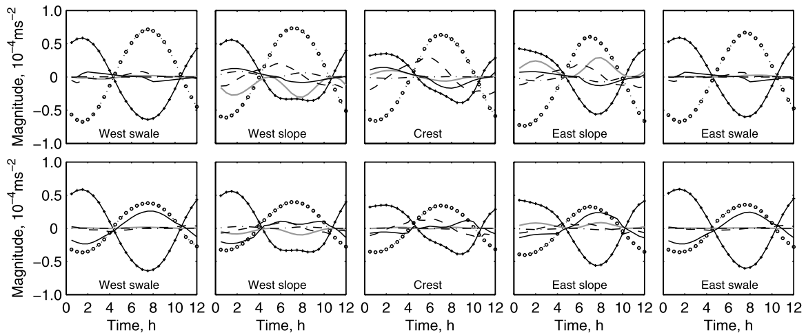
Figure 11. Significant terms of the cross-shelf momentum balance equation at five different locations along the transect AA' and at two vertical levels: (top) surface and (bottom) near the bottom. The lines legend is as in Figure 10.
