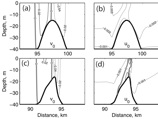
Figure 9. Cross-section plots of the along- and across-isobath residual flow ( v_o' and u_o' ) for banks rotated 5^\circ with (top) symmetric and (bottom) asymmetric bathymetric profiles, along transect BB' . Black contours represent positive values, while gray contours represent negative values. The thick gray contour represents the zero isotach.
