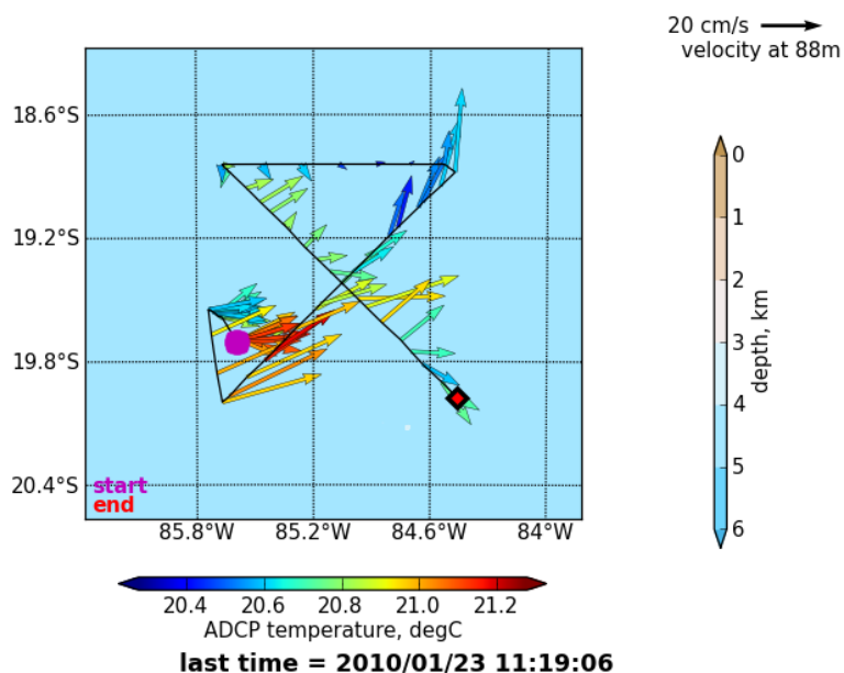
Figure 5-8. Detail of the cruise track for the two VMP Surveys. Purple dot denotes the location for the 1 st survey around the STRATUS 10 mooring and beginning of the 2 nd survey. Red diamond denotes the end of the 2 nd survey of the eddy. Arrows are current vectors near surface from ships's ADCP, colored according to water temperature.
