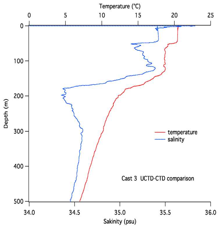
Figure 5-17. CTD casts made during Stratus 10 cruise, in chronological order from top to bottom.
