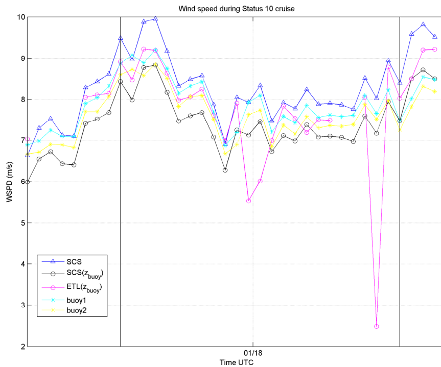
Figure 3-9. Wind speed. Z_{buoy} refers to adjustment to height of sensor on buoy.
