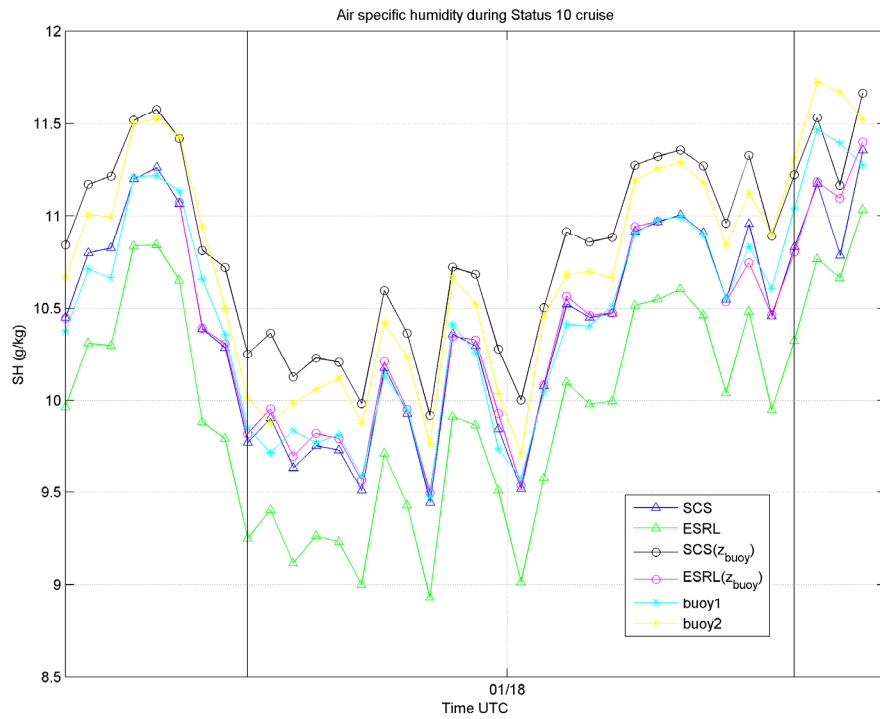
Figure 3-12. Air specific humidity. Z_{\text{buoy}} refers to adjustment to height of sensor on buoy.
