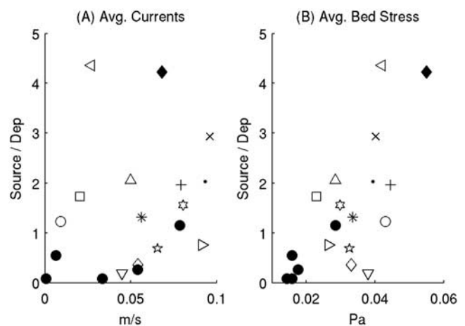
Figure 12. Source/sink ratio of fluvial source to deposit size (y axis) compared to (a) time-averaged currents and (b) time-averaged bed shear stress. The y axis is the fluvial source divided by the amount of deposition within 10 km of each river mouth. Currents and bed shear stress were time averaged at grid cells within 10 km of each river mouth. Symbols used for each river provided in Table 1.
