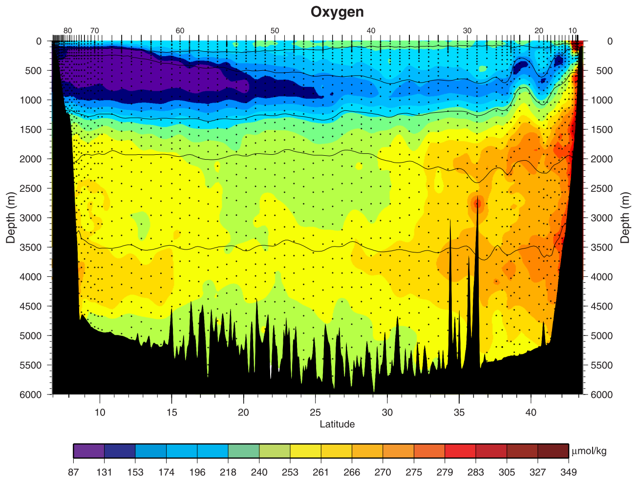
Figure 3d. Dissolved oxygen ( \mu\text{mol kg}^{-1} ). Dots show where bottle samples were collected. Contours indicate 6 subsets of neutral density layers.
