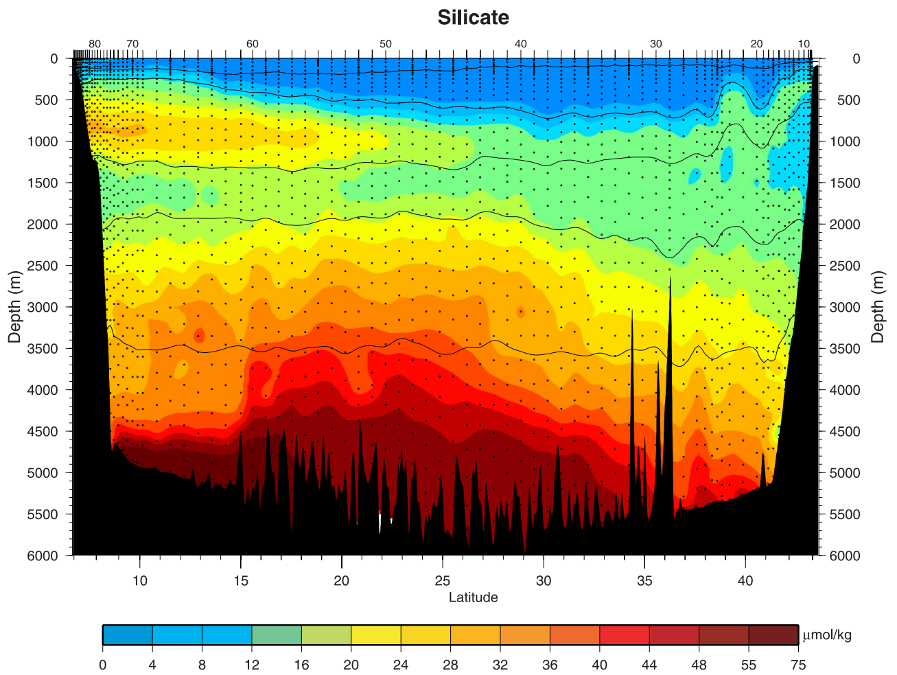
Figure 3g. Silicate ( \mu\text{mol kg}^{-1} ). Dots and contours as in Figure 3d.
