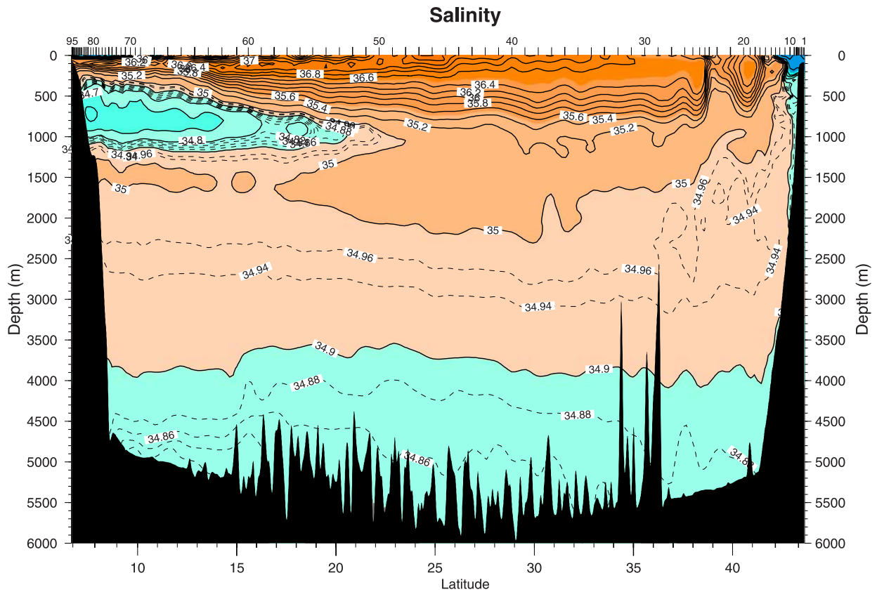
Figure 3b. Salinity.
