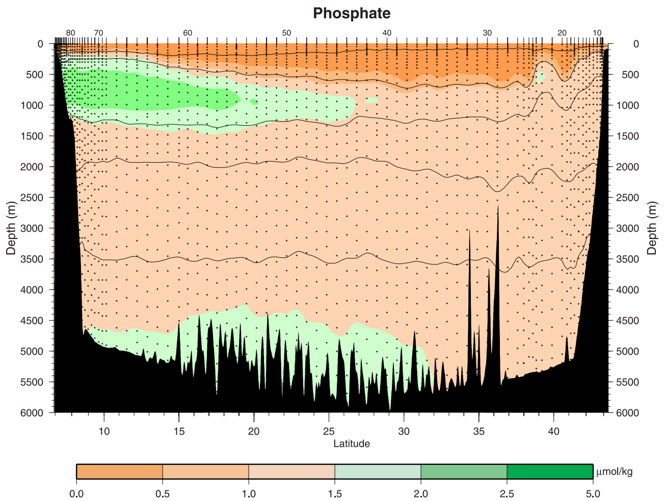
Figure 3f. Phosphate ( \mu\text{mol kg}^{-1} ). Dots and contours as in Figure 3d.
