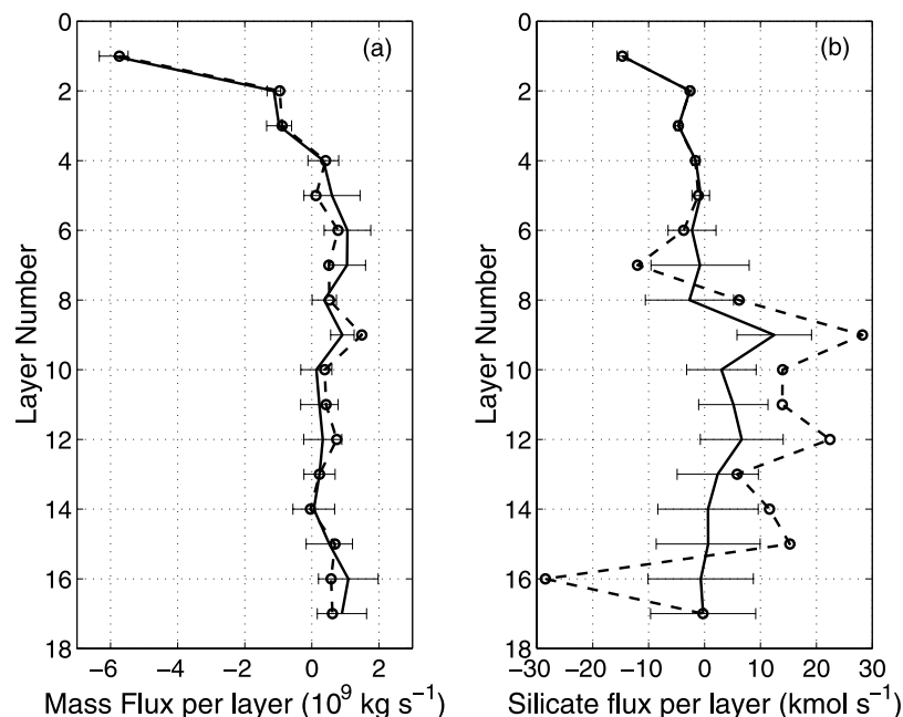
Figure 11. Total (a) mass and (b) silicate fluxes across 52°W section for 17 neutral density layers; dashed profiles are for solution conserving mass only; solid profiles are for solution conserving both mass and silicate. Errors bars are shown for the latter, for errors due to inversion only.
