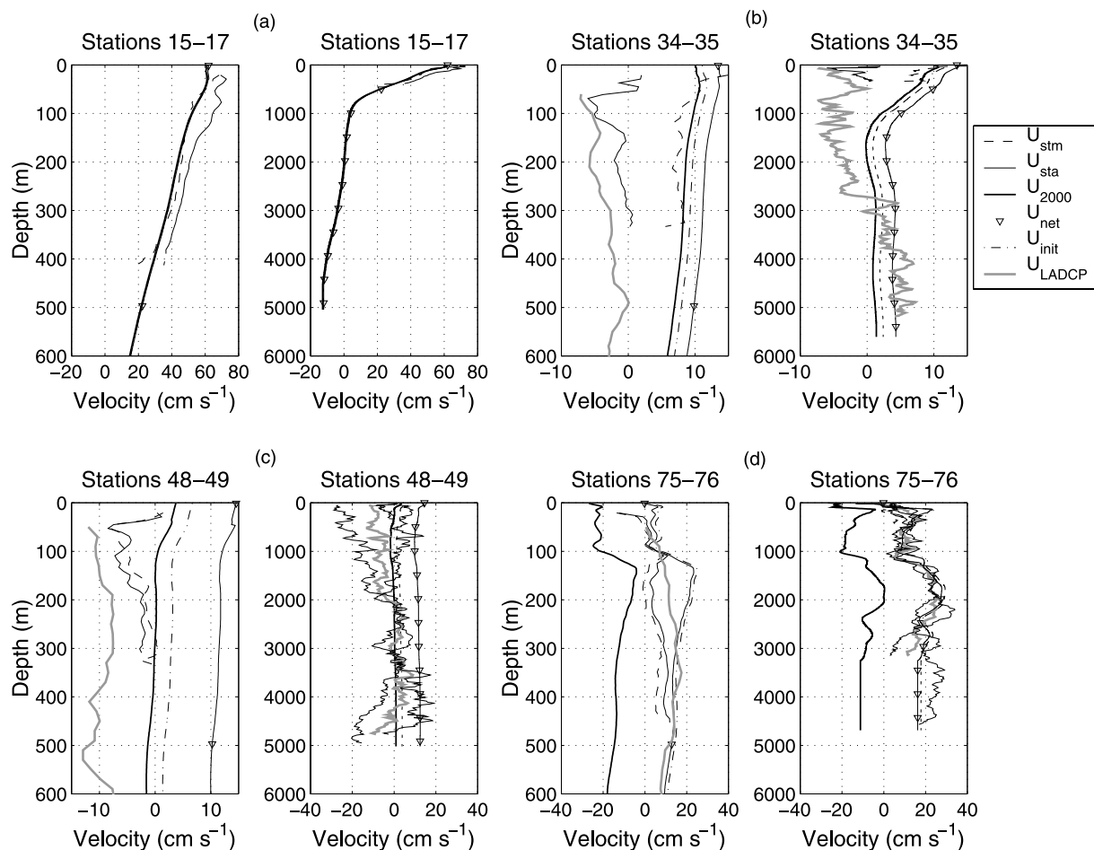
Figure 5. Comparison of different velocity estimates, as a function of depth, for four different station pairs. In each pair of panels the full depth profiles are shown to the right and an expanded view of the top 600 m is shown to the left. Three geostrophic profiles are shown: relative to 2000 dbar ( U_{2000} , heavy solid line), referenced to ADCP velocities ( U_{init} , light dash-dotted line), and including final adjustment ( U_{net} , inverted triangles). Two profiles are shown for shipboard ADCP, using first method ( U_{sta} , light solid line) or second method ( U_{stm} , light dashed line); see text. Where applicable, the gray solid profile is the LADCP velocity ( U_{LADCP} ) averaged between the two stations in the pair (uncorrected; see text). The right panels of Figures 5c and 5d also show the individual LADCP profiles comprising the station pair mean.
