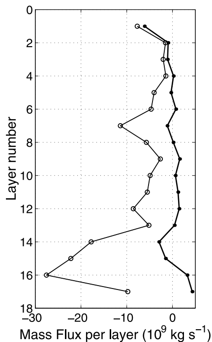
Figure 7. Total mass flux across 52°W section, for each of 17 neutral density layers, for geostrophic velocity referenced to ADCP data (open circles); for geostrophic velocity referenced to ADCP data, and then adjusted by a constant velocity to balance overall mass (solid dots).
