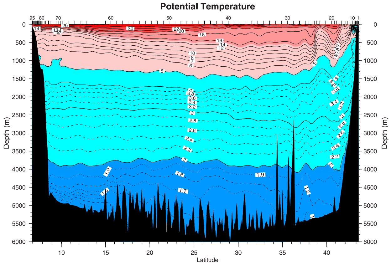
Figure 3a. Potential temperature (°C).
