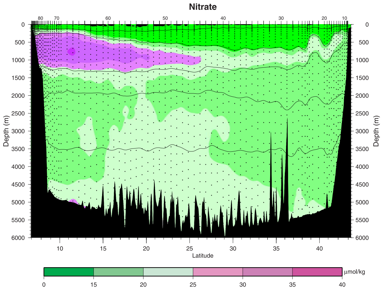
Figure 3e. Nitrate ( \mu\text{mol kg}^{-1} ). Dots and contours as in Figure 3d.
