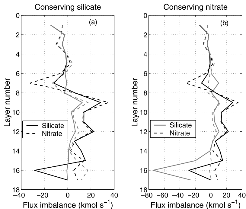
Figure 9. Total nutrient flux across 52°W section in each of 17 neutral density layers; solid (dashed) is silicate (nitrate). Black profiles are from inverse solution conserving only mass; gray profiles conserve both mass and either (a) silicate or (b) nitrate. Note different x axis scales.
