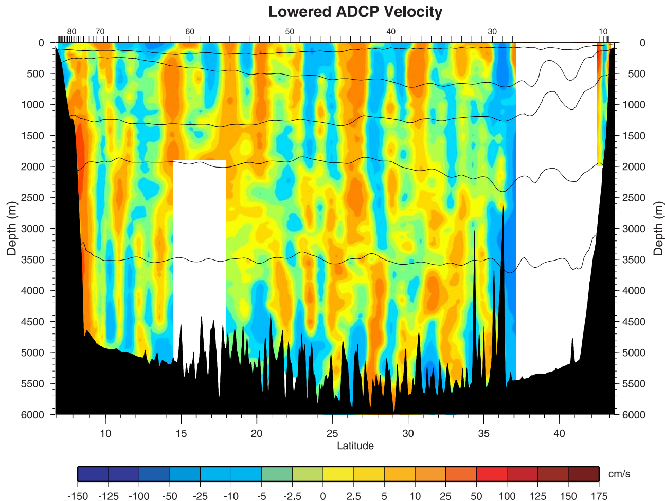
Figure 2. LADCP velocities perpendicular to A20 track line; positive velocities have eastward component. Blank areas are those where no LADCP data are available.
