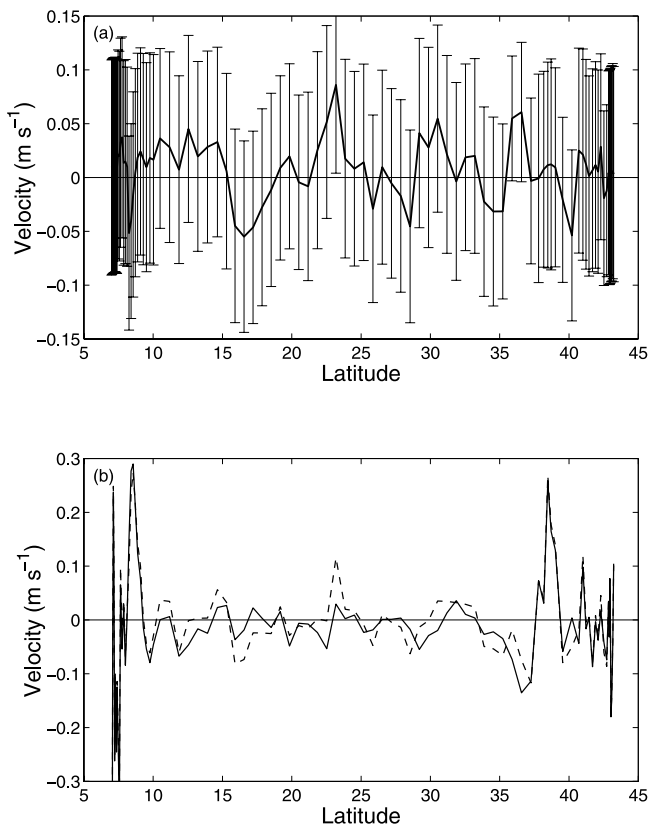
Figure 10. (a) Solution vector for final inverse, with error bars. (b) Initial reference velocity added to 2000-dbar referenced geostrophic velocity field (solid) and net reference velocity added to geostrophic velocity (dashed). The dashed line is the sum of the solid line and the velocity values shown in Figure 10a.
