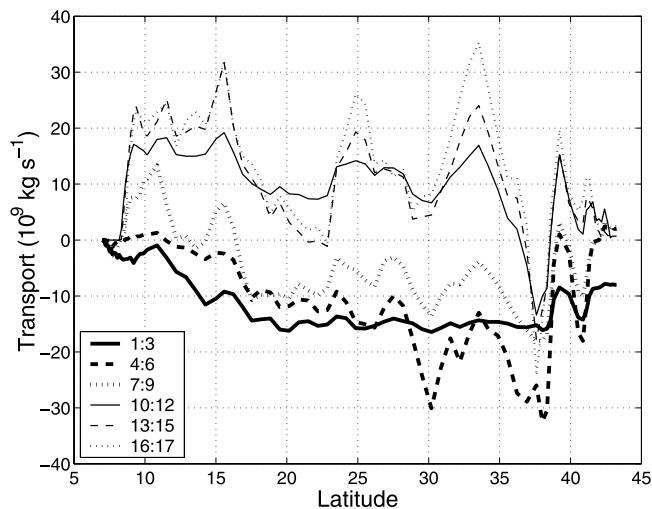
Figure 14. Meridional mass transport stream functions for 6 groups of neutral density layers indicated by the bold contours in Figure 3c. Transport in each layer is integrated northward from the southernmost station.
