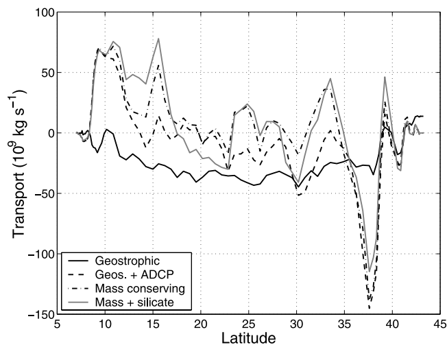
Figure 13. Total mass transport stream functions along 52°W for four different velocity fields discussed in the text. Top to bottom transport is integrated northward from the southernmost station.
