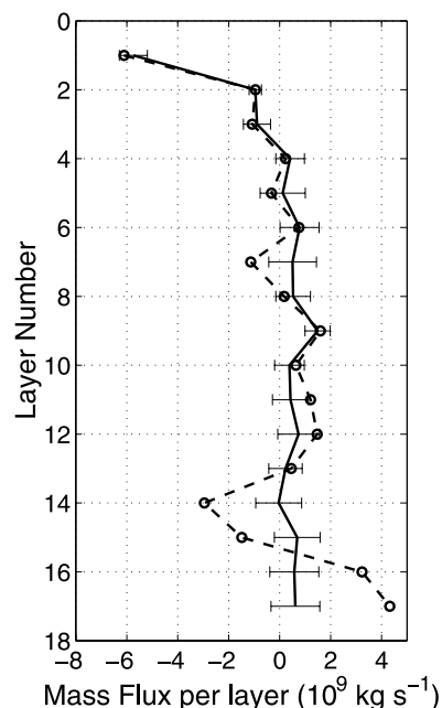
Figure 8. As in Figure 7. Dashed line is the same solution as solid dots shown in Figure 7; solid line is for solution resulting from inverse that imposes mass conservation in individual layers. Errors due to inversion are shown for the latter solution.
