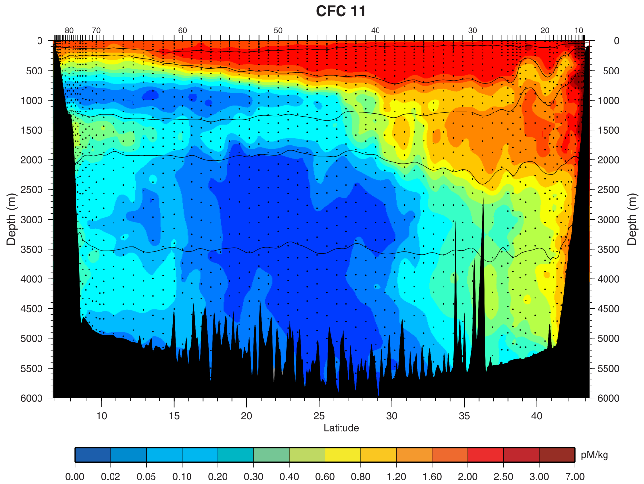
Figure 3h. CFC-11 ( \text{pmol kg}^{-1} ). Dots and contours as in Figure 3d.
