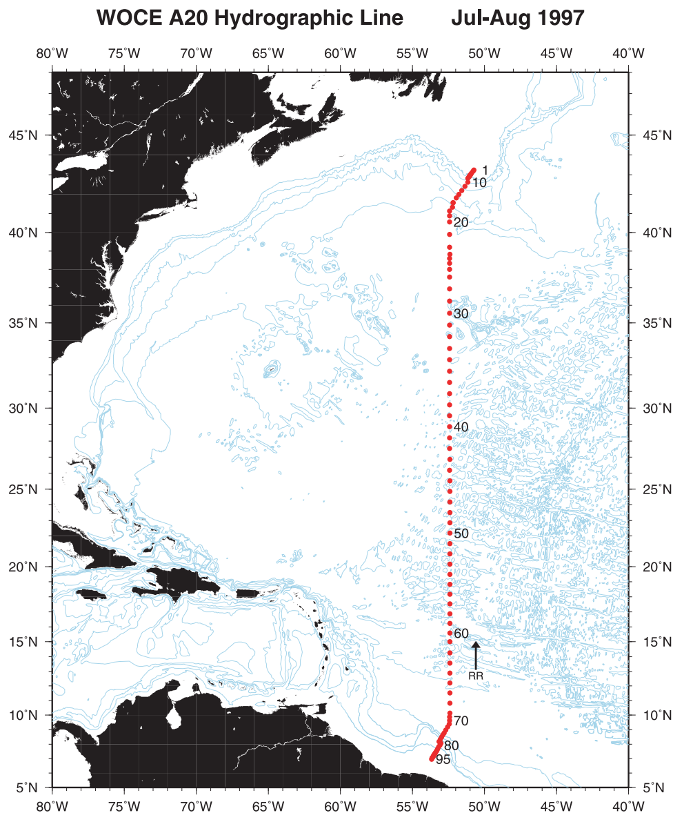
Figure 1. Cruise track for WOCE section A20, superposed on topography: topographic contours are every 1000 m. Red dots are station positions, with some stations numbers indicated. “RR” indicates the location of Researcher Ridge (shallower than 3000 m).
