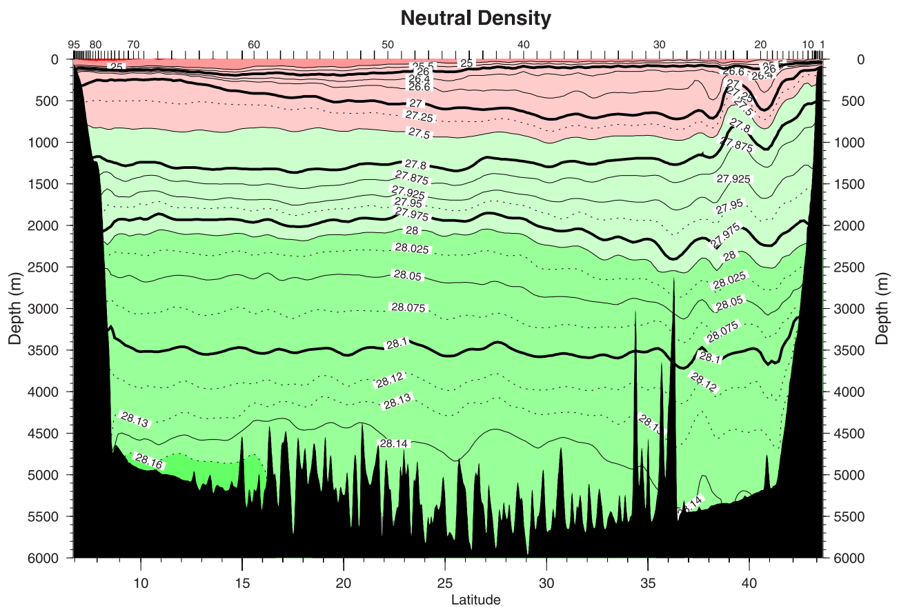
Figure 3c. Neutral density. Solid contours indicate the 17 density layers used in the inverse calculation; bold contours indicate six subsets of the layers referred to in the paper; dashed contours show additional detail.
