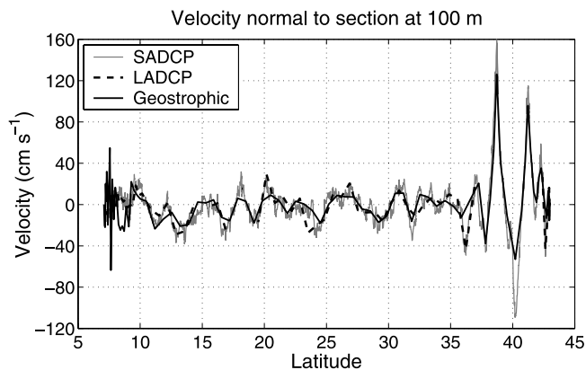
Figure 4. Comparison of velocity normal to cruise track at a depth of 100 m: shipboard ADCP (gray line); lowered ADCP (dashed black line); and geostrophic relative to 2000 dbar (solid black line).
