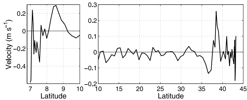
Figure 6. Initial velocity adjustment made to 2000 dbar-referenced geostrophic velocity, as determined by comparison to ADCP. The southern end of the section is expanded and has a different scale for the vertical axis because some reference velocities there are much larger.
