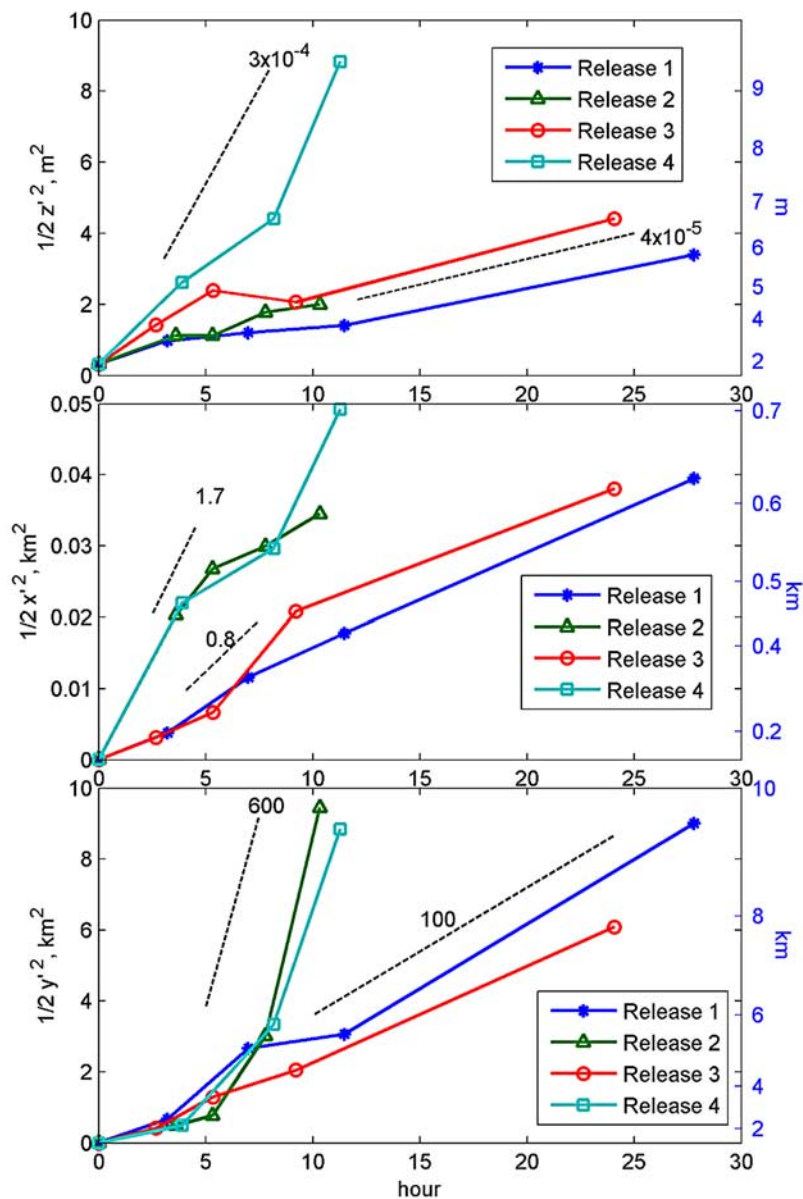
Figure 8. Time evolution of the 2nd moment of the dye distribution in the vertical (top), cross-estuary (middle), and along-estuary (bottom). Dashed lines indicate values of dispersion rate ( \text{m}^2/\text{s} ) for different slopes. The right-hand axis indicates the equivalent length scale of the patch ( \sim 4 x' ).
