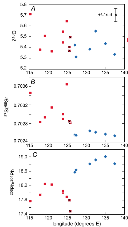
Figure 1. (a) Oxygen isotope composition versus longitude, (b) 87 Sr/ 86 Sr versus longitude, and (c) 206 Pb/ 204 Pb versus longitude of AAD samples used in this study, illustrating the distinctions in Sr and Pb isotopic composition between Indian- and Pacific-type MORB at the AAD. Indian-type samples are shown with red squares (zone B4 samples are shown with red squares with black crosses), and Pacific-type samples are shown with blue diamonds; sample classification is based on Pyle et al. [1992, 1995]. Average reproducibility of replicate measurements of the same samples (1 s.d.) is shown in Figure 1a. Average values of \delta^{18}O ( \pm 2 times the standard error of the mean) of the Indian- and Pacific-type samples are shown by large symbols to the right of the diagram in Figure 1a. See section 4.1 for discussion.
