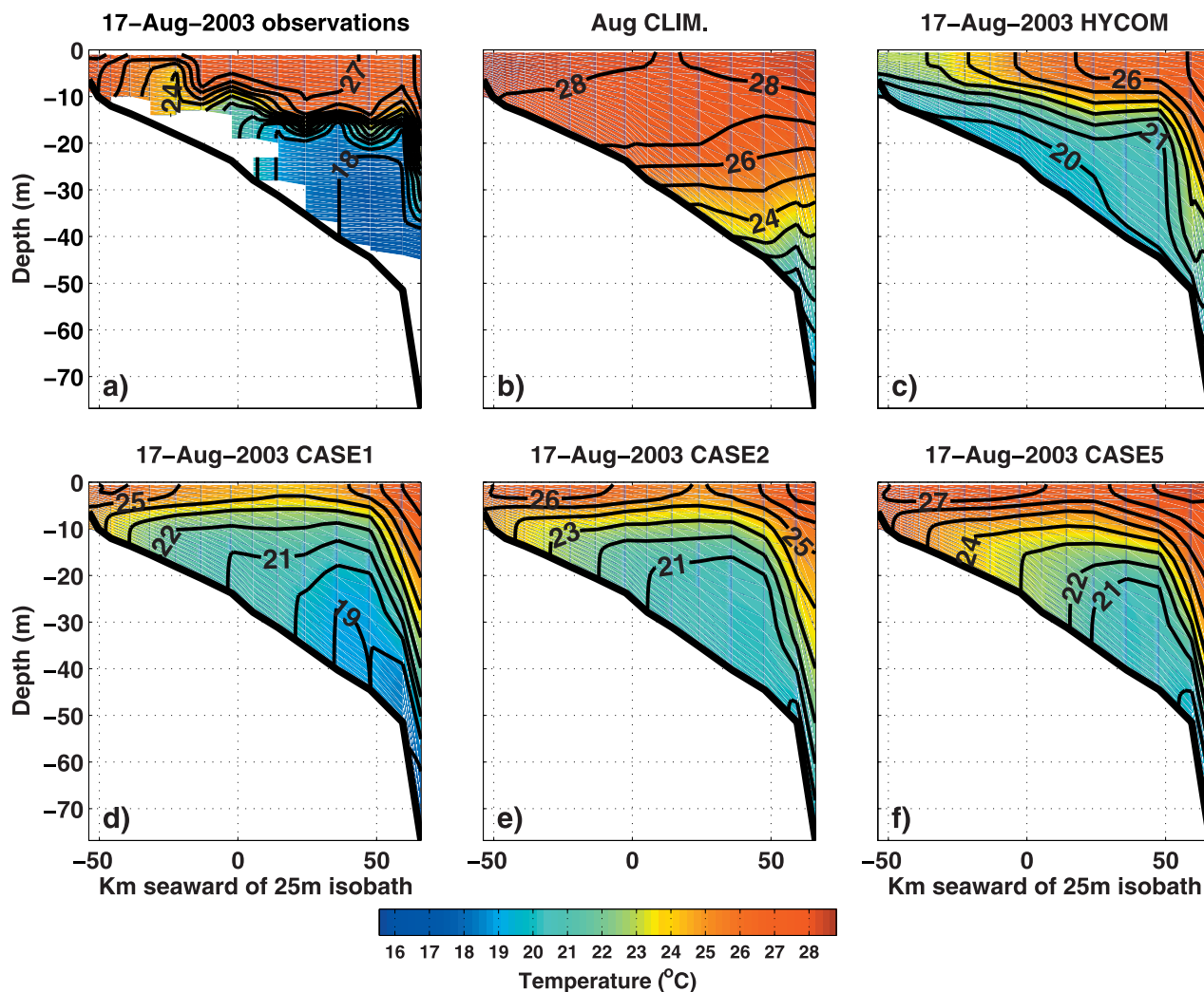
Figure 6. Observed and model temperature transect for 17 August 2003. (a) Observed temperature, (b) climatological, (c) HYCOM, (d) case 1, (e) case 2, and (f) case 5. The contour intervals are 1^{\circ}\text{C} .
