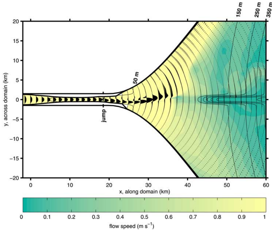
Figure 11. Snapshot of the flow in the lower (Black Sea) basin when it is set to -50 m so that the hydraulic jump occurs within the Bosporus. The arrows represent the depth-integrated flux. The water's edge is marked by a heavy black line. On leaving the Bosporus Strait the jet attaches to the coast and flows along it. Such a jet may have been responsible for scouring the northwestern channel at the Bosporus mouth (cf. Figure 3).
