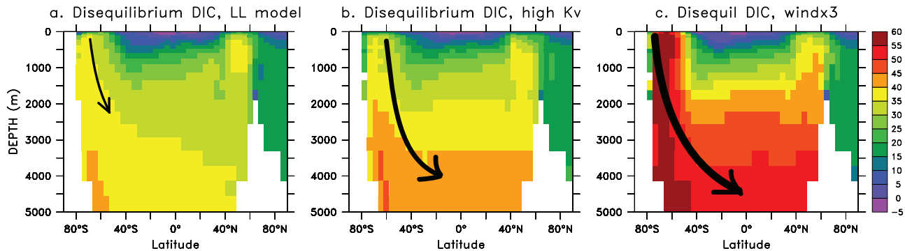
Figure 8. Global zonal averages of disequilibrium DIC in the (a) LL, (b) high K_v , and (c) windx3 GCMs. Results shown for the regular gas exchange (RGE) models. Disequilibrium DIC ( \mu\text{mol}/\text{kg} ) at each point calculated as the difference between total DIC , surface equilibrium DIC , and DIC_{soft} = r_{C:P} \cdot (PO_4 - PO_{4,pre}) . Increasing ventilation via the Southern Ocean results in more accumulation of deep disequilibrium DIC .
