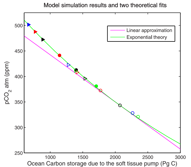
Figure 6. Variation of atmospheric p\text{CO}_2 (ppm) with the soft-tissue ocean carbon storage (PgC), OCS_{soft} = V_{oc} \cdot r_{C:P} \cdot ([\text{PO}_4] - [\text{PO}_{4\text{pref}}]) . The exponential fit given by equation (8) and the linear fit given by equation (9) are shown on top of model results from eight different models. Fast gas exchange simulations shown for all models. Biological timescale \tau is either 30 days (open symbols) or 1 year (full symbols). Model notation as in Figure 3.
