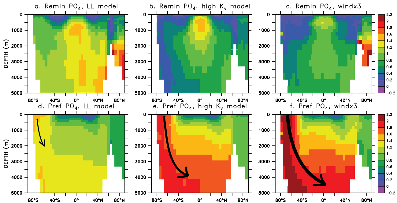
Figure 4. Global zonal averages of remineralized \text{PO}_4 (top) and preformed \text{PO}_4 (bottom) in the LL, high K_v , and windx3 GCM simulations. Units are \mu\text{mol}/\text{kg} . Larger vertical mixing K_v , or larger Southern Ocean winds result in stronger Southern Ocean overturning circulation (see arrows) and larger deep preformed \text{PO}_4 .
