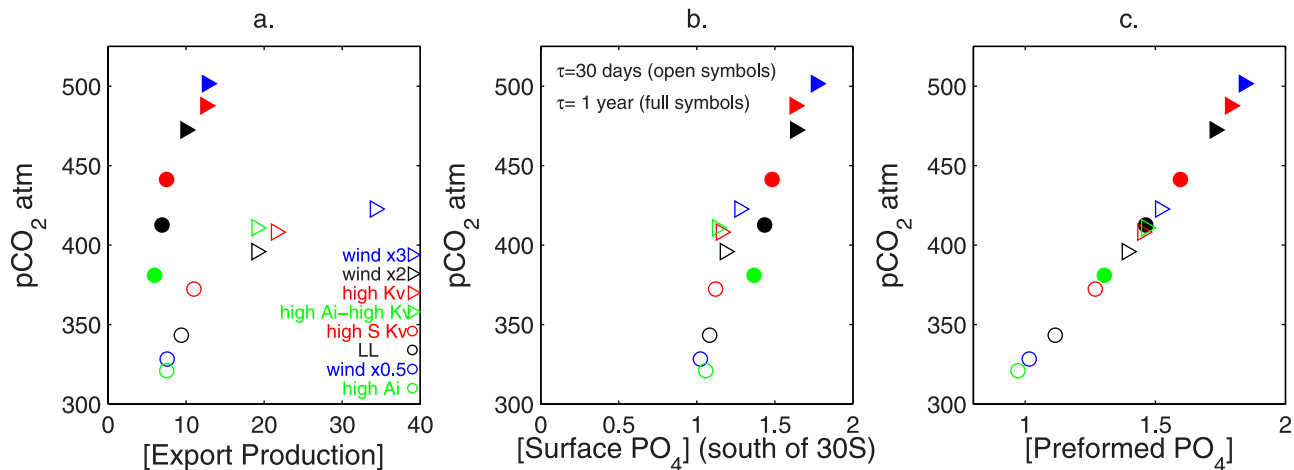
Figure 3. Atmospheric p\text{CO}_2 (ppm) versus (a) total globally averaged export Production ( \text{PgC/a} ), (b) average surface \text{PO}_4 south of 30^\circ\text{S} ( \mu\text{mol/kg} ), and (c) global volume averaged preformed \text{PO}_4 ( \mu\text{mol/kg} ). Fast gas exchange simulations. Models have biological timescale \tau = 30 days (open symbols) or \tau = 1 year (full symbols). Shown are the LL (black circle), high A_i (green circle), windx0.5 (blue circle), high south K_v (red circle), high K_v -high A_i (green triangle) high K_v (red triangle), windx2 (black triangle), and windx3 (blue triangle) models. Circles denote lower Southern Ocean ventilation models, and triangles denote higher-ventilation models.
