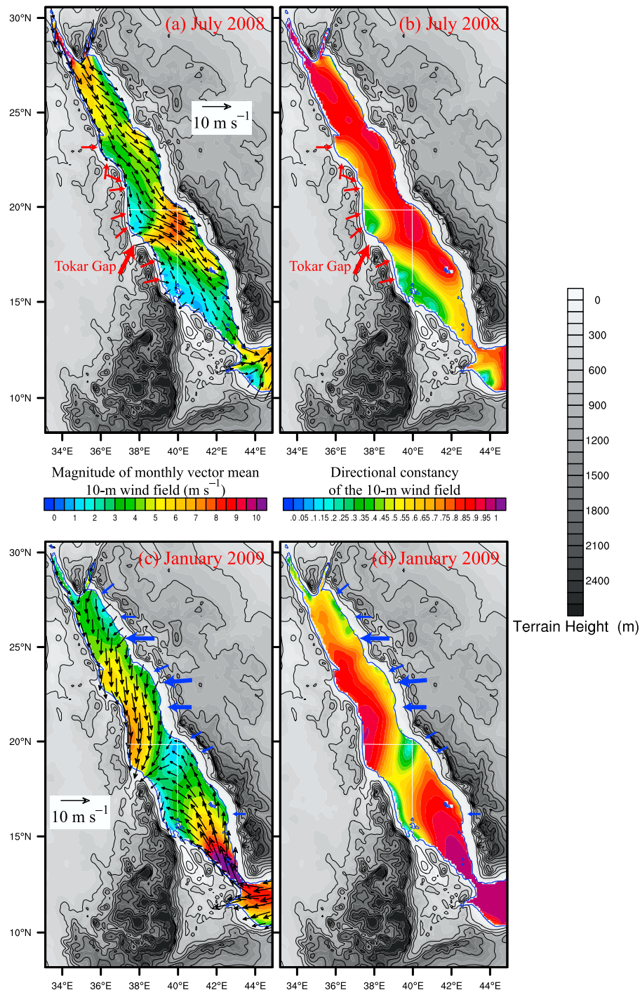
Figure 1. Monthly means of 10-m surface winds over the Red Sea from hourly WRF model output. (a) July 2008 monthly vector mean 10-m surface wind vector field overlapped with its magnitude (color contours). (b) July 2008 monthly mean 10-m wind directional constancy (color contours), defined as the ratio of the magnitude of the monthly mean 10-m wind vector to the monthly mean 10-m wind speed. (c)–(d) Same as Figures 1a–1b but for January 2009. The red (blue) arrows in Figures 1a–1b (Figures 1c–1d) indicate the locations of mountain gaps along the western (eastern) coast of the Red Sea. The wind vectors are shown for \sim 30\% of the grid points.
