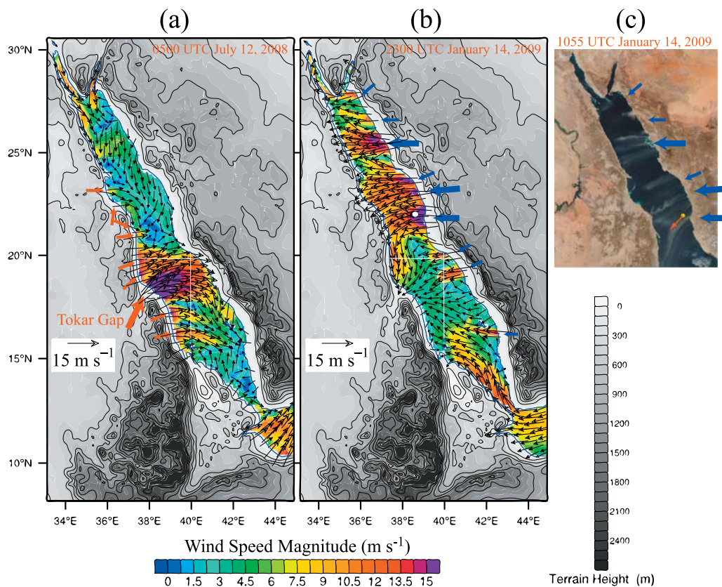
Figure 3. WRF model output of 10-m surface wind vector field overlapped with its magnitude (color contours) over the Red Sea region at (a) 0500 UTC 12 July 2008 and (b) 2300 UTC 14 January 2009. The wind vectors are shown for \sim 44\% of the grid points. (c) Dust plumes blew off the coast of Saudi Arabia and over the Red Sea in mid-January 2009. The Moderate Resolution Imaging Spectroradiometer (MODIS) on NASA's Aqua satellite captured this image at 1055 UTC 14 January 2009. The red arrows in Figure 3a indicate the locations of mountain gaps along the western coast of the Red Sea. The blue arrows in Figures 3b and 3c indicate the locations of mountain gaps along the eastern coast of the Red Sea. The white dot in Figure 3b and yellow dot in Figure 3c indicate the buoy location, and the red arrow in Figure 3c indicates the buoy wind direction.
