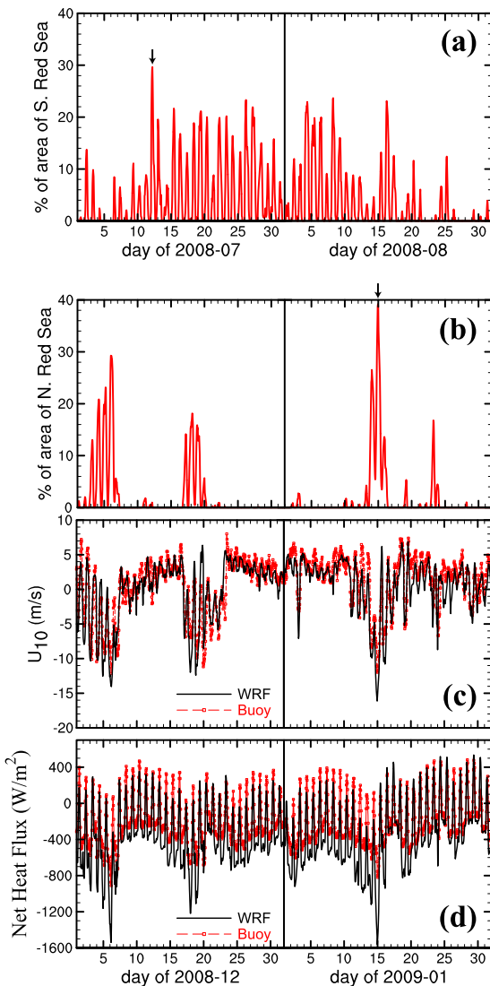
Figure 2. (a) Time series (July–August 2008) of the area percentage of the southern Red Sea (south of 20°N), over which the eastward 10-m zonal winds were greater than 10 \text{ m s}^{-1} . The small black arrow indicates the time of 0500 UTC 12 July 2008. (b) Time series (December 2008 to January 2009) of the area percentage of the northern Red Sea (north of 20°N), over which the westward 10-m zonal winds were greater than 10 \text{ m s}^{-1} . The small black arrow indicates the time of 2300 UTC 14 January 2009. Time series (December 2008 to January 2009) of buoy measured and WRF simulated (at the buoy location) (c) 10-m zonal winds and (d) net heat flux with negative values indicating ocean heat loss.
