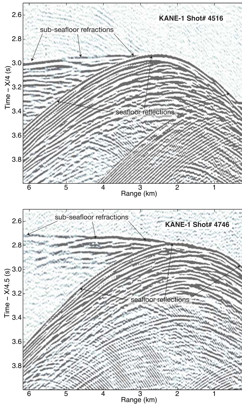
Figure 2. Representative shot gathers from profile K1 over the Kane OCC. Horizontal axes are distances from source to receivers along the streamer, and vertical axes are reduced two-way traveltimes (reduction velocities of 4 \text{ km s}^{-1} and 4.5 \text{ km s}^{-1} , top and bottom, respectively).
