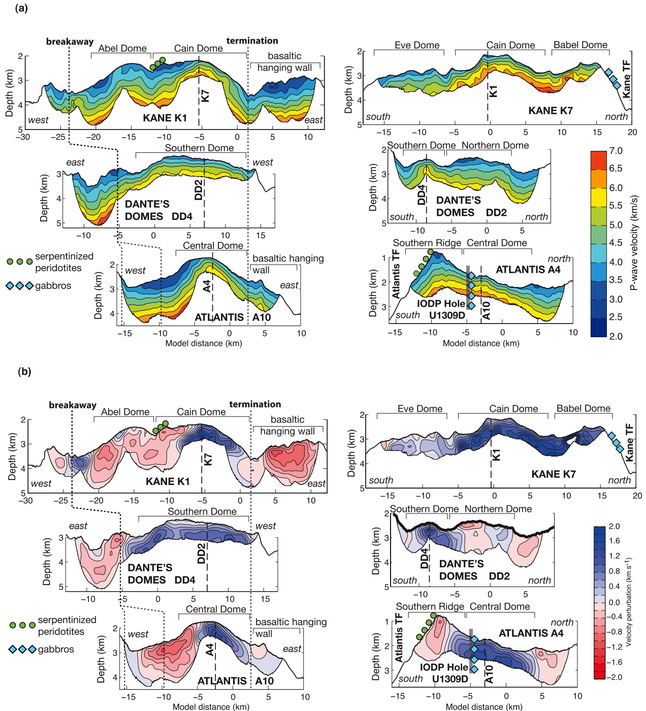
Figure 6. (a) Two-dimensional tomography models of P wave velocity beneath Kane, Dante's Domes, and Atlantis OCCs (profile locations in Figure 1). Contours are every 0.5 \text{ km s}^{-1} . Left panels are dip profiles, and right panels are strike profiles. Short-dashed lines on dip profiles indicate locations of breakaways and terminations. Long-dashed lines show crossings between dip and strike profiles. Green dots and blue diamonds (serpentinite and gabbro, respectively) show dominant in situ lithologies sampled by submersible or remotely operated vehicle [Auzende et al., 1994; Dick et al., 2008; Karson et al., 2006] or drilled [Blackman et al., 2006] (IODP Hole U1309D, vertical gray line projected onto profile A4). (b) Same as Figure 6a with models shown as perturbations with respect to the initial one-dimensional velocity model (Figure 4), with contours every 0.2 \text{ km s}^{-1} .
