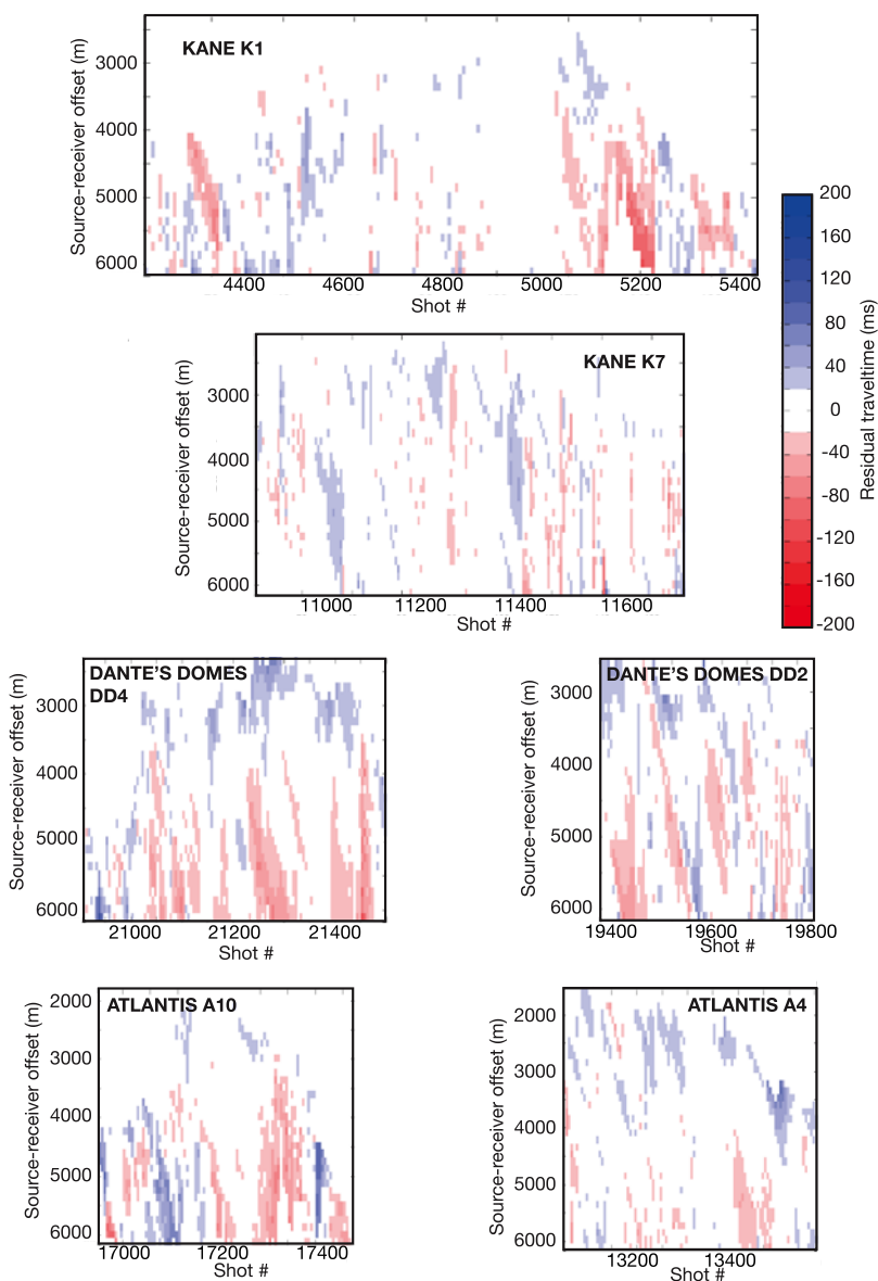
Figure 9. Color plots showing residual traveltimes predicted by the final models displayed as a function of shot number and source-receiver offset for each of the seismic profiles.
