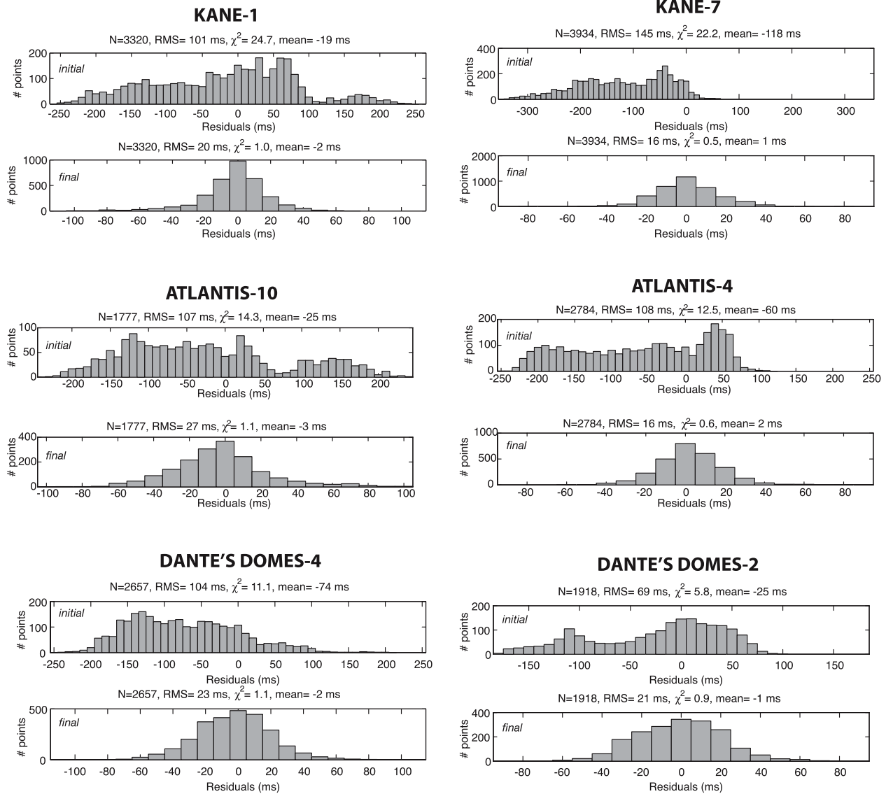
Figure 8. Traveltime residual histograms. Results of both initial and final models are shown for each seismic profile. N indicates number of observations, RMS is root-mean squared, \chi^2 is weighted misfit function, and mean is the mean of the distributions.
