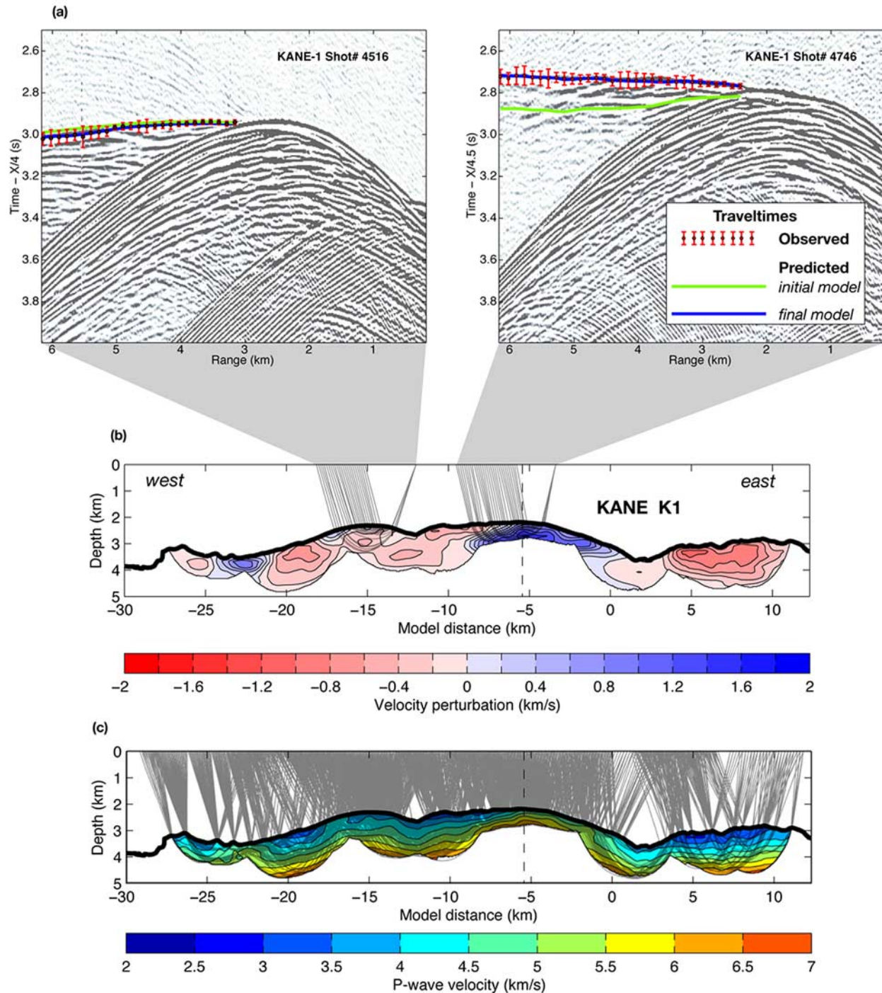
Figure 7. (a) Shot gathers from Figure 2 with observed traveltimes and their assigned uncertainty (circles with red error bars). Traveltimes curves are shown as predicted by the initial model (green, from Figure 4) and the final model in Figure 6 (blue). (b) Final velocity model for profile K1, shown as perturbations with respect to the initial model, and contoured every 0.2 km s -1 . Raypaths (gray lines) for the two source-receiver pairs in Figure 7a, above, are shown. (c) Final velocity model for profile K1 with complete ray coverage and contours every 0.5 km s -1 .
