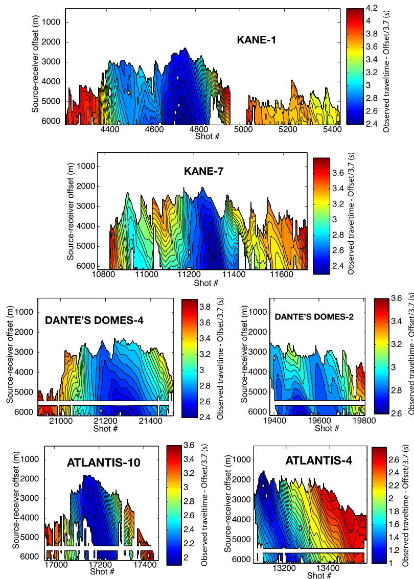
Figure 3. Color plots showing observed traveltimes picks (two-way traveltimes reduced at 3.7 \text{ km s}^{-1} ) displayed as a function of shot number and source-receiver offset for each of the seismic profiles. White areas indicate that no traveltimes were picked for a particular shot-receiver pair because of noisy data or because subsurface refractions arrive later than the seafloor reflection at short offsets.
