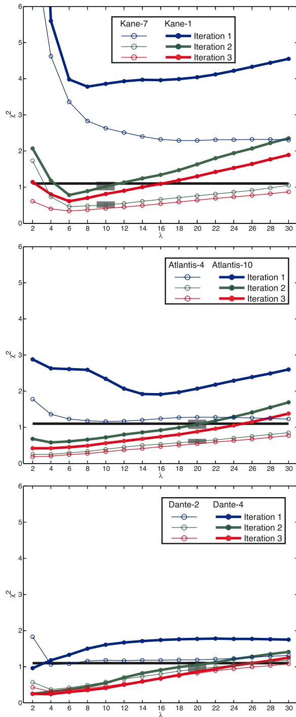
Figure 5. Variation in misfit function between observed and predicted traveltimes as a function of damping parameter \lambda , for several inversion iterations. Gray squares indicate the preferred solutions shown in Figure 6. Black line corresponds to \chi^2 = 1.1 , the adopted threshold value for the misfit function.
