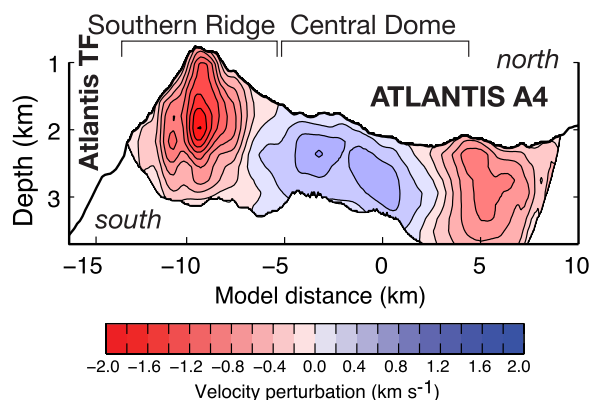
Figure 11. Alternate solution for profile A4 across Atlantis OCC shown as perturbations with respect to the initial one-dimensional velocity model labeled as “A4 alternate initial” in Figure 4; contours are every 0.2 \text{ km s}^{-1} .
