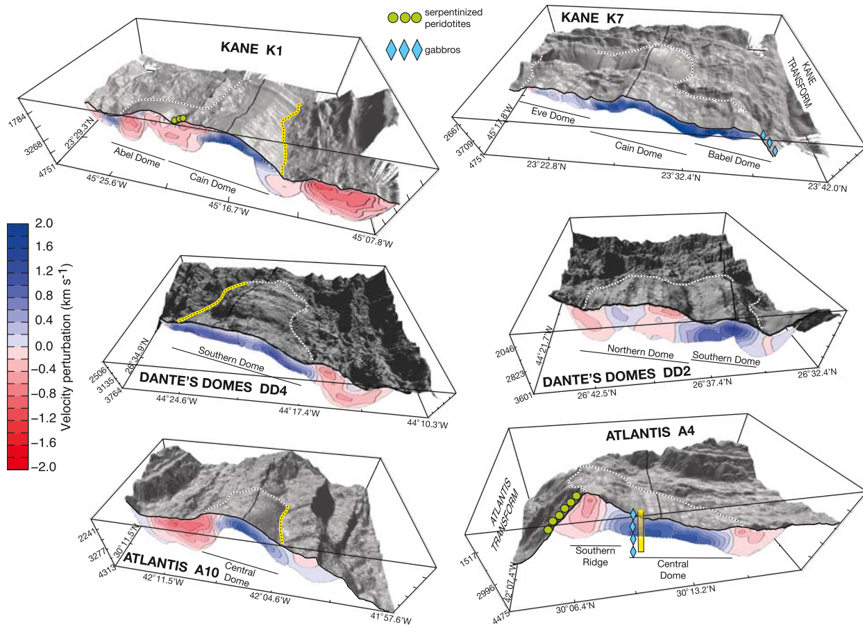
Figure 12. Three-dimensional renditions of seafloor topography (shaded gray) with intersecting vertical sections of the velocity profiles (red-blue images showing velocity perturbations as in Figure 6b, contoured every 0.2 \text{ km s}^{-1} ). Left panels show dip sections, and right panels show strike sections. Blue and red areas indicate velocities faster and slower than the reference model, respectively. Dashed lines on the seafloor topography indicate the limits of dominantly smooth, corrugated detachment surfaces; yellow segments show detachment terminations. Solid black lines draped on the seafloor locate the orthogonal seismic profiles at each OCC. Colored dots and diamonds are in situ lithologies as in Figure 6. Vertical yellow bar in profile A4 locates IODP Hole U1309D. Primary morphological features are labeled. Horizontal axes are latitude and longitude, and vertical axes show depth below sea level in meters.
