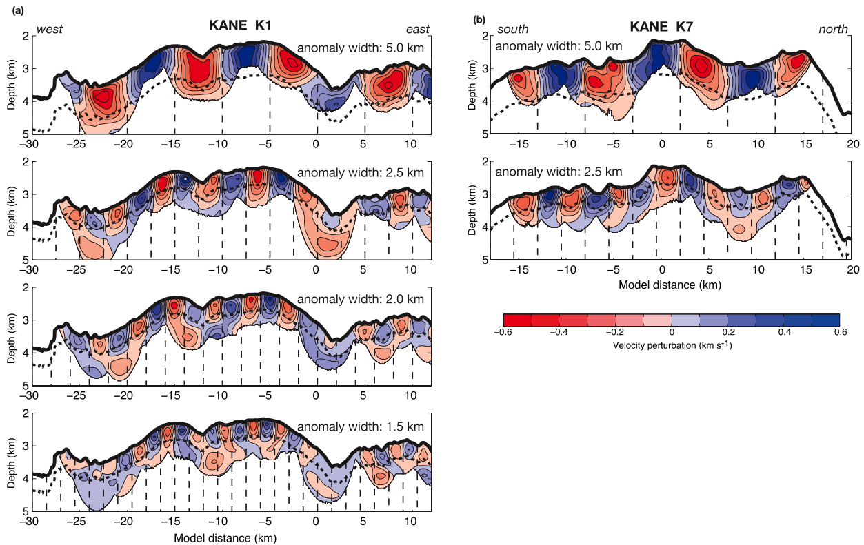
Figure 10. Resolution tests for profiles (a) K1 and (b) K7 of the Kane OCC. Red-blue anomalies show recovered synthetic anomalies. Vertical long-dashed lines locate the alternating positive and negative true anomalies (widths indicated within each panel). Short-dashed lines correspond to a subseafloor depth of 0.5 km, except for the top panels, where it corresponds to 1 km subseafloor depth.
