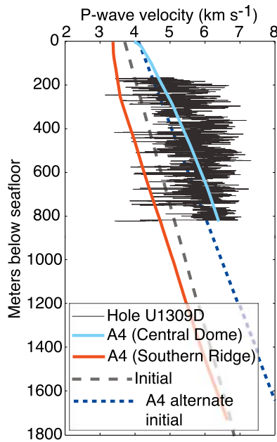
Figure 4. One-dimensional velocity structures at Atlantis OCC extracted from profile A4 beneath the Central Dome at the location closest to Hole U1309 (blue) and beneath the Southern Ridge at -9.5 km model distance (red). Solid black line shows sonic-log velocities measured in situ within the upper \sim 200 – 800 m of IODP Hole U1309D [Blackman et al. , 2006]. Long-dash gray line shows the initial velocity model used in our tomography inversions. Short-dash blue line shows an alternate initial velocity model for profile A4 that was used to obtain the results shown in Figure 11.
