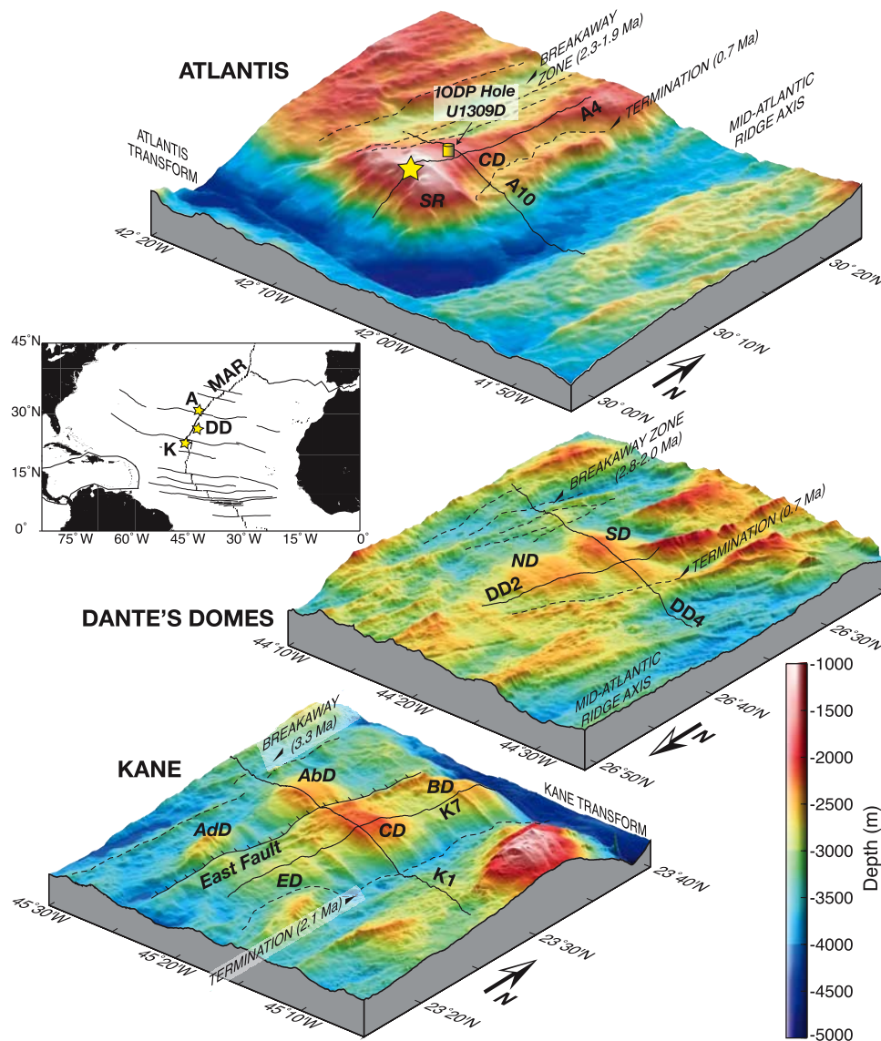
Figure 1. Shaded-relief, three-dimensional perspectives of multibeam bathymetry over Atlantis, Kane, and Dante's Domes OCCs. (Note the different view angle of the Dante's Dome image). Solid lines locate seismic profiles (numbered with A, DD, and K). Dashed lines show locations of breakaways and terminations of detachment faults. SR and CD are the Southern Ridge and Central Dome, respectively, of Atlantis OCC; ND and SD are the northern and southern domes, respectively, of Dante's Domes OCC; and AD, BD, CD, and ED are the Abel, Babel, Cain, and Eve domes, respectively, of Kane OCC. Yellow star on Atlantis OCC locates the Lost City hydrothermal field. The inset at left shows the location of the three OCCs on the flanks of the MAR in the northern central Atlantic.
