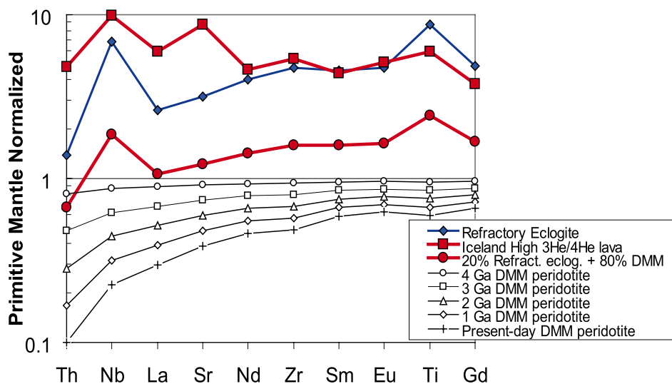
Figure 4. Spidergram of McDonough's [1991] refractory eclogite used in the modeling, including spidergrams demonstrating the time-dependent trace element composition of DMM. In the mixing models shown in Figure 2, the lithospheric peridotite and refractory eclogitic portions of a 3 Ga subducted plate are mixed together such that the final mixture has 20–25% eclogite. This mixing calculation is shown in the spidergram, where 20% ancient (3 Ga), refractory eclogite has been added to peridotite from the deepest portion of same age oceanic mantle lithosphere (with the same peridotite composition as DMM at 3 Ga). Refer to Table 3 for compositions of the 3 Ga refractory eclogite and the 3 Ga peridotite. Excluding Sr (see text for discussion of shallow lithospheric contamination and the resulting Sr-anomalies in some Icelandic lavas), the shape of the hybrid peridotite-eclogite spidergram, including the positive Nb and Ti anomalies, is very similar in shape to the spidergram of the high ^3\text{He}/^4\text{He} Icelandic lava. This similarity is consistent with the hybrid peridotite-eclogite being the source of the high ^3\text{He}/^4\text{He} mantle sample by OIBs.
