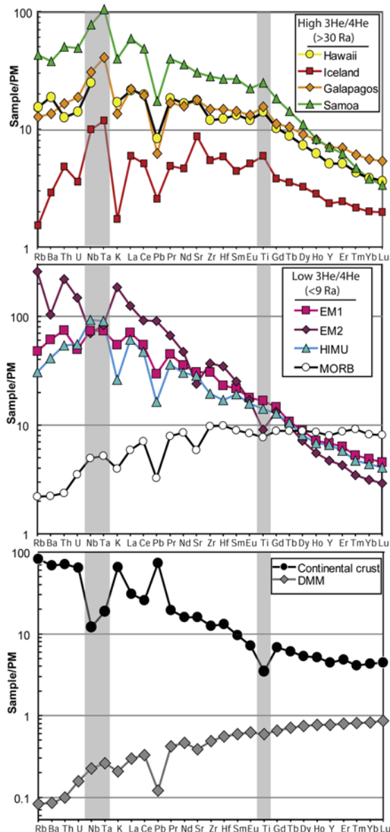
Figure 1. Titanium, tantalum, and niobium (TITAN) are highly enriched in ocean island basalts (OIBs) with high ^3\text{He}/^4\text{He} . (top) Primitive mantle (PM) normalized trace element data (spidergrams) for basalts with the highest ^3\text{He}/^4\text{He} (>30 Ra) from 4 different hot spots. All high ^3\text{He}/^4\text{He} samples exhibit TITAN enrichment relative to neighboring elements on the spidergrams. (middle) Spidergrams for the low ^3\text{He}/^4\text{He} (<9 Ra) mantle end-members. EM1 lavas are from Pitcairn, EM2 lavas are from Samoa, and HIMU lavas are from Mangaia and Tubuaii. Spidergrams for the mantle end-members and MORB are from Hart and Gaetani [2006] and (for EM2) Jackson et al. [2007a]. TITAN enrichment is not as pronounced, or is absent, in the average spidergrams of the low ^3\text{He}/^4\text{He} mantle end-members. (bottom) Spidergrams for DMM [Workman and Hart, 2005] and continental crust [Rudnick and Gao, 2003] indicate that these two shallow earth reservoirs are not entirely geochemically complementary: TITAN depletion in the continents is not balanced by corresponding enrichment in DMM. However, the TITAN-enrichment in high ^3\text{He}/^4\text{He} lavas suggests that these lavas sample a (deeper) mantle reservoir that hosts part of the TITAN that is missing in the shallow geochemical reservoirs, DMM, and continental crust. Sources of the ^3\text{He}/^4\text{He} data for the mantle end-members and the high ^3\text{He}/^4\text{He} lavas can be found in the text and in Table 1.
