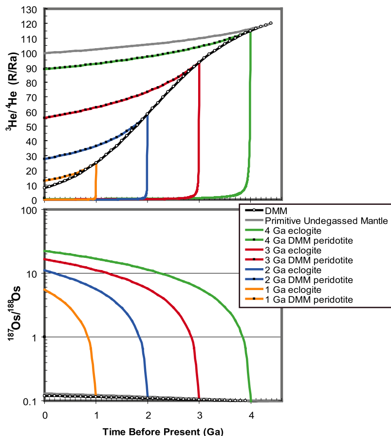
Figure 3. Time evolution of ^3\text{He}/^4\text{He} and ^{187}\text{Os}/^{188}\text{Os} of DMM, ancient subducted lithospheric peridotite, and eclogite. (top) At 4.4 Ga, DMM starts forming by melt extraction from primitive mantle to form continental and oceanic crust, and the ^3\text{He}/^4\text{He} trajectories of DMM and the (hypothetical) primitive undegassed mantle separate immediately. Due to continuous depletion by melt extraction, DMM evolves low ^3\text{He}/^4\text{He} . Portions of the ancient lithospheric peridotite, which compose the lowermost portion of downgoing slabs, are sent into the lower mantle throughout geologic time. Model curves are shown at 1 Ga intervals, and this is not intended to imply that the isolation of oceanic plates is episodic. The isolated peridotite portions of the downgoing slabs are modeled as having exactly the same U, Th/U, ^{238}\text{U}/^3\text{He} , and ^3\text{He}/^4\text{He} as ambient DMM at the time of isolation, and they preserve higher ^3\text{He}/^4\text{He} than DMM due to their isolation from further melt depletion. Also shown is the concomitant subduction of the eclogitic portions of the same slabs, which begin with the same ^3\text{He}/^4\text{He} as DMM at the time of subduction; the U and Th of the subducted refractory eclogite are from McDonough [1991] and are shown in Table 3. To simulate degassing, the ^{238}\text{U}/^3\text{He} of the eclogite is increased by a factor of 1000 relative to the contemporary DMM composition, and as a result the ^3\text{He}/^4\text{He} ratios of the subducted eclogites rapidly decrease. (bottom) The ^{187}\text{Os}/^{188}\text{Os} of Primitive Mantle (0.130 [ Meisel et al. , 2001]) and DMM (0.125 [ Standish et al. , 2002]) are very similar. The time evolution of ^{187}\text{Re}/^{188}\text{Os} of ancient subducted peridotite from the base of the oceanic mantle lithosphere is approximated by the trajectory of DMM in Figure 3 (a continuous depletion model is not used to describe the evolution of ^{187}\text{Os}/^{188}\text{Os} of DMM). The present-day ^{187}\text{Re}/^{188}\text{Os} of the refractory eclogite is from Becker [2000], and this composition generates increasingly radiogenic present-day ^{187}\text{Os}/^{188}\text{Os} for earlier isolation times. Refer to Appendix A and Table 3 for all parameters used in the model. When 20–25% of a refractory eclogite from an oceanic plate subducted at 3 Ga is mixed together with 75–80% of a peridotitic portion of the same plate, the models generate the ^3\text{He}/^4\text{He} and ^{187}\text{Os}/^{188}\text{Os} of the mantle sampled by the highest ^3\text{He}/^4\text{He} (>30 Ra) OIBs (see Figure 2 for mixing results). Note that the very radiogenic Os of the eclogite is vastly reduced in the mixture due to the low Os contents of the eclogite (6 ppt) and the high Os contents of the isolated DMM peridotite (3,000 ppt).
