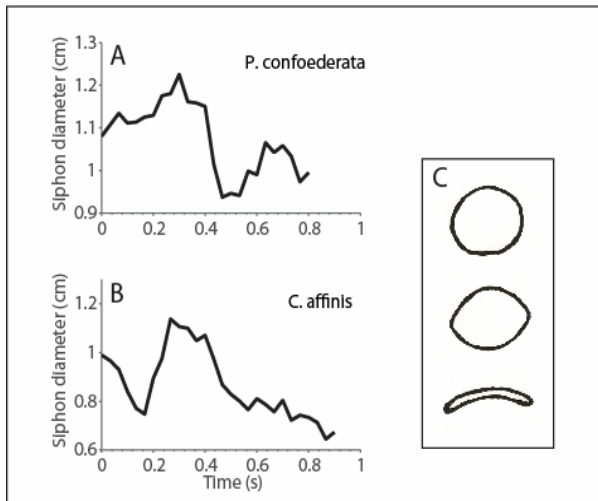
Fig. 3.3. Change in salp atrial siphon diameter d with time. (A) 63.3 mm-long P. confoederata , (B) 63.3 mm-long C. affinis and (C) cross section of P. confoederata atrial siphon over course of jet period sketched from salp swimming perpendicular to 1-mm thick laser sheet.
