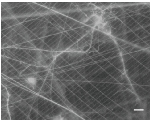
Fig. 4.3. Microscope image of fluorescently stained P. confoederata mucous filtering mesh. Scale bar is 5 \mu\text{m} .
