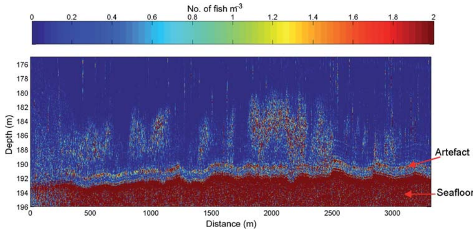
Figure 8. Numerical density of Atlantic herring as determined through resonance classification using the low-frequency acoustic channel. Data are from same transect as in Figure 5, but over a greater distance. There is an artefact in the data, just above the seafloor, associated with the high echo level from the seafloor.
