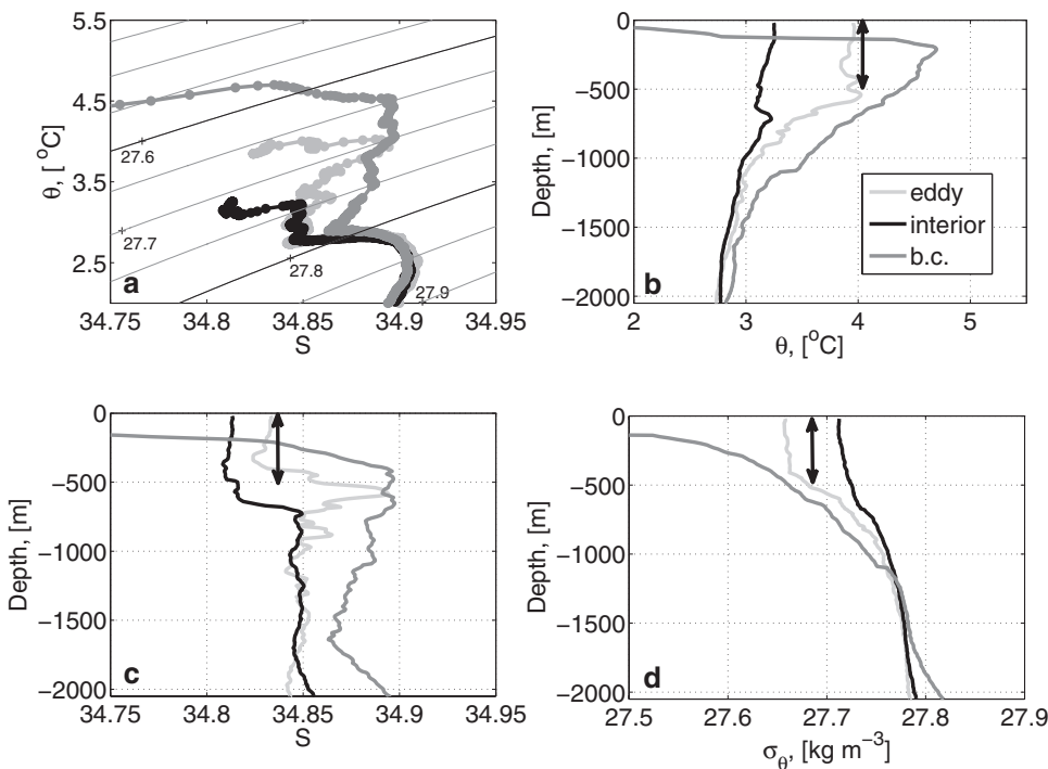
Figure 5. A convected eddy observed in winter of 1997. (a) \theta/S diagram; (b) potential temperature; (c) salinity; (d) potential density in the eddy (gray), interior (black) and boundary current (b. c., dark gray). The mixed layer in the eddy is indicated with an arrow.
