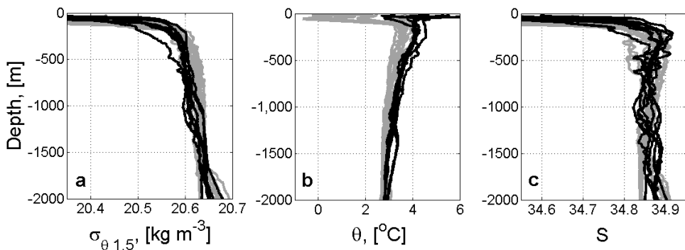
Figure 10. Unconvected ICAs observed pre-1997 (gray) and post-1997 (black): (a) potential density referenced to 1500 m; (b) potential temperature; (c) salinity.
