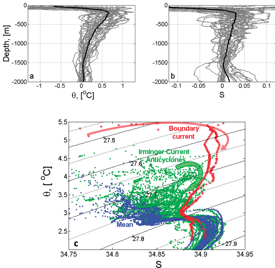
Figure 3. Characteristics of the ICAAs: (a) potential temperature and (b) salinity anomalies (gray) for all ICAAs relative to the interior (see text); the average anomaly is shown in black; (c) \theta/S diagram for ICAAs (green), Labrador Sea interior (blue) and two typical profiles from the West Greenland Current (red). The arrow indicates schematically the elbow in \theta/S space associated with the ICAAs.
