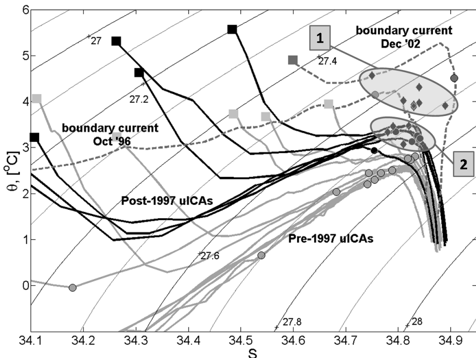
Figure 8. Unconvected pre-97 (light gray), post-97 (black) ICA and boundary current (dark gray dashed) mixed layer evolution trajectories. Diamonds show the properties of observed mixed layers in cICAs while the circles on each trajectory indicated the estimated mixed layer properties given a realistic buoyancy loss (see text). The squares mark the surface initial conditions for each profile. The shaded ellipses indicated the two clusters of cICAs described in the text.
