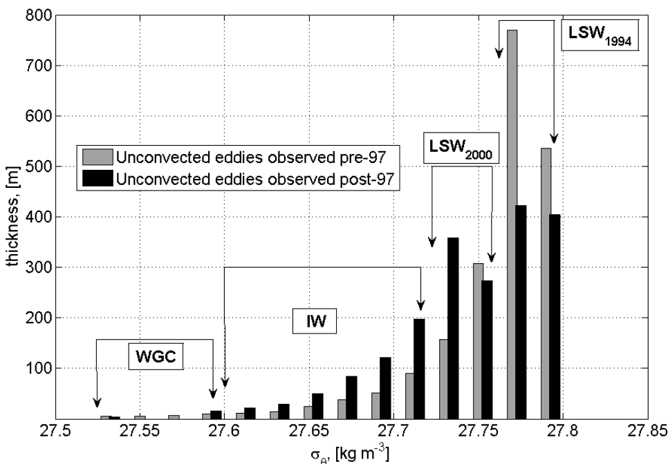
Figure 11. Layers' thickness in the unconvected ICAs (gray—pre-1997 and black—post-1997). The principal water masses and their density ranges are labeled.
