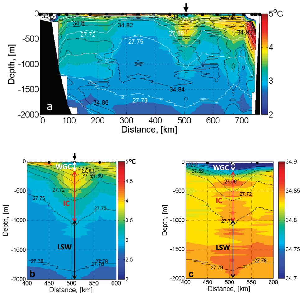
Figure 2. (a) A hydrographic section of potential temperature \theta (color), salinity (black contours) and potential density \sigma_\theta (white contours) across the Labrador Sea sampled in May 1997. The arrow marks the location of an ICA. (b) Potential temperature and (c) salinity in the ICA (May 1997) with arrows indicating different water masses and black dots representing positions of the hydrographic stations.
