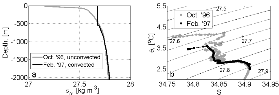
Figure 7. Potential density (left) and \theta/S diagram (right) of a convected (Feb. 1997) and an unconvected (Oct. 1996) ICA.
