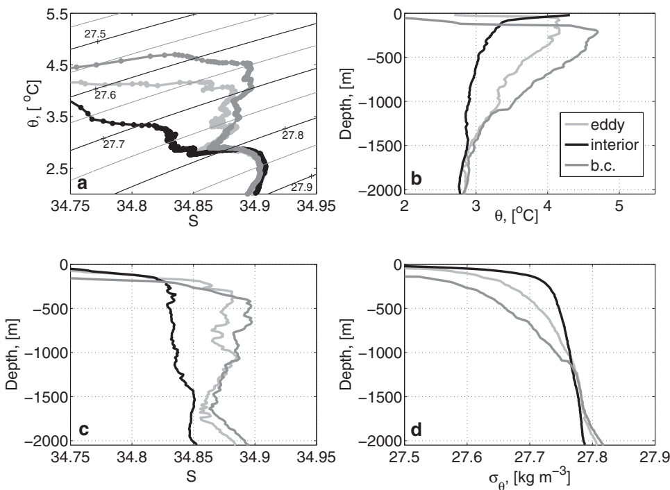
Figure 4. (a) \theta/S diagram; (b) potential temperature; (c) salinity; and (d) potential density for the unconvected eddy observed in spring of 1997 (gray), the interior (black), and the boundary current (dark gray).
