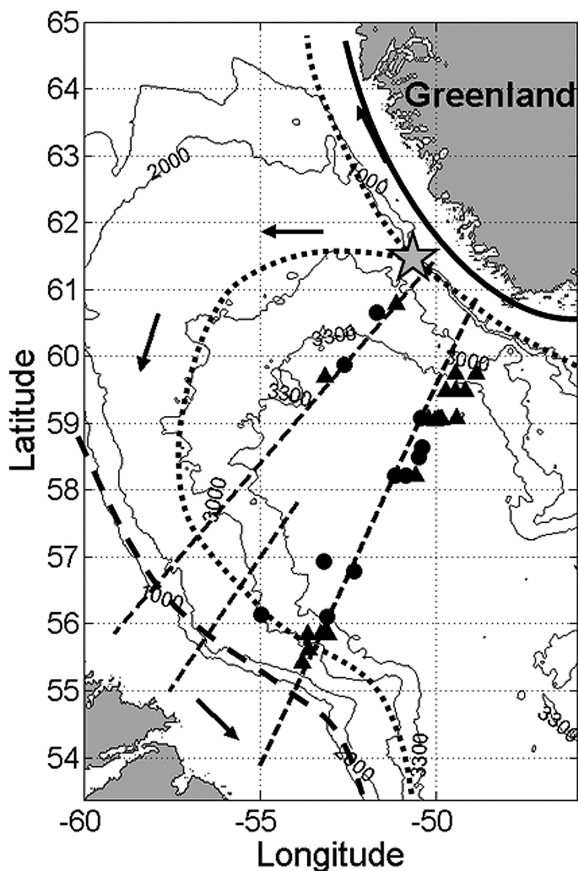
Figure 1. Schematic circulation of the Labrador Sea overlaid on the bathymetry (thin black lines with numbers indicating the depths of 1000, 2000, 3000 and 3300 m). The southernmost section (AR7W) and the other two sections occupied are shown by the thin dashed lines. The West Greenland Current (WGC) is shown by a solid line, the Irminger Current (IC) by a thick dotted line, and the Labrador Current is shown by a thick dashed line. Arrows represent the direction of the flow. The star marks the approximate location of eddy formation. Symbols indicate the locations where the ICAs were found. Convected ICAs are identified by circles and unconvected ICAs by triangles.
