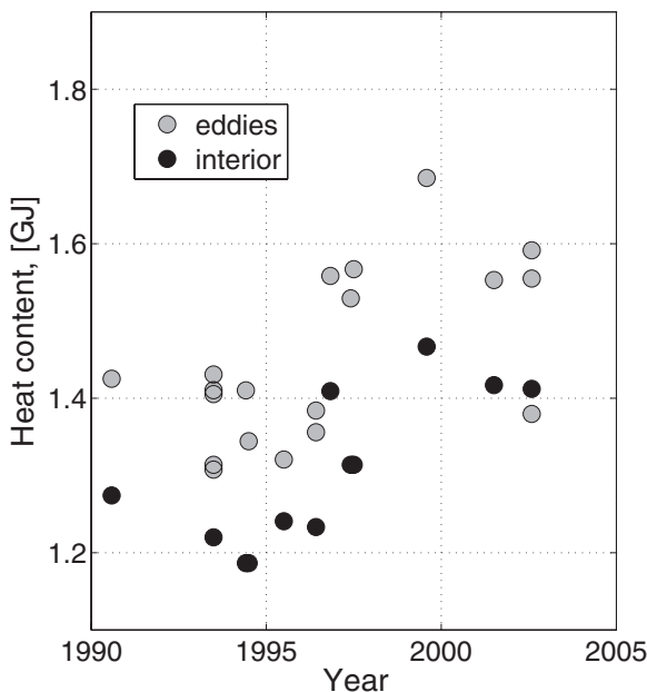
Figure 12. Heat content as a function of time in the interior and in the ICAs.
