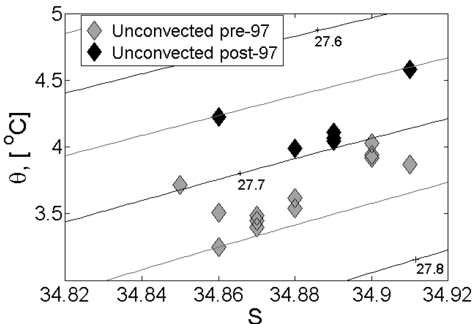
Figure 9. \theta/S diagram showing the core properties of the unconvected ICAs. Color shows the time of observation: pre-1997 (gray) and in 1997 and after (black).
