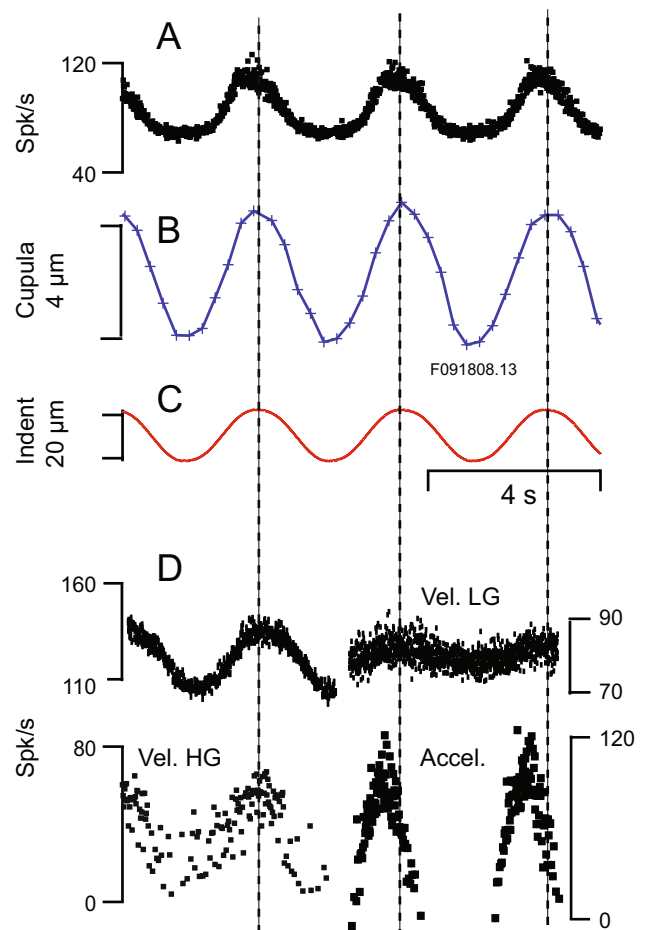
FIG. 2. Cupula displacement and afferent responses to 0.3-Hz sinusoidal stimuli in normal animals. Simultaneous recordings of afferent responses (A) and cupula displacement (B) in response to sinusoidal stimulus (C) at 0.3 Hz. D Additional afferents recorded in response to the same stimulus showed a range of gains and relative phases of peak response. Since 0.3 Hz is above the mechanical lower corner frequency, a subset of afferents responded in phase with, and in proportion to, cupula displacement (velocity-sensitive), while other afferents responded with a phase advance relative to cupula displacement (e.g., acceleration-sensitive).
