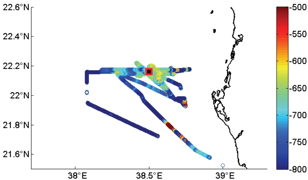
Figure III-5: Bathymetric survey track and uncorrected depth in meters. The mooring deployment site is indicated by a red/black square. A sound speed of 1500 m/s was assumed in estimating the uncorrected depth.
