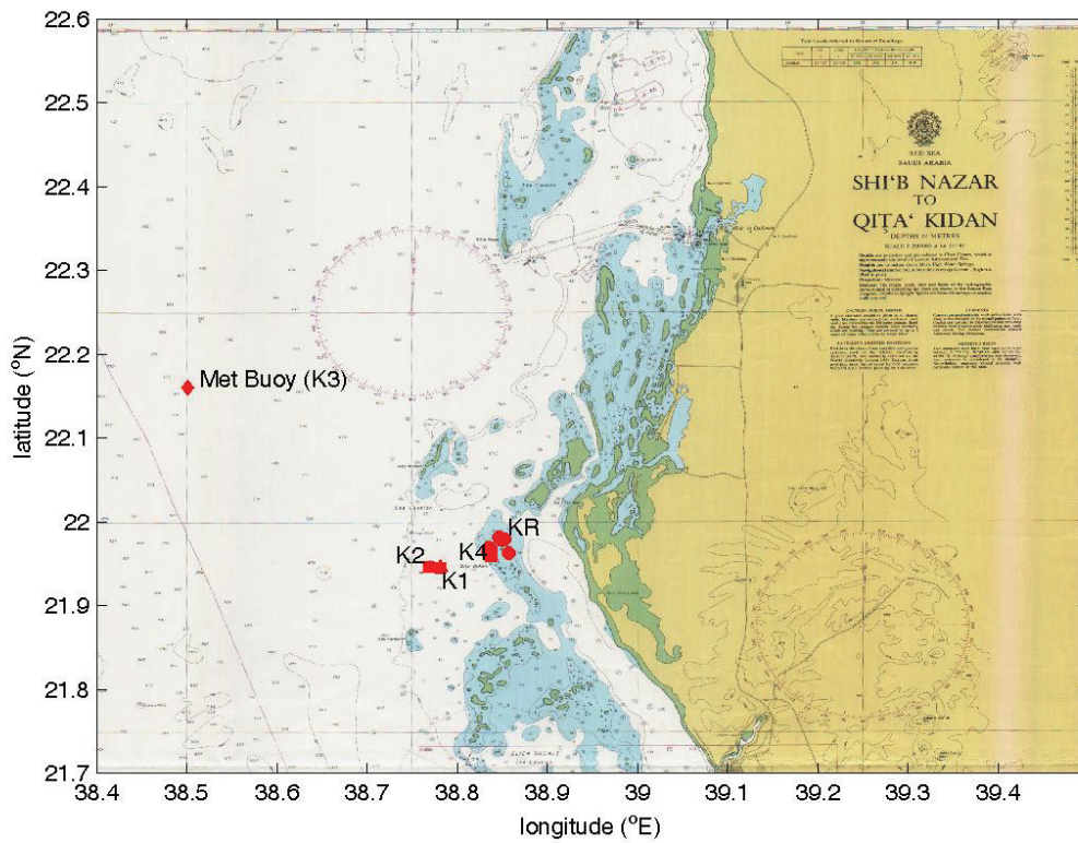
Figure IV-1: A fine-scale (upper) and a larger-scale (lower) view of the locations of the moorings and bathymetric survey lines, superimposed on an Admiralty chart of the eastern Red Sea.
