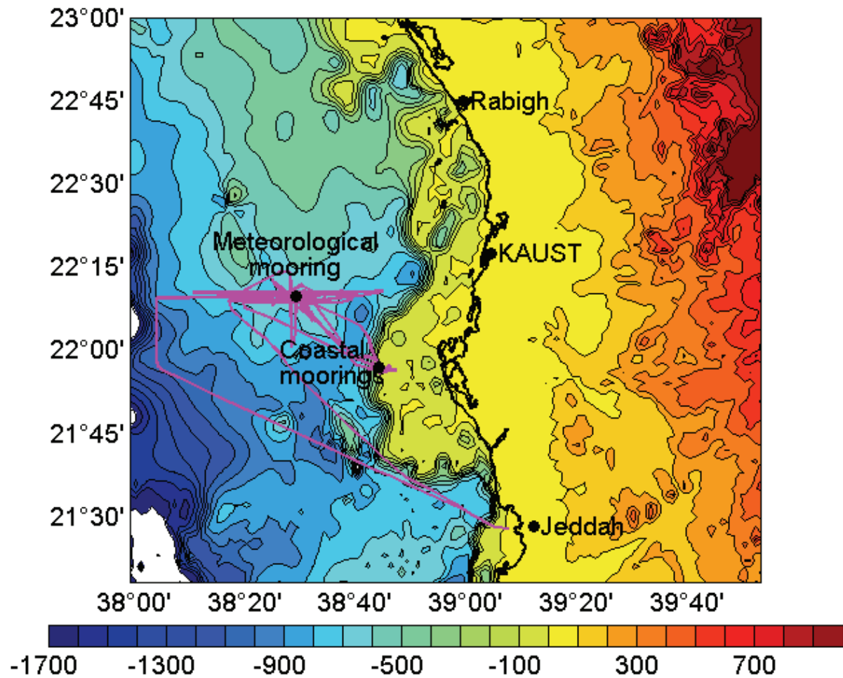
Figure II-2: The KAUST Fall 2008 Leg-1 cruise track (pink line). Background coloring and color scale indicate the ocean depth and land elevation in meters (from GEBCO 1-min bathymetry product).
