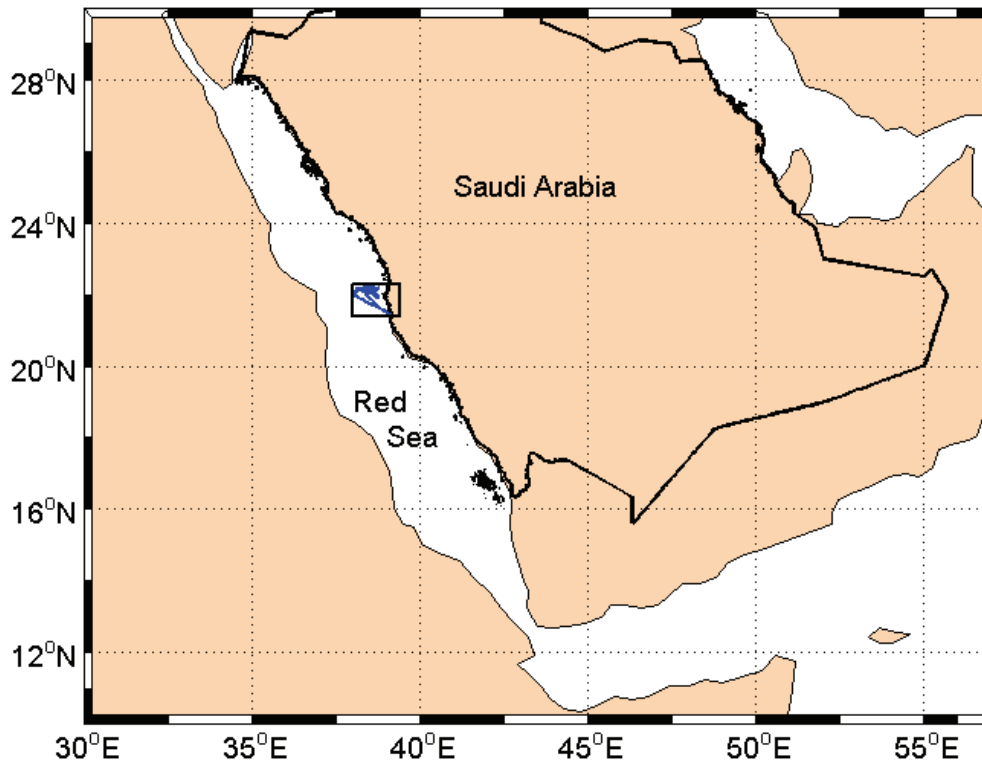
Figure II-1: The KAUST Fall 2008 Leg-1 area of operations in its large-scale context. The actual cruise track is indicated by a blue line. The cruise track is shown in more detail in Figure II-2.
