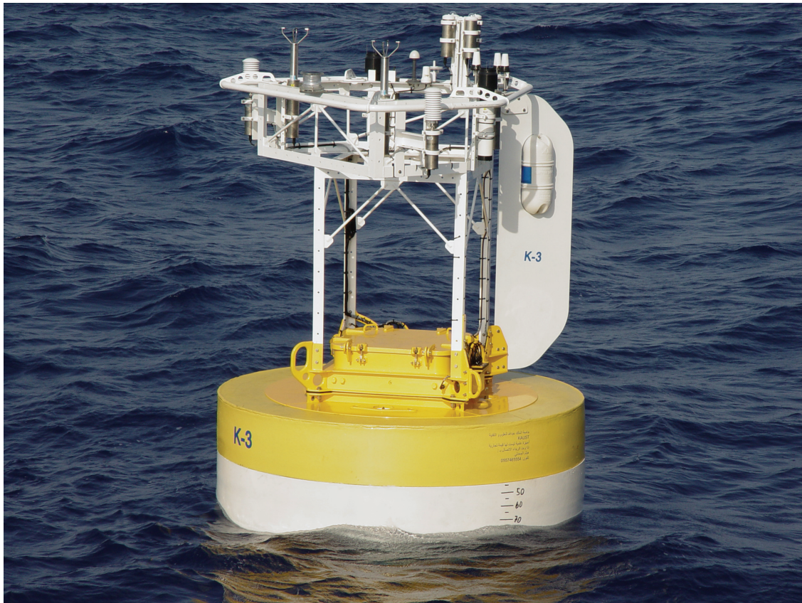
Figure III-2: Meteorological buoy after deployment. (Photo by Yasser Abualnaja.)
