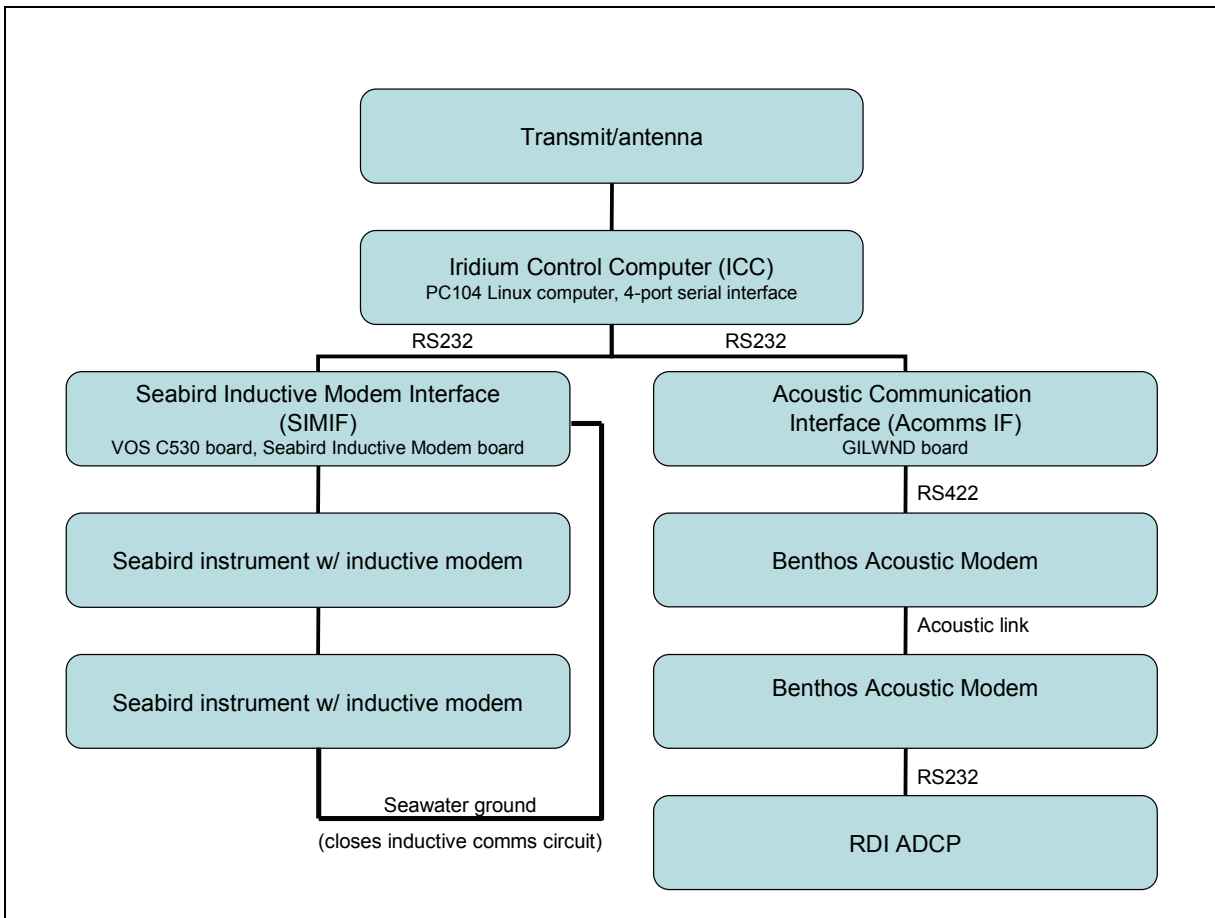
Figure III-4: Schematic of subsurface telemetry system.
