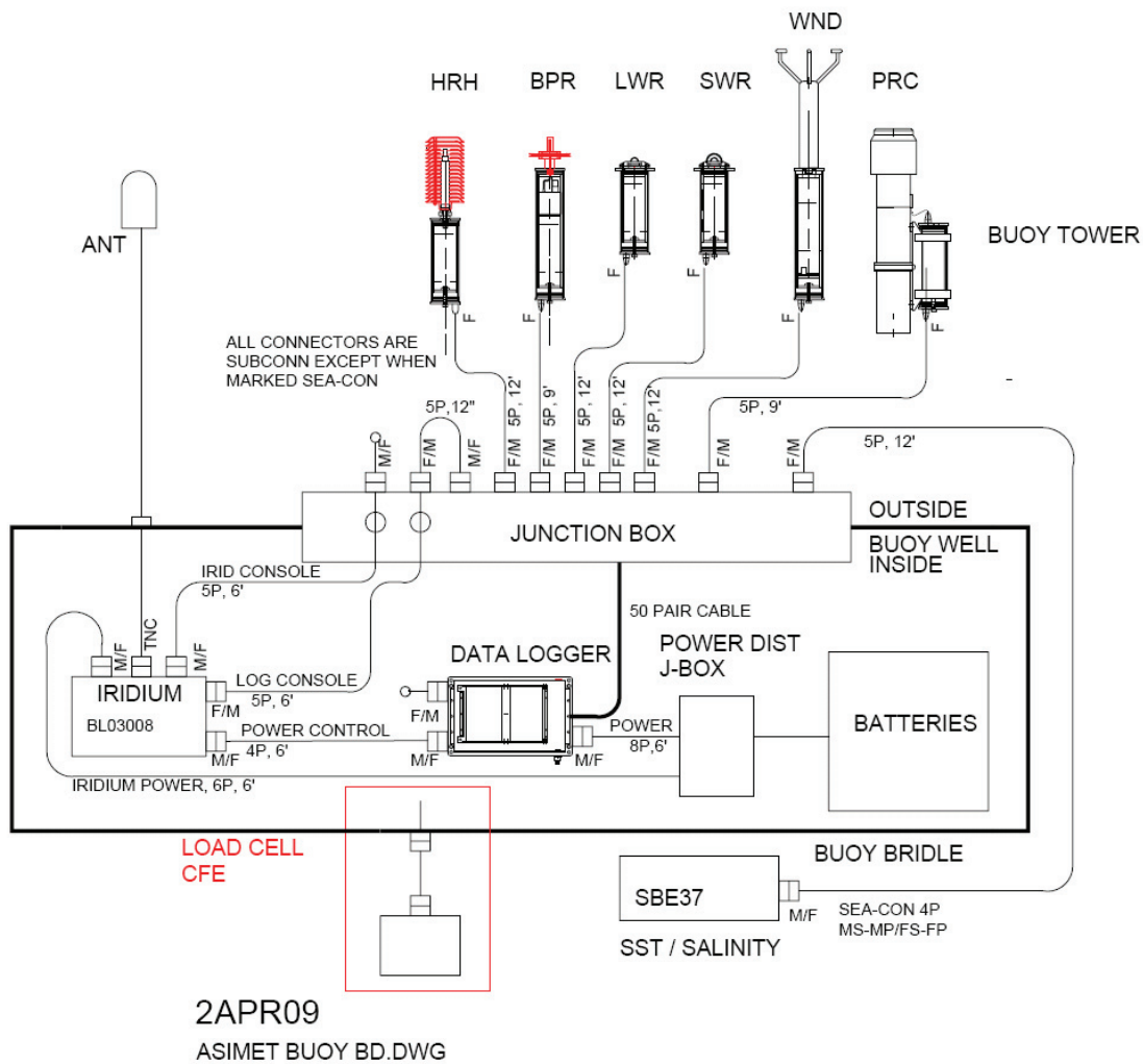
Figure III-1: Schematic representation of complete buoy meteorological system. The buoy carries two of these packages. Note that there is no load cell on the KAUST buoy.
