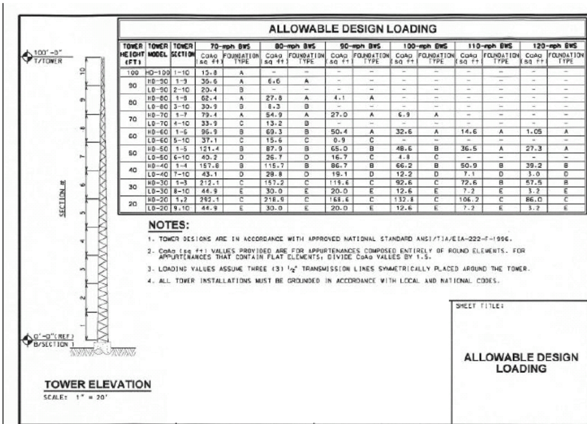
Figure VI-1: A table reproduced from the Glen Martin Engineering, Inc brochure for the “AN Self-supporting tower”. The HD-30 model used for KAUST is the bottom three sections of the 100-foot tower shown.
