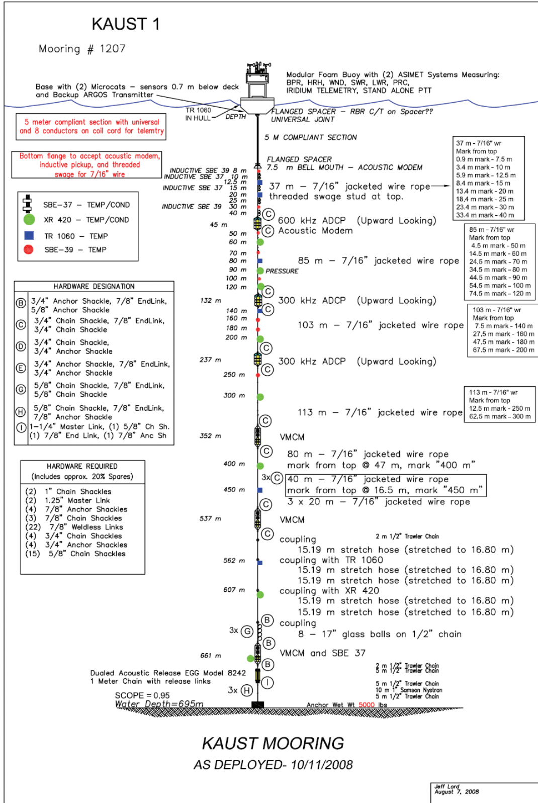
Figure III-3: Mooring Diagram for KAUST air-sea interaction mooring.
