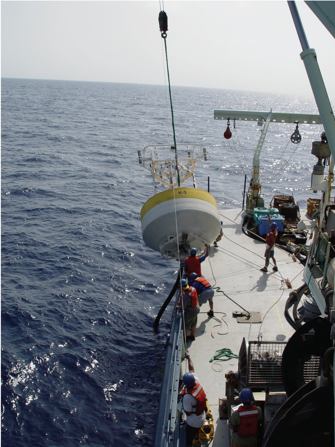
Figure III-7: Meteorological buoy during deployment. Note that there are no instruments clamped to the black EM Chain assembly below the buoy. (Photo by Yasser Abualnaja.)
