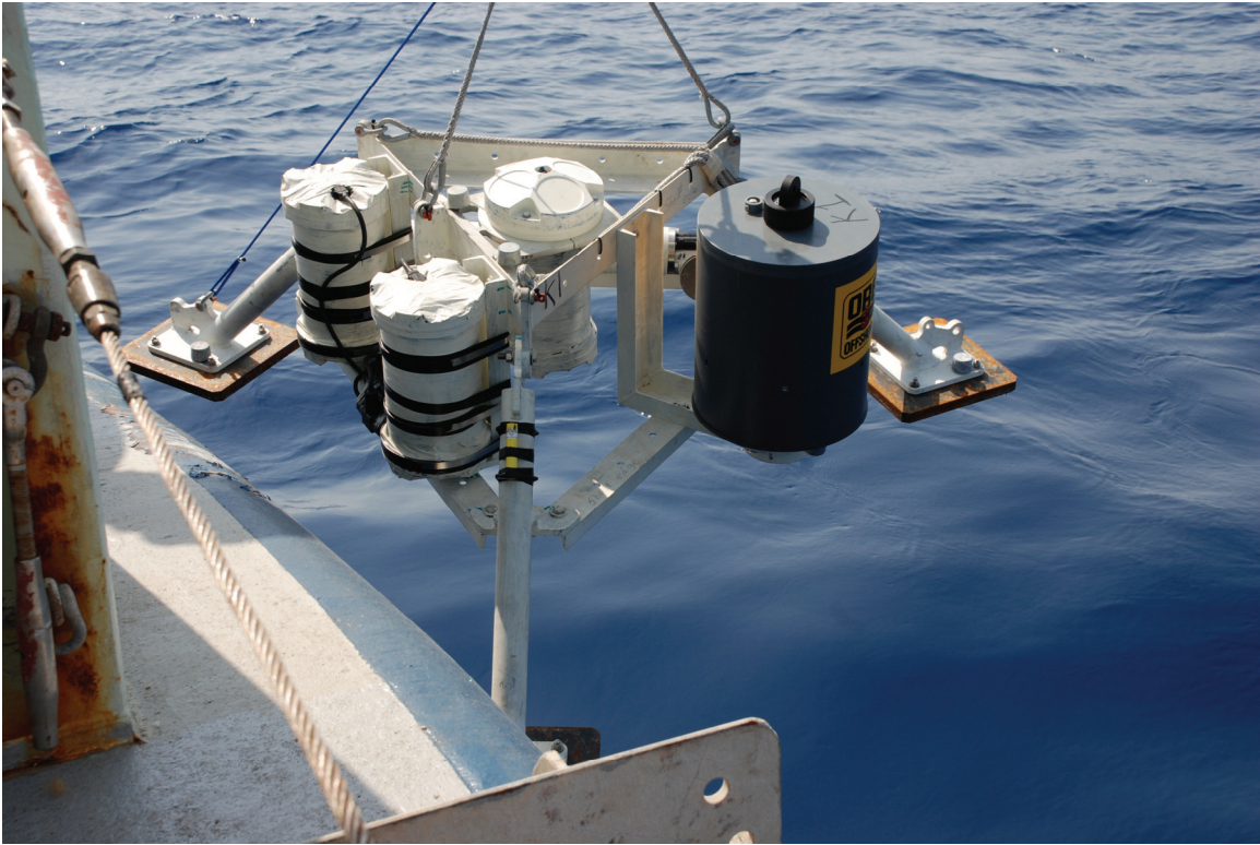
Figure IV-6: Deployment of the K1 (shelf-edge) bottom tripod. The instrument in the center of the frame is a 300-kHz ADCP. The white canisters attached to one side of the tripod house extra ADCP batteries. The gray canister is an ORE acoustic release unit housing 90 m of line for tripod recovery. The small yellow cylinder taped to the tripod leg closest to the viewer is an acoustic transponder. Attached to the leg furthest from the viewer, and not clearly visible here, is a Seaguage pressure recorder (photo courtesy of Susan Avery).
