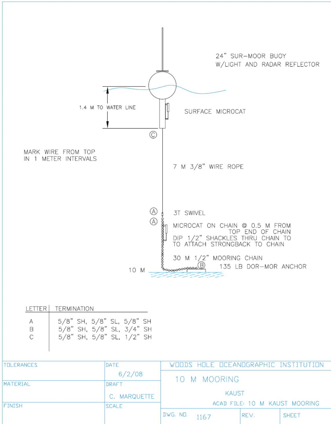
Figure IV-7: Mooring diagram for the reef-edge mooring.
