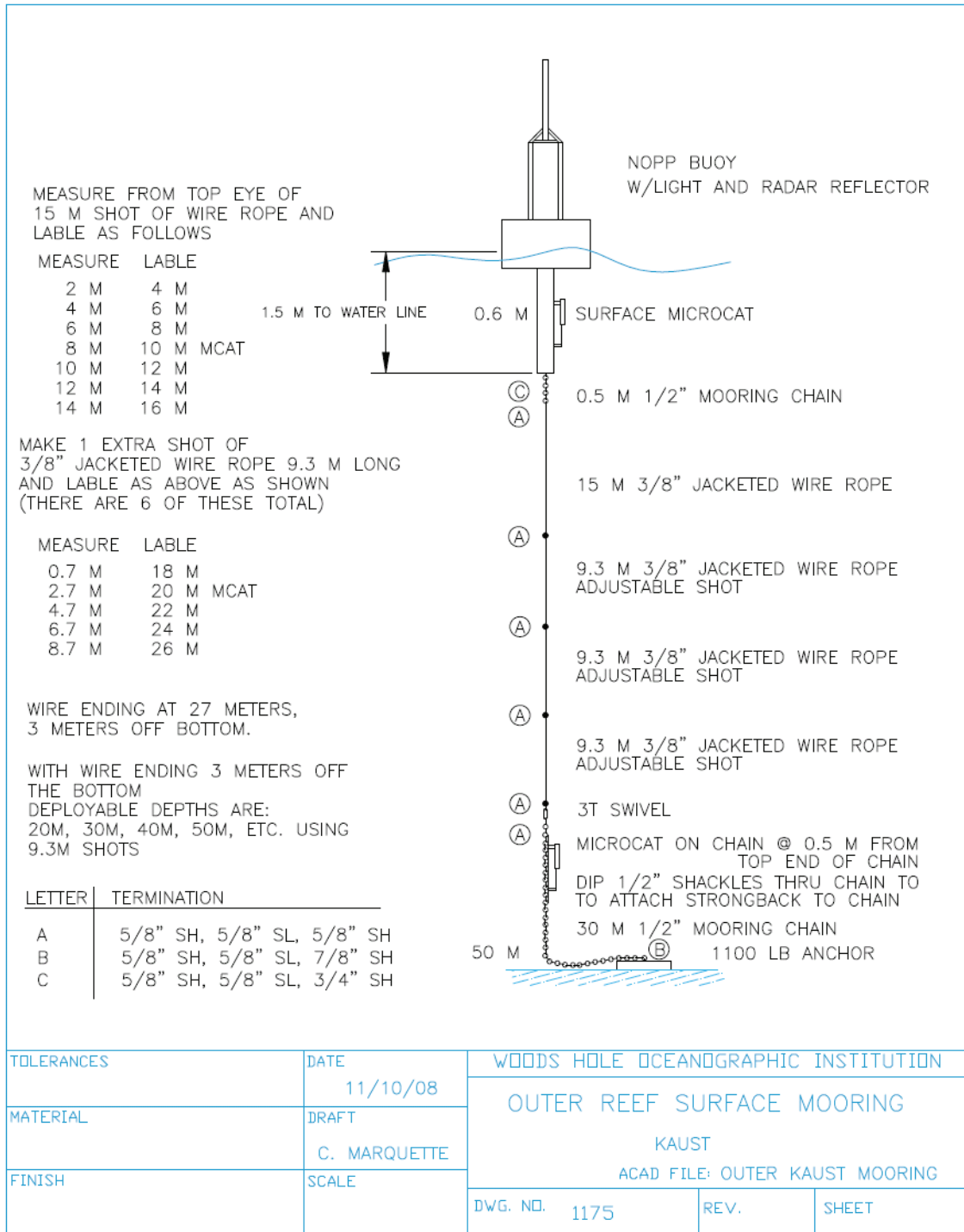
Figure IV-5: Mooring diagram for the K1 and K2 shelf moorings.
