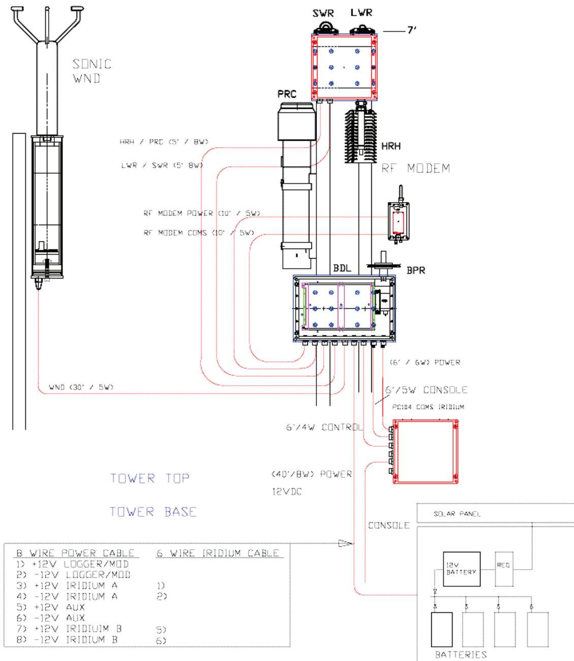
Figure VI-3: Schematic of tower meteorological system, including telemetry and power systems.
