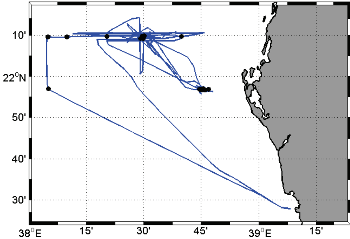
Figure V-1: Locations of all CTD stations (black circles) and cruise track (blue line).
