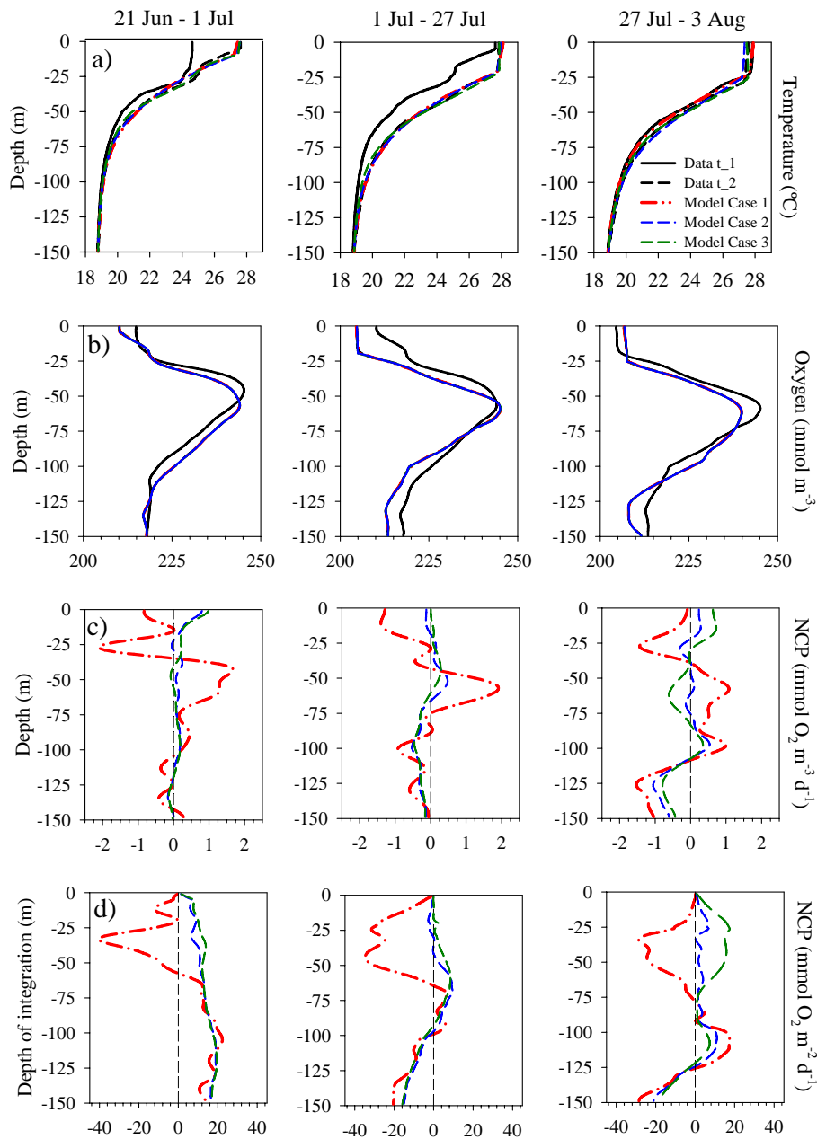
Fig. 2. Vertical distribution of temperature ( a ), oxygen ( b ), net community production ( c ) and depth-integrated net community production ( d ) at the center of cyclonic eddy C1 computed from the model runs Case 1 (red dot-dashed line), Case 2 (blue dashed line) and Case 3 (green dashed line), and for the initial ( t_1 ) and final ( t_2 ) in situ profiles of temperature (a) and oxygen (b). See Table 1 for details.
