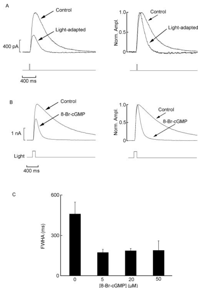
Figure 5. Acceleration of the photocurrent by 8-Br-cGMP resembles light adaptation effects. A , Left, Superimposed flash responses ( 4.95 \times 10^{13} photons \times cm ^{-2} ) in a control photoreceptor stimulated under dark-adapted conditions and subsequently during exposure to sustained background illumination ( 4.2 \times 10^{13} photons \cdot cm ^{-2} \cdot s ^{-1} ). Right, The same two traces were normalized with respect to their peak amplitude (Norm. Ampl.), revealing a pronounced acceleration in response kinetics after light adaptation. B , A similar comparison is made between the dark-adapted responses in one control cell and one dialyzed with 20 \mu\text{M} 8-Br-cGMP. Again, the treatment caused not only a reduction in photocurrent amplitude but also a more rapid time course. C , Flash response speed, measured as the FWHM of the light-evoked current, in control conditions and during perfusion with increasing concentrations of 8-Br-cGMP, in separate groups of cells. Error bars denote SD.
