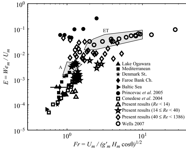
FIGURE 12. Dependence of the entrainment parameter E = We_m / U_m on the Froude number. Solid and open symbols are used for observational and laboratory data, respectively. Shaded areas represent the non-rotating laboratory experiments of Ellison & Turner (1959) (ET) and Alavian (1986) (A).
