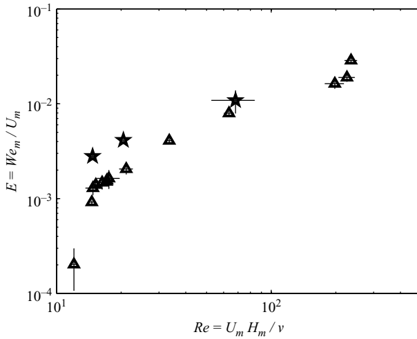
FIGURE 8. Entrainment parameter, E , dependence on the Reynolds number, Re , for experiments lying in two different ranges of the Froude number: 1.3 \leq Fr < 1.5 (triangles), and 2.4 \leq Fr < 2.7 (stars). Error bars are shown for each data point.
