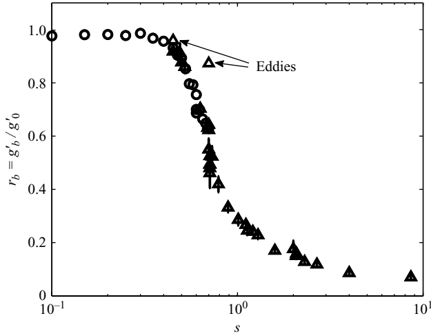
FIGURE 4. Dependence of the mixing ratio measured at the end of the slope, r_b = g'_b / g'_0 , on the slope s for Q = 2.5 \text{ cm}^3 \text{ s}^{-1} , f = 1 \text{ s}^{-1} , and g'_0 = 4 \text{ cm s}^{-2} . Circles represents the results from CWAO and triangles are the present results. The two triangles indicated as “eddies” had Q = 8.3 \text{ cm}^3 \text{ s}^{-1} , f = 1.75 \text{ s}^{-1} and g'_0 = 4 \text{ cm s}^{-2} . Vertical bars indicate the 90% confidence intervals.
