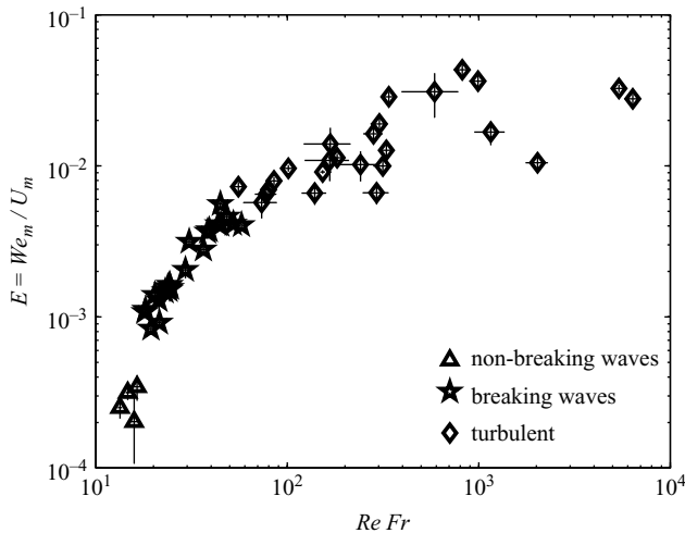
FIGURE 9. Entrainment parameter, E , dependence on both the Froude and Reynolds numbers, ReFr , for the three regimes discussed in the text. Error bars are shown for each data point.
