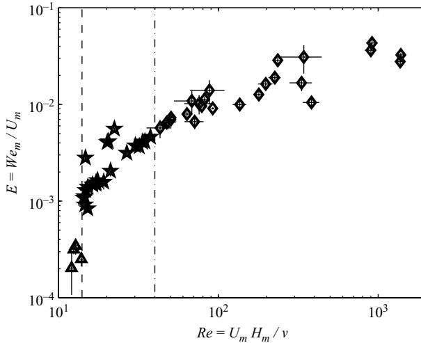
FIGURE 6. Entrainment parameter, E , dependence on the Reynolds number, Re . Triangles represent the non-breaking-waves regime (figure 2a), stars the breaking-waves regime (figure 2b), and diamonds the turbulent regime (figure 3). The dashed line indicates Re = 14 , and the dash-dotted line indicates Re = 40 . Error bars are shown for each data point.
