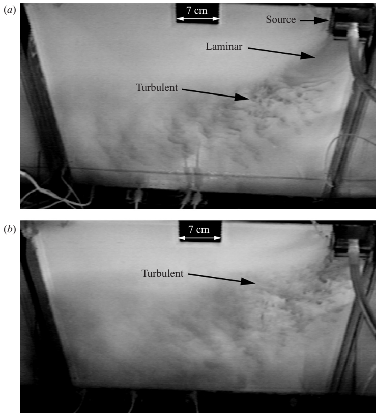
FIGURE 3. Top view of the density current turbulent regime: (a) with a laminar region near the source for Q = 2.5 \text{ cm}^3 \text{ s}^{-1} , f = 1 \text{ s}^{-1} , g'_0 = 4 \text{ cm s}^{-2} , and s = 2 ; and (b) with a turbulent region immediately after the source for Q = 8.3 \text{ cm}^3 \text{ s}^{-1} , f = 1 \text{ s}^{-1} , g'_0 = 9.8 \text{ cm s}^{-2} , and s = 2.1 . The calculated average current thickness is (a) H_m = 0.53 \pm 0.041 \text{ cm} and (b) H_m = 1.28 \pm 0.110 \text{ cm} .
