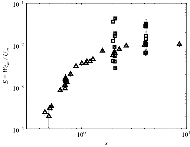
FIGURE 5. Entrainment parameter, E , dependence on the slope angle, s . Triangles represent the experiments shown in figure 4 in which only the slope angle was varied. Squares represent all the other experiments in which the flow rate, the Coriolis parameter, and the initial reduced gravity were also varied. Error bars are shown for each data point.
