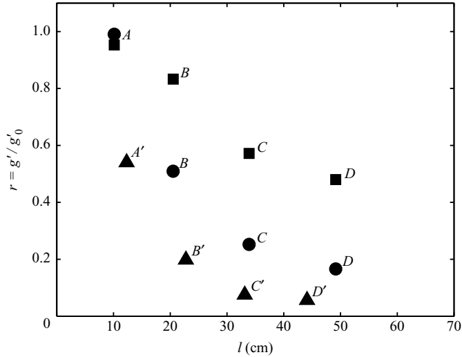
FIGURE 10. Mixing dependence on down-slope distance. Solid triangles: high Reynolds number, Re = 900 ( Fr = 1 , Q = 8.3 \text{ cm}^3 \text{ s}^{-1} , f = 1 \text{ s}^{-1} , g'_0 = 99.8 \text{ cm s}^{-2} , s = 2 ). Solid circles: intermediate Reynolds number, Re = 43.1 ( Fr = 1.7 , Q = 2.5 \text{ cm}^3 \text{ s}^{-1} , f = 1 \text{ s}^{-1} , g'_0 = 4 \text{ cm s}^{-2} , s = 2 ). Solid squares: low Reynolds number, Re = 14.6 ( Fr = 1.5 , Q = 2.5 \text{ cm}^3 \text{ s}^{-1} , f = 1 \text{ s}^{-1} , g'_0 = 4 \text{ cm s}^{-2} , s = 0.7 ).
