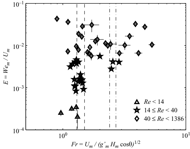
FIGURE 7. Entrainment parameter, E , dependence on the Froude number, Fr , for different ranges of Reynolds number Re characterizing the three regimes discussed in the text. The dashed lines indicate 1.3 \leq Fr < 1.5 , while the dash-dotted lines indicate 2.4 \leq Fr < 2.7 . Error bars are shown for each data point.
