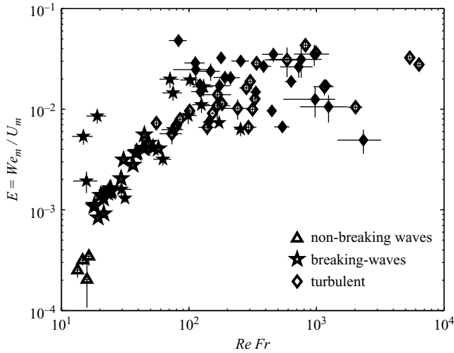
FIGURE 11. Entrainment parameter, E , dependence on both the Froude and Reynolds numbers, ReFr , for the three regimes discussed in the text. Open symbols show the same data as figure 9. Solid symbols show the data collected at three locations on the slope for a selected number of experiments. Error bars are shown for each data point.
