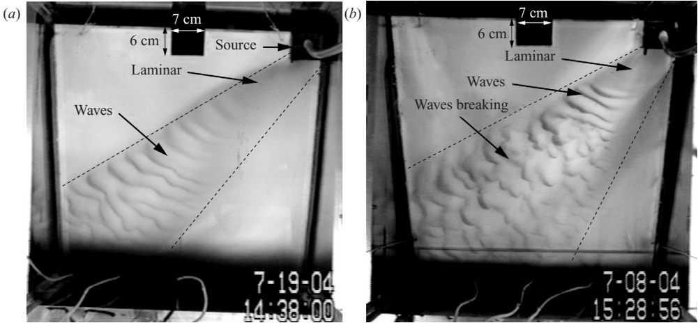
FIGURE 2. Top view of the density current: (a) non-breaking waves regime for Q = 2.5 \text{ cm}^3 \text{ s}^{-1} , f = 1 \text{ s}^{-1} , g'_0 = 4 \text{ cm s}^{-2} , and s = 0.45 ; and (b) breaking-waves regime for Q = 2.5 \text{ cm}^3 \text{ s}^{-1} , f = 1 \text{ s}^{-1} , g'_0 = 4 \text{ cm s}^{-2} , and s = 0.7 . The calculated average current thickness is (a) H_m = 0.18 \pm 0.003 \text{ cm} and (b) H_m = 0.18 \pm 0.009 . The dotted lines indicate the approximate edges of the current.
