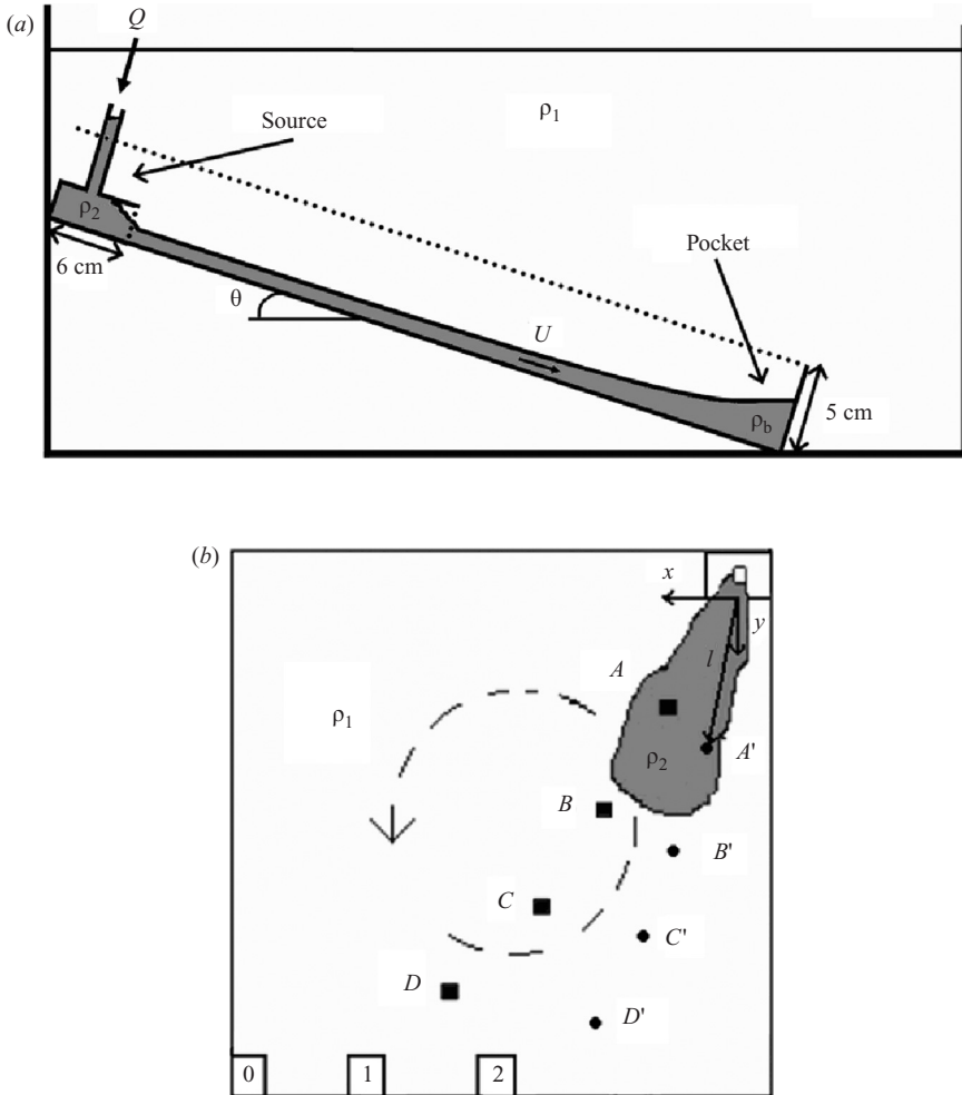
FIGURE 1. Sketch of the experimental apparatus: (a) side view of the rotating tank with the source positioned at the top of the slope, and the pocket positioned at the end of the slope; (b) top view of the slope together with the (x, y) system of reference. The dashed arrow indicates the counterclockwise direction of rotation of the table. Not to scale.
