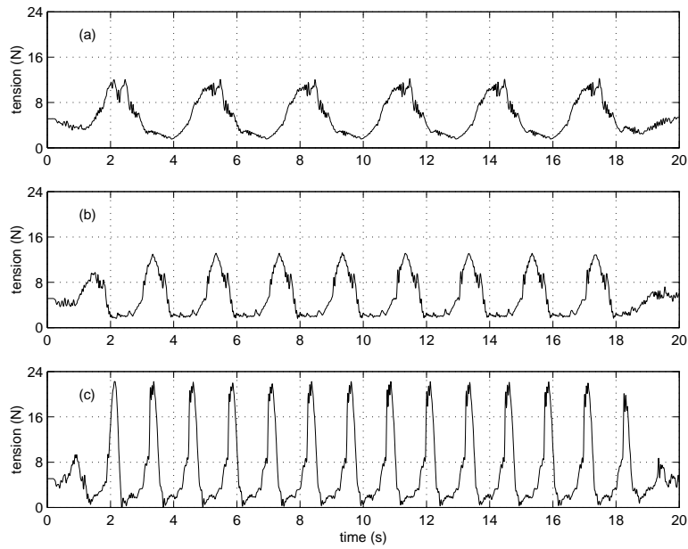
Figure 7-22: Tension time series for the grass bottom at \Delta\tau \approx 0.80 for excitation amplitude 0.25 m and excitation periods (a) 3.0 s, (b) 2.0 s, and (c) 1.25 s.
