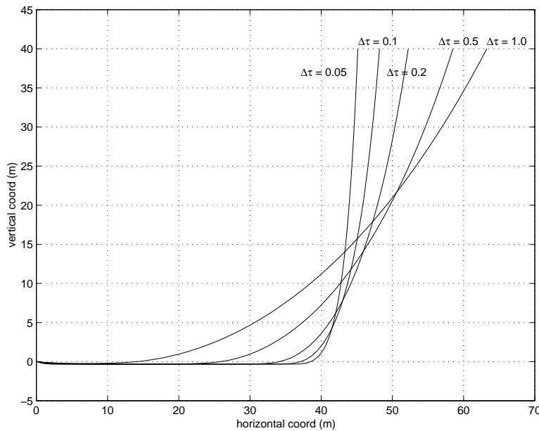
Figure 6-5: Static configurations of the simplified SWEX mooring used in the study to isolate tension mechanisms.
