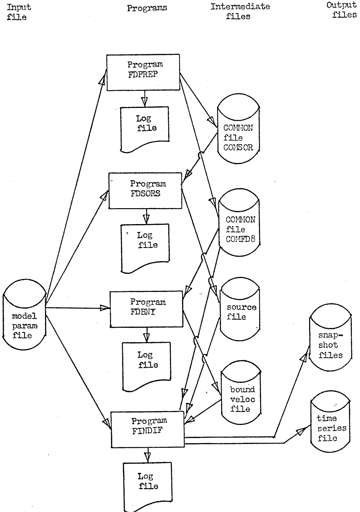
Figure 2 SYSTEM DIAGRAM
