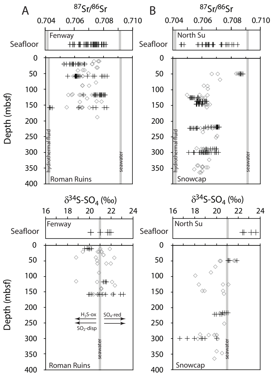
Figure 3.7. Sr isotope ( ^{87}\text{Sr}/^{86}\text{Sr} ) and S isotope ( \delta^{34}\text{S} ) values determined by this study (black crosses) and compared with values determined by Roberts et al. (2003) and Bach et al. (2005) by whole rock analysis (gray diamonds). Concordance between the datasets is good, however the overall range of isotope values is greater for in situ analyses, reflecting the local \sim 1 mm heterogeneity recorded by in situ measurements. A) Fenway (seafloor) and Roman Ruins (drill core), B) Snowcap (drill core) and North Su (seafloor).
