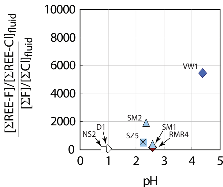
Figure 2.10. Comparison among measured pH (25 °C) and aqueous species distribution of REEs with fluoride and chloride predicted by thermodynamic calculations for selected Manu Basin hydrothermal fluids. Data shown as the ratio of total REE-fluoride and REE-chloride complex as a function of total fluoride and chloride concentration. As pH decreases, the fraction of REE complexed with fluoride decreases, likely resulting from increased association of HF and lower relative availability of fluoride to complex with REE at low pH. For low pH acid-sulfate fluids, there is essentially no REE-fluoride complex formation despite a range of fluoride concentrations in these fluids. In contrast, the fraction of REE-fluoride complex formation increases with pH as HF is increasingly dissociated and free fluoride is present.
