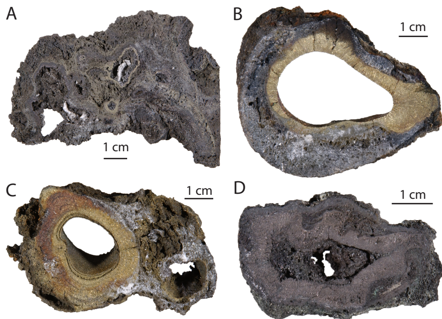
Figure 5.3. Cross sections of chimneys sampled from vent fields in the Manus Basin. A) Relict diffuser-type chimney from Vienna Woods, composed of a fine-grained Zn-sulfide matrix (gray) hosting minor amounts of pyrite and chalcopyrite (yellow) that are locally coarse-grained and form continuous rims around narrow channelways. Amorphous silica is present as a major ( \sim 25 wt% \text{SiO}_2 ), late mineral (sample J2_200_5_R1). B) Open conduit smoker from Roman Ruins (PACMANUS) with a central channel enclosed by an inner monomineralic chalcopyrite layer (yellow) and outer anhydrite-rich layer (light gray) and a thin exterior pyrite-marcasite and Fe-oxide rim (sample J2_213_2_R1). C) Open conduit smoker from North Su (SuSu Knolls) with two chalcopyrite-lined channelways coalesced by a fine-grained anhydrite-chalcopyrite matrix (sample J2_223_1_R1). D) Tennantite-lined (purple-gray) chimney from North Su (SuSu Knolls) with conduit infill of fine-grained tennantite and an outer layer of mixed barite and fine-grained tennantite and pyrite (dark gray) (sample J2_223_13_R1). Scale bar in figures is 1 cm.
