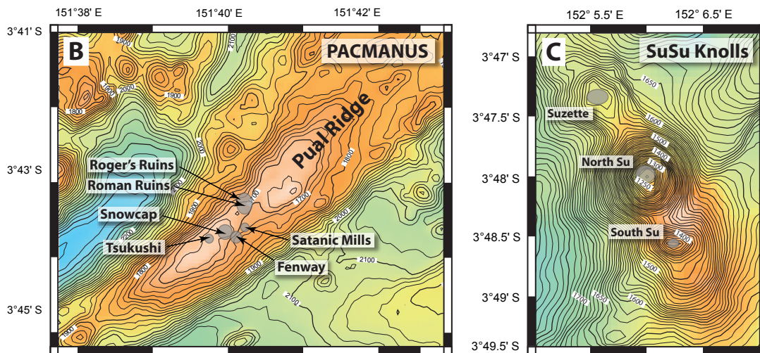
Figure 5.1. A) Regional tectonic setting of the Manus Basin indicating active plate motions and rifting, and areas of known hydrothermal activity in the Manus Basin. B) Distribution of known hydrothermal vent fields at PACMANUS. C) Known hydrothermal vent fields at SuSu Knolls. Bathymetry based on EM300 SeaBeam sonar (modified from Tivey et al., 2007).
