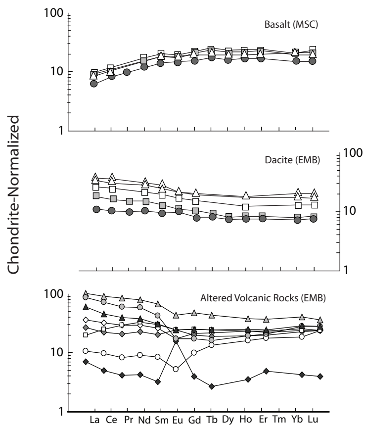
Figure 2.7. Chondrite-normalized REE pattern shapes of unaltered glass erupted at the Manus Spreading Center (basalt) and in the Eastern Manus Basin (dacite-rhyolite) compared to those of altered volcanic rocks in the Eastern Manus Basin. Data for fresh volcanic glasses are from Sinton et al. (2003) and for altered volcanic rocks from Beaudoin et al. (2007).
