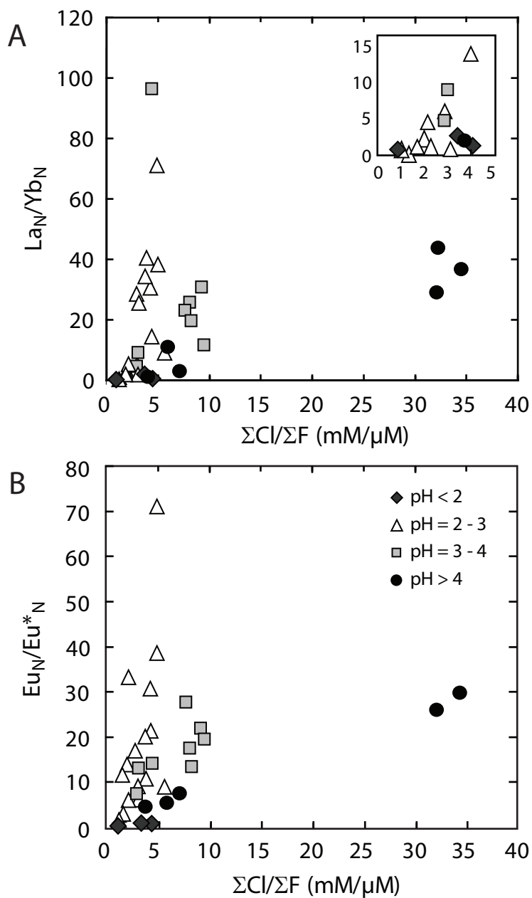
Figure 2.6. Trends between A) chondrite-normalized La/Yb ratios vs. \Sigma Cl/\Sigma F ratios, and B) chondrite-normalized Eu-anomaly ( Eu/Eu^* ) vs. \Sigma Cl/\Sigma F ratios for all vent fluids sampled from the Manus Basin (Vienna Woods, PACMANUS, DESMOS and SuSu Knolls). Note the apparent influence of pH on the observed geochemical trends. See text for discussion.
