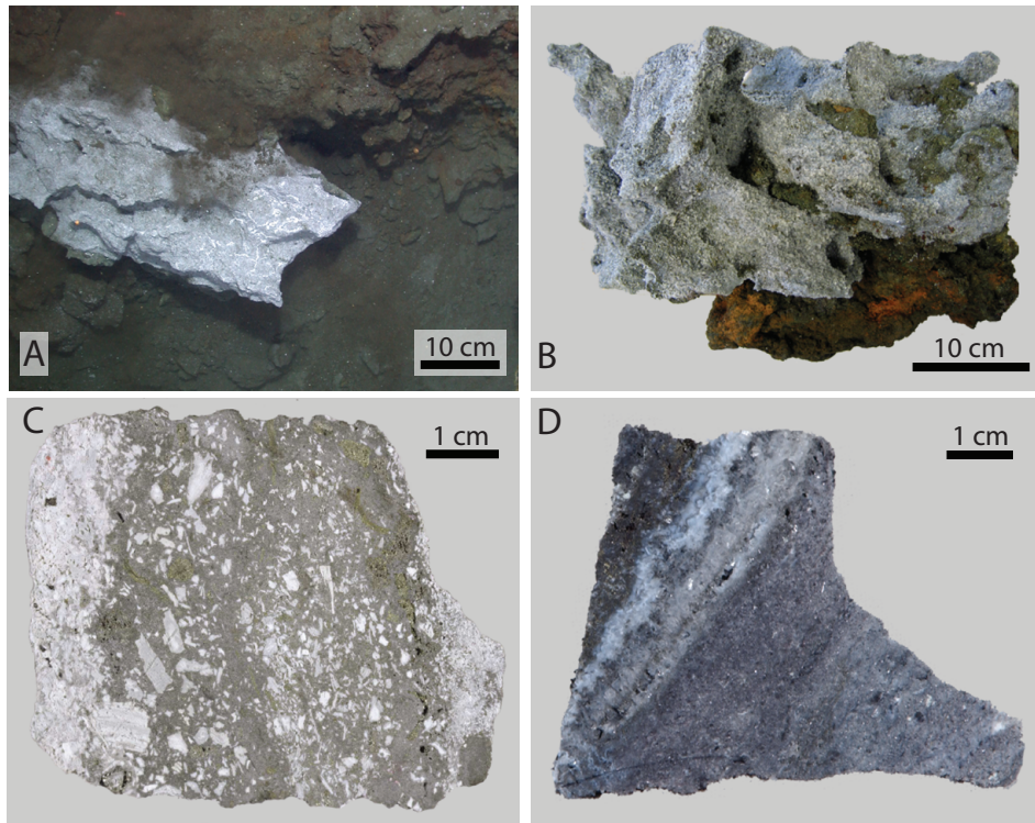
Figure 3.2. Photographs of A) massive anhydrite exposed at the seafloor (Fenway mound, PACMANUS). B) massive anhydrite (sample J2_212_7_R1 from Fenway). C) semi-massive sulfide (chalcopyrite+pyrite) within a matrix of anhydrite+silica (ODP drill core sample 193_1189A_12R_1, 120-128 cm, 105 mbsf, from Roman Ruins, PACMANUS). Photograph modified after Binns et al. (2007). D) cross-section through composite vein of massive anhydrite with frequent fine-to-medium grained chalcopyrite-rich sulfide dissemination (samples sample J2_227_7_R2 from North Su, SuSu Knolls).
