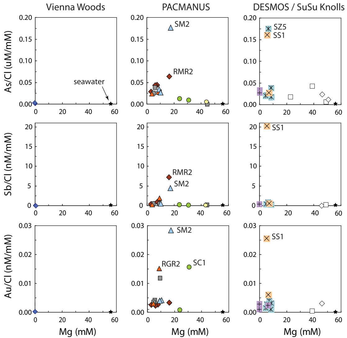
Figure 4.4. (contd) Chloride-normalized concentrations of As, Sb and Au versus Mg for seafloor hydrothermal fluids from Vienna Woods, PACMANUS, DESMOS and SuSu Knolls. Symbols as for Figure 4.3.
