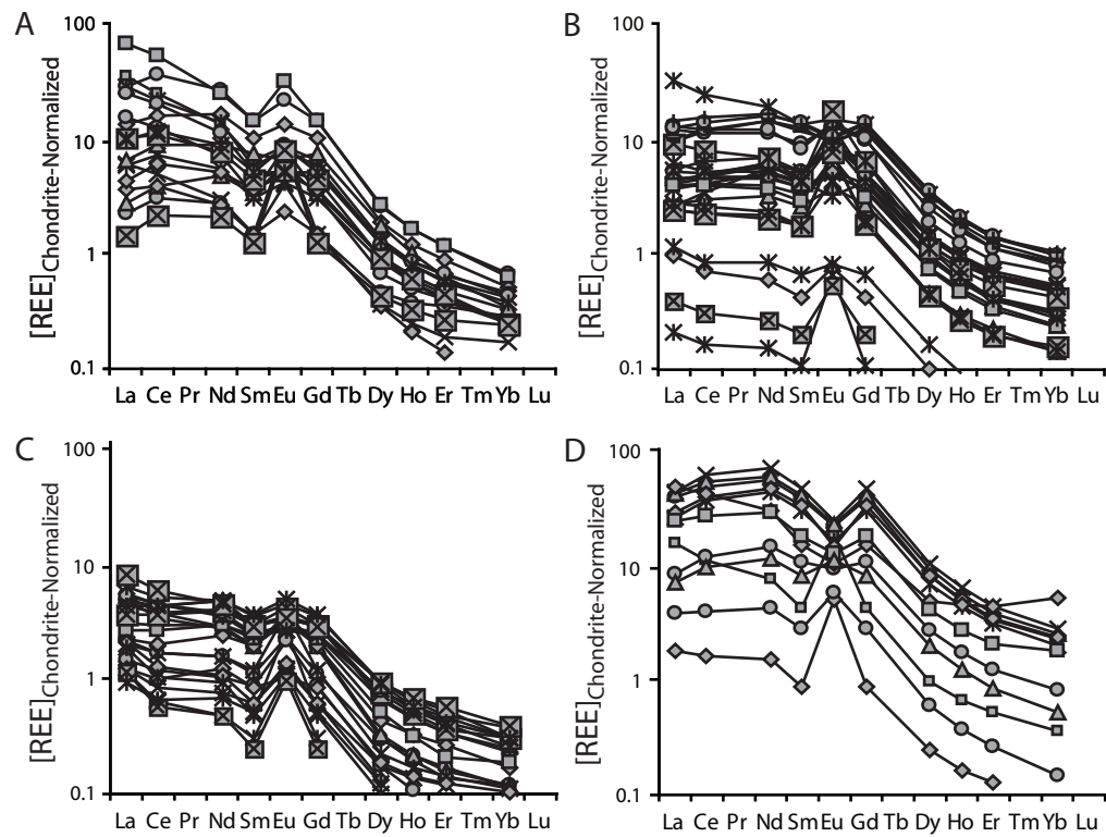
Figure 3.4. Chondrite-normalized REE patterns for anhydrite recovered from site 1189 (Roman Ruins), PACMANUS hydrothermal system. Individual patterns determined in situ by laser ablation ICP-MS. A) sample 193_1189A_3R_1, 89-93cm, 20 mbsf, B) sample 193_1189A_7R_1, 19-23cm, 58 mbsf, C) sample 193_1189B_10R_1, 42-44cm, 118 mbsf, D) sample 193_1189B_14R_2, 0-3cm, 158 mbsf. Chondritic values from Anders and Grevasse (1989).
