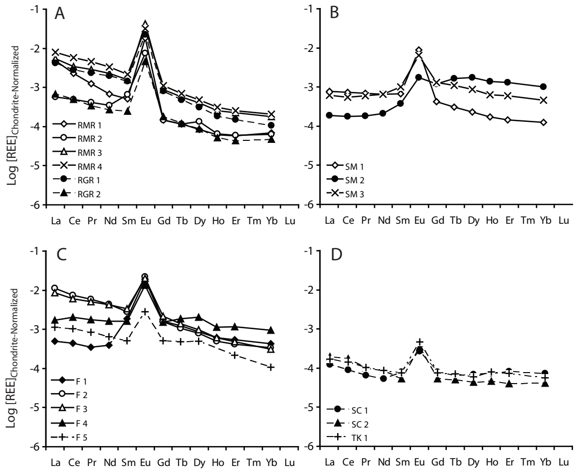
Figure 2.3. Chondrite-normalized REE patterns for high- and low-temperature smoker vent fluids sampled from the PACMANUS hydrothermal area, Eastern Manus Basin: A) Roman Ruins-Roger's Ruins, B) Satanic Mills, C) Fenway and, D) Snowcap and Tsukushi.
