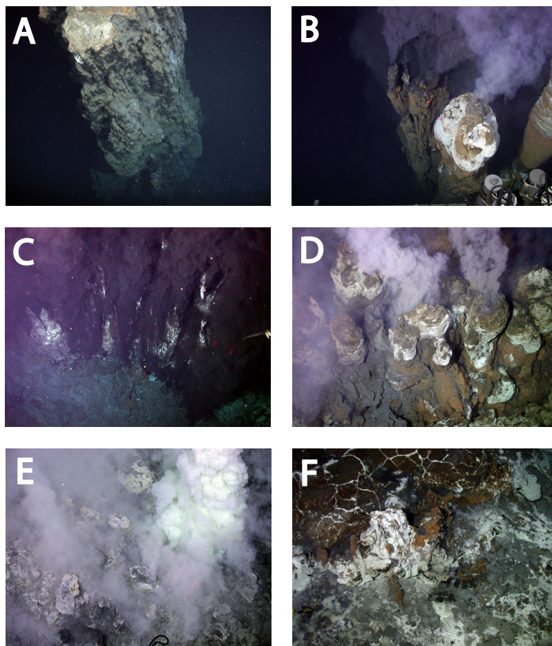
Figure 5.2. Jason II photographs of relict and active vent deposits at hydrothermal vent fields in the Manus Basin. (A) Approximately 5 m tall relict columnar chimney from the Vienna Woods vent field (top of chimney removed by prior sampling). (B) Contrasting venting characteristics of high-temperature black smoker fluids from open conduit chimneys (background) and lower-temperature gray smoker fluids from diffuser-type chimneys (foreground). From top of 3 m tall multi-spined, coalesced chimneys at the Roman Ruins vent field (PACMANUS). (C) Vigorous black smoker discharge from cracks and small open conduit orifices at the base of the black smoker complex at the Fenway vent field (PACMANUS). Field of view ~ 2 m. (D) Lower-temperature venting through multiple diffuser (“beehive”) chimneys at Roman Ruins (PACMANUS). Field of view ~ 2 m. (E) Vigorous milky-white acid-sulfate fluid discharge (pH < 2, at 25 °C) from brecciated and altered rocks at the North Su vent field (SuSu Knolls). Field of view ~ 1.5 m. (F) Oxide-crusting sulfidic pavement (top of frame) on top of brecciated hydrothermal sulfidic sediment at the Suzette vent field (SuSu Knolls).
