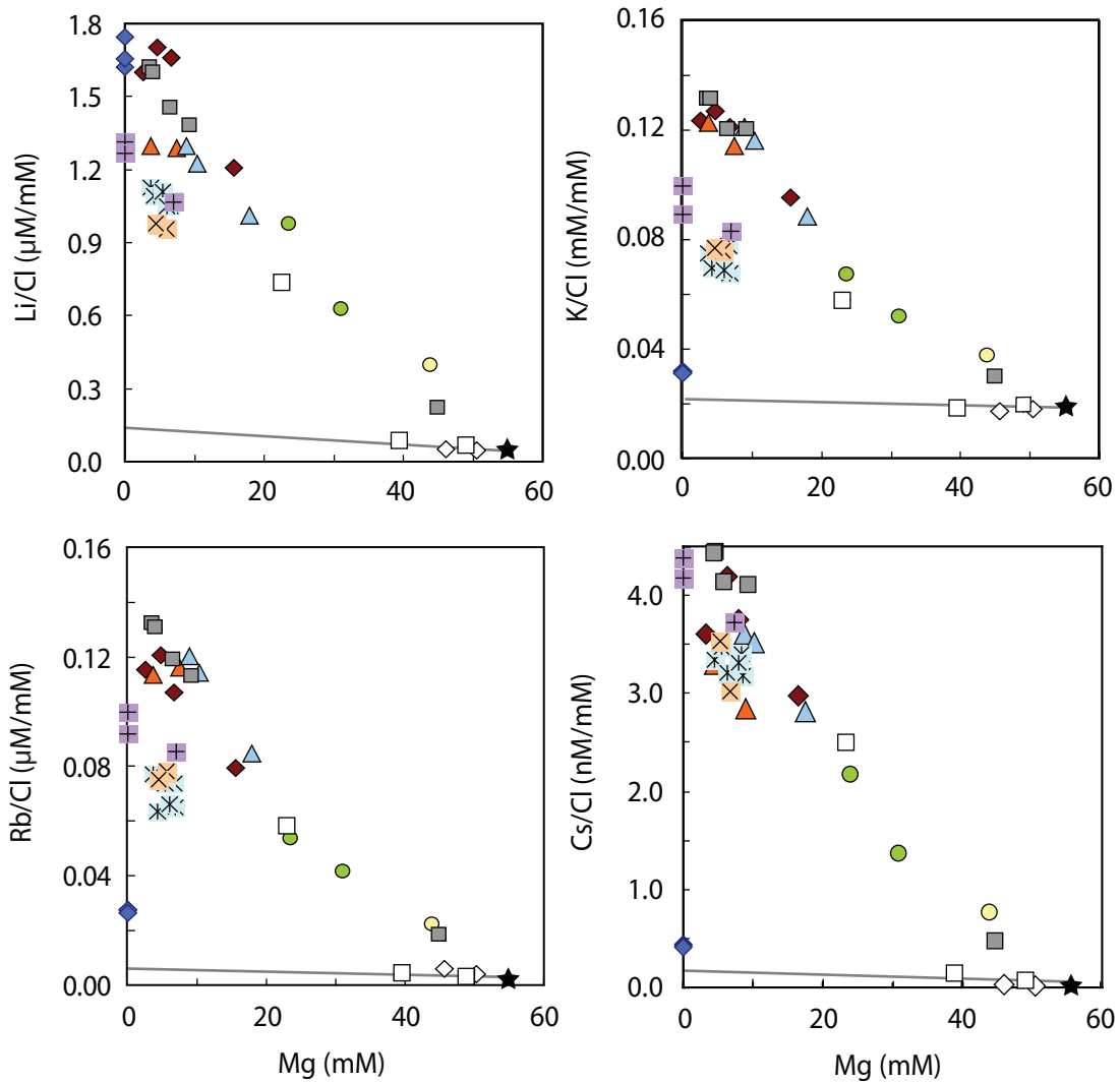
Figure 4.5. Chloride-normalized concentrations of alkali metals Li, K, Rb and Cs versus Mg in hydrothermal fluids from the Vienna Woods, PACMANUS, DESMOS and SuSu Knolls vent fields in the Manus Basin. Symbols as given in Figure 4.3.
