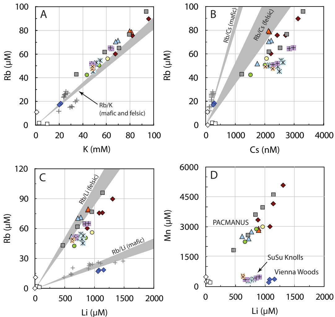
Figure 4.6. Concentrations of A) Rb versus K, B) Rb versus Cs, C) Rb versus Li and D) Mn versus Li in seafloor vent fluids from the Vienna Woods, PACMANUS, DESMOS and SuSu Knolls hydrothermal systems in the Manus Basin. Concentrations of alkali metals in mid-ocean ridge hydrothermal fluids are indicated by gray crosses; data from Palmer and Edmond (1989) and You et al. (1994). The shaded gray areas show the ratios of these elements in basalt erupted in the Manus Spreading Center ("mafic" line) and dacite/rhyolite erupted in the Eastern Manus Basin ("felsic" line); data from Sinton et al. (2003) and D. Niedermeier and W. Bach ( unpubl. data ). Symbols as given in Figure 4.3.
