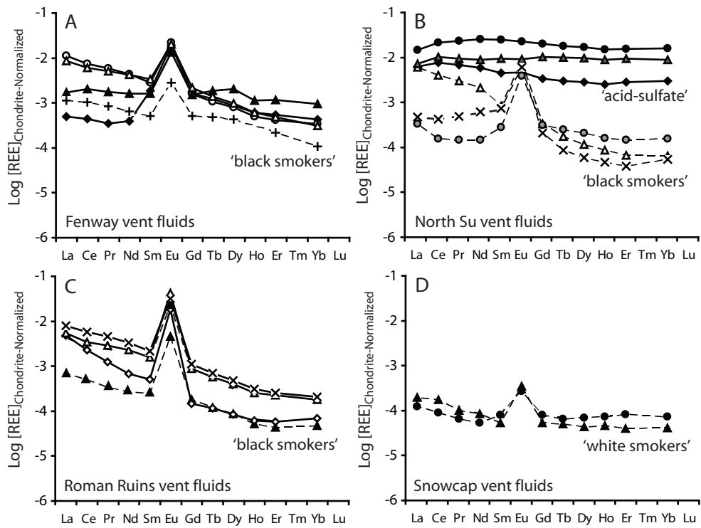
Figure 3.8. Chondrite-normalized REE patterns for seafloor hydrothermal fluids sampled from the Manus Basin. A) black smoker fluids from Fenway, PACMANUS, B) black smoker fluids and acid-sulfate fluids from North Su, SuSu Knolls, C) black smoker fluids from Roman Ruins, PACMANUS, D) white/gray smoker fluids from Snowcap. (Data reported in Chapter 2.)
