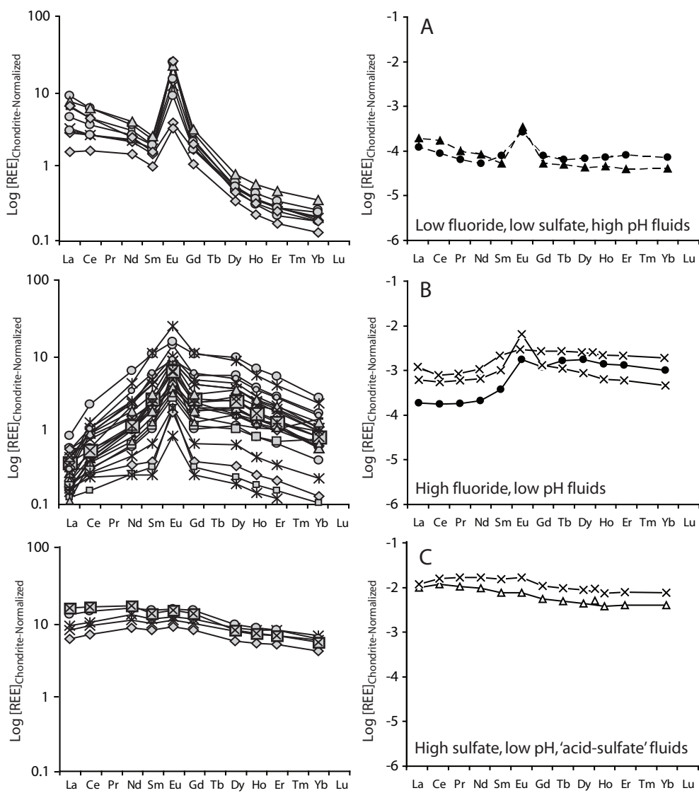
Figure 3.9. Summary of REE N pattern shapes of Snowcap anhydrite samples (left) and comparison with REE N pattern shapes of seafloor vent fluids from hydrothermal systems in the Manus Basin (right) that are variably affected by magmatic volatile degassing. The similarity between REE compositions of Snowcap anhydrites and of vent fluids is evidence for magmatic volatile degassing affecting the compositions of mineral deposits at Snowcap. A) Light-REE enriched patterns of low F and low SO 4 fluids from Snowcap, B) Light-REE depleted, heavy-REE enriched patterns of high F, low pH fluids from Satanic Mills (PACMANUS) and Suzette (SuSu Knolls), C) Flat REE patterns with no Eu-anomaly of magmatic vapor-rich low pH acid-sulfate fluids from DESMOS.
