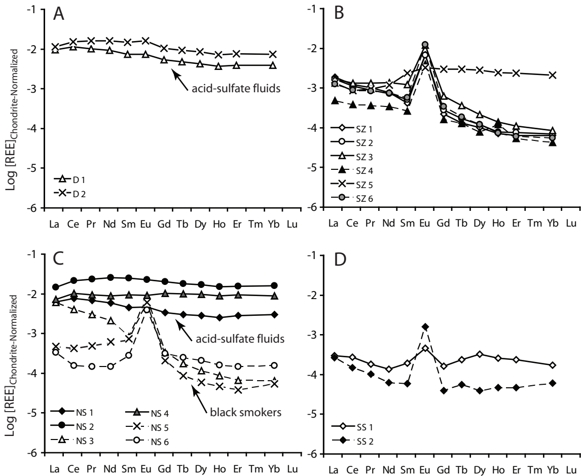
Figure 2.4. Chondrite-normalized REE patterns of fluids sampled from DESMOS and SuSu Knolls hydrothermal areas in the Eastern Manus Basin: A) acid-sulfate fluids from DESMOS, B) smoker fluids from Suzette, C) acid-sulfate (filled symbols) and smoker fluids (open symbols) from North Su, and D) smoker fluids from South Su.
