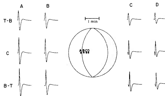
Fig. 11. Theoretical seismograms for models described in Figure 10. The dip of the fault is 55^\circ . Also shown is the theoretical fault plane solution; points A, B, C, and D represent projections of ray paths for which seismograms were calculated. T-B, C, and B-T signify rupture propagation radiating from top-to-bottom, from the center, and from bottom-to-top, respectively.
