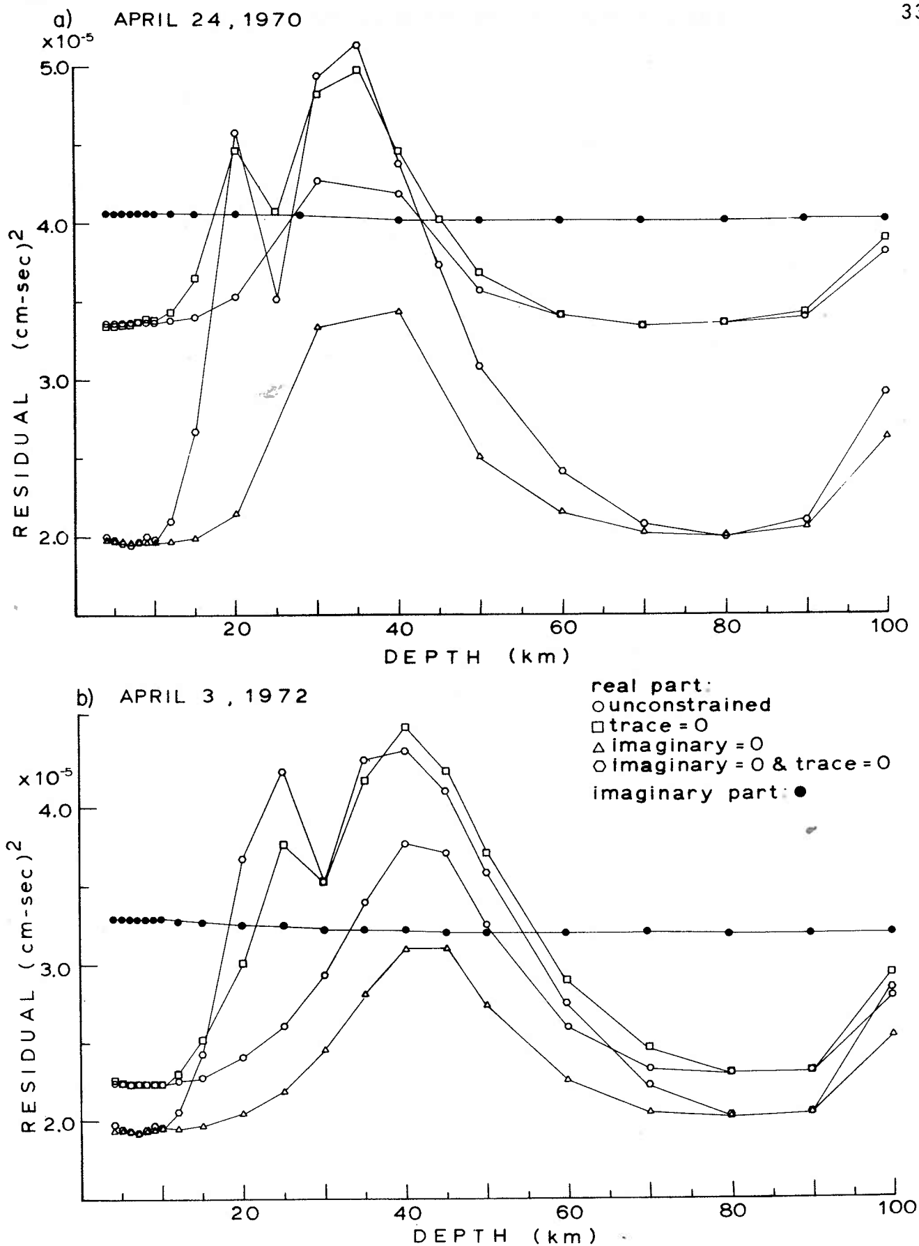
Fig. 6. (a) Residuals versus focal depth for the inversion of the Rayleigh wave radiation pattern to obtain the moment tensor for the April 24, 1970, event. (b) Residuals versus focal depth for the April 3, 1972, event.
