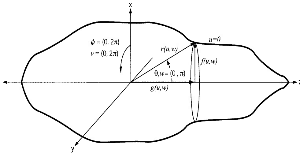
Figure 2-1: Scattering geometry for an irregular, axisymmetric finite-length body. The body is symmetric about the z -axis. The azimuthal angular coordinates, \phi and \nu , range from 0 to 2\pi in the xy -plane, and the polar angular coordinates, \theta and w , range from 0 to \pi , measured from the z -axis. The radial coordinate in the (u, w, \nu) coordinate system equals zero on the surface. Broadside incidence corresponds to \theta=90 degrees. End-on incidence corresponds to 0 and 180 degrees. In the new coordinate system, g(u, w) is the length along the z -axis, and f(u, w) is the projection in the xy -plane.
