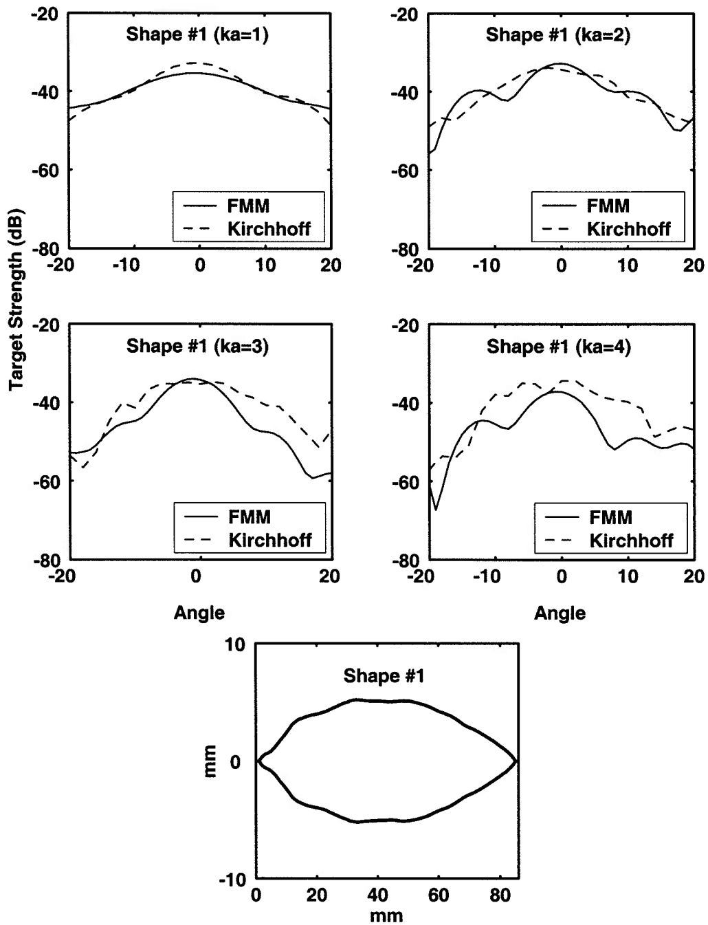
Figure 2-11: FMM and Kirchhoff Approximation: Target Strength as a function of angle for irregular Shape #1 at ka = 1 , ka = 2 , ka = 3 and ka = 4 . Kirchhoff approximation results are based on the formulation from Clay and Horne (1994). Shape #1 is shown in the bottom frame. The vertical axis is exaggerated to better illustrate the irregularity of the surface. Broadside corresponds to 0 degrees.
