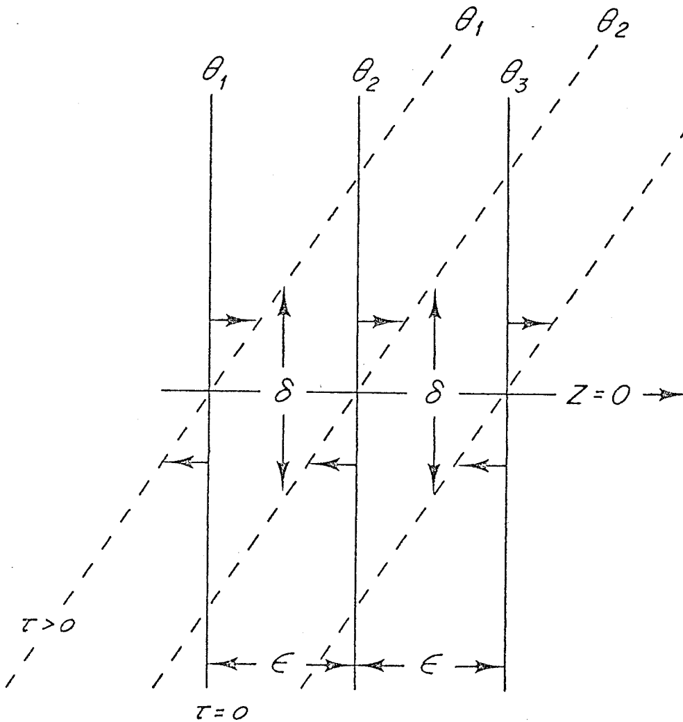
Figure 25. Illustration of the geometry referred to in the text to derive (21.8). Initially the three \theta contours are vertical and equally spaced by a distance \epsilon . The shear flows tips them as shown above.
