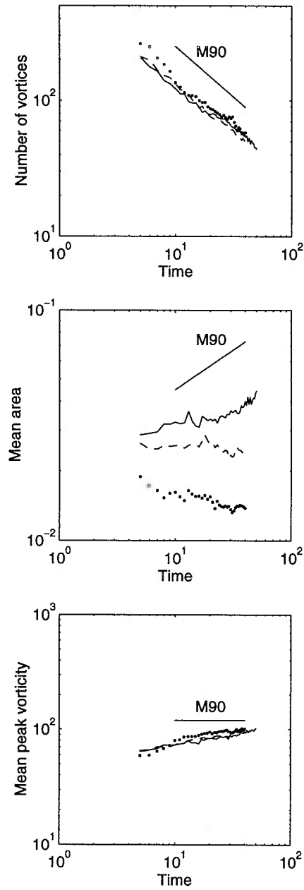
Figure 4.10: Vortex statistics for weak slope cases. Shown are runs with \beta_2 = 0 or \Lambda = \infty (solid), \Lambda = 4 (dots), and \Lambda = 16 (dashed). Vortices are connected regions with q_1 > 10 .
