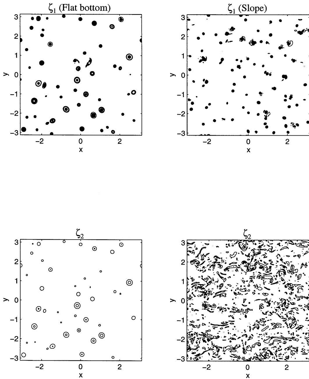
Figure 4.11: The relative vorticity fields at t = 20 for the flat-bottom (left) and the slope (right) cases. The contour values are \pm[10 : 10 : 100] .
