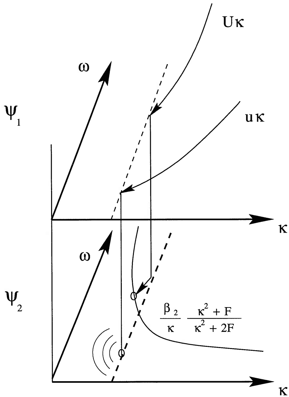
Figure 4.25: The arrest to topographic waves from small scale initial flow. Again the dashed line indicates the deformation wavenumber and layer depths are assumed equal.
