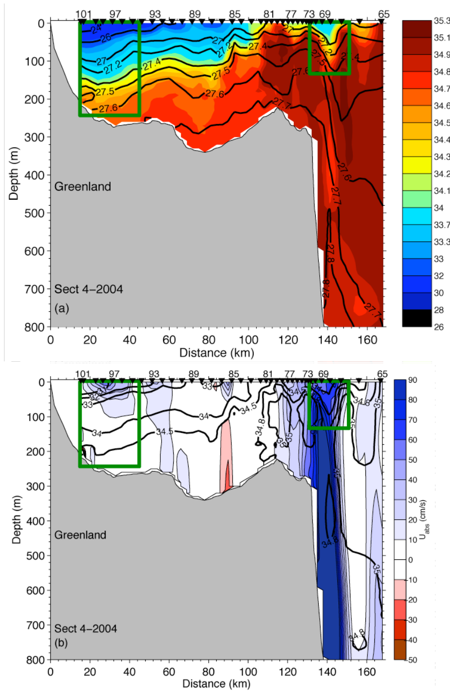
Figure 2.6. Same as Fig. 2.3, except for 2004 JR105 section 4, which is near 66°N.
