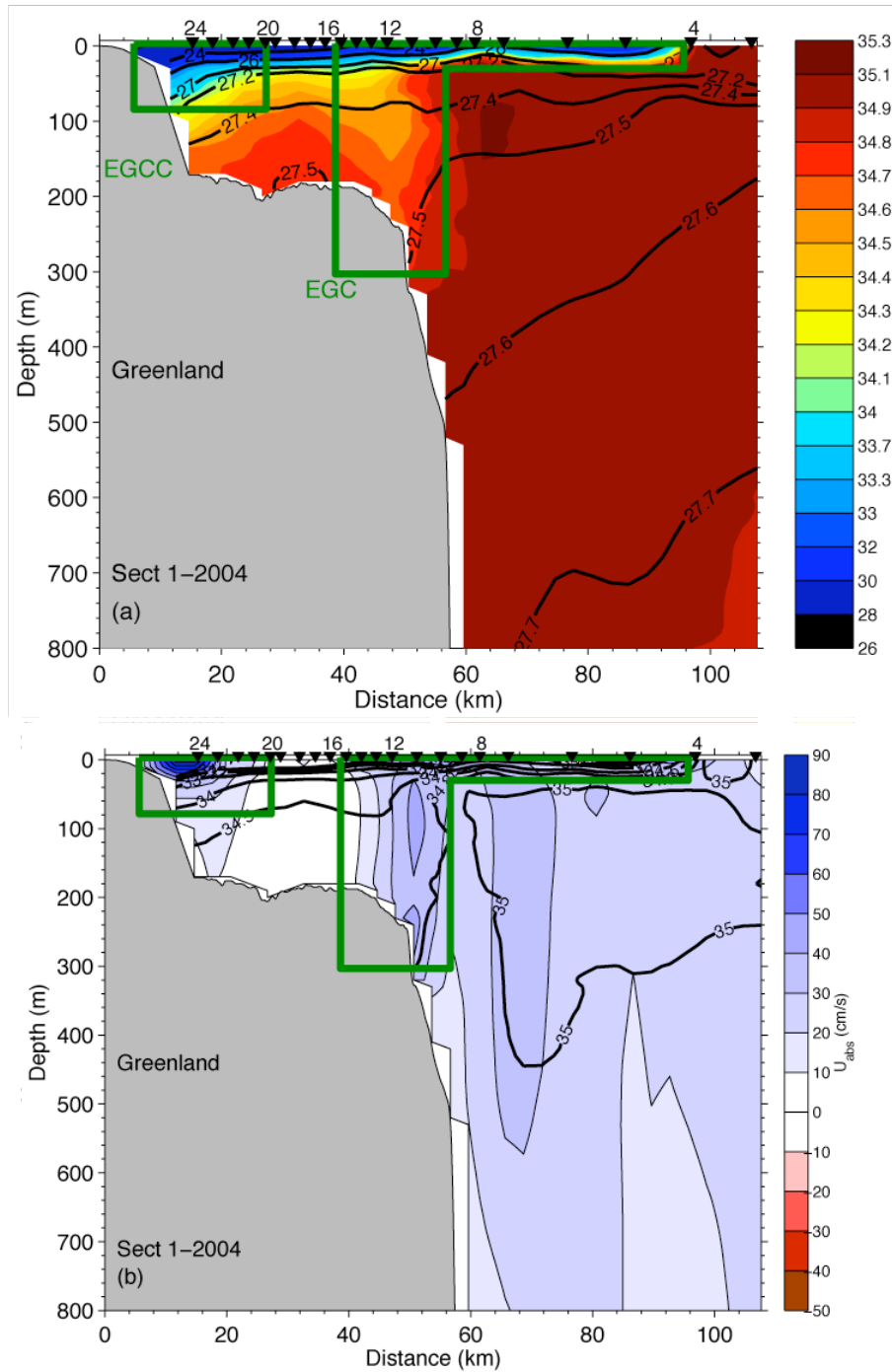
Figure 2.3. (a) Salinity field (color) from 2004 JR105 section 1 near Cape Farewell ( 60^\circ\text{N} ) with select isopycnals ( \text{kg m}^{-3} ) contoured in black. Boxes outline the boundaries defined in the text for the EGCC and the EGC. Black inverted triangles mark the numbered CTD stations. (b) Alongstream absolute velocity, U_{abs} (color, \text{cm s}^{-1} ), for 2004 JR105 section 1 where U_a > 0 denotes equatorward flow. The isohalines (34, 34.5, 34.8, and 35) used in defining the currents are contoured in black.
