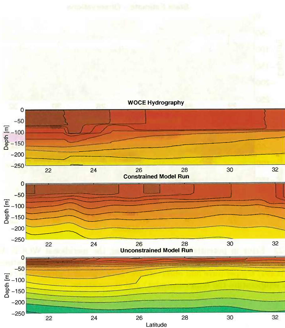
Figure 3-22: Meridional sections of potential temperature along the WOCE AR11 line ( 33^{\circ}W ) in November, 1992. Top panel: Observations from WOCE (courtesy of T. Joyce). Middle panel: Constrained model estimate. Lower panel: Unconstrained model simulation.
