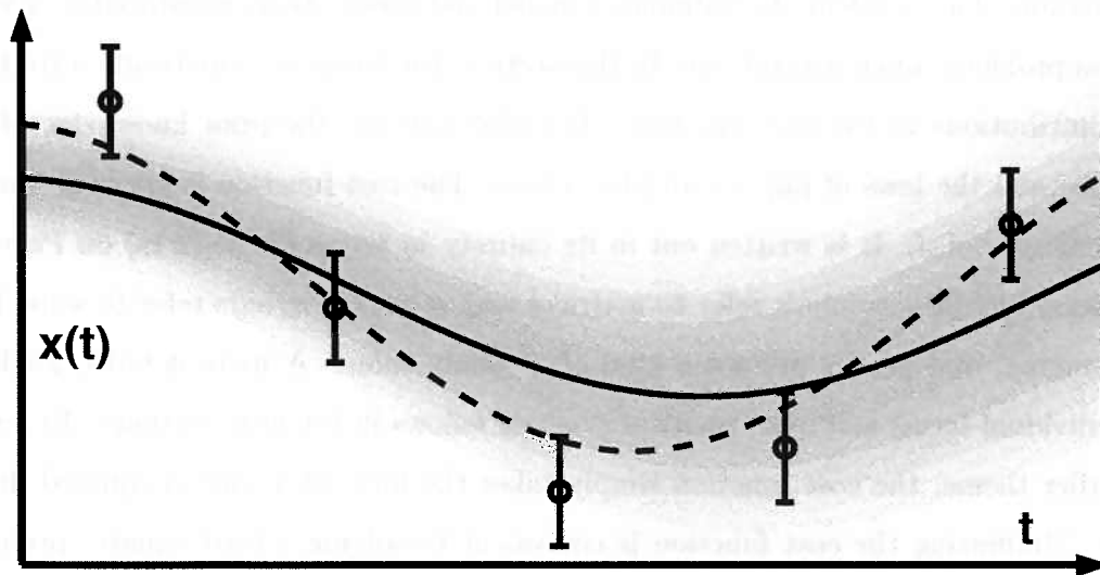
Figure 2-1: Schematic of state estimation. The goal is to find a model trajectory that is within observational uncertainty ( O's with error bars ). The model trajectory is also subject to uncertainty due to model error and uncertain model parameters ( shown as a gray probability distribution cloud ). Here, the first-guess model simulation ( solid black line ) is not within the observational uncertainty at all times. However, there is a model trajectory ( dashed line ) that is consistent with both the observational and model uncertainty. This improved model trajectory is the state estimate.
