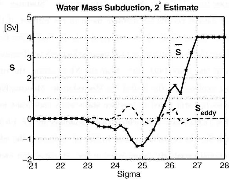
Figure 4-20: Water-mass subduction rate, \bar{S}(\sigma) ( solid line ), and eddy subduction rate, S_{eddy}(\sigma) ( dashed line ), for the 2 degree state estimate. The “X”s mark the density resolution of the diagnostics. The subduction rate is computed about a time-variable mixed-layer base. As the 2° state estimate has little eddy variability, S_{eddy}(\sigma) represents an estimate of the error of the diagnostic scheme.
