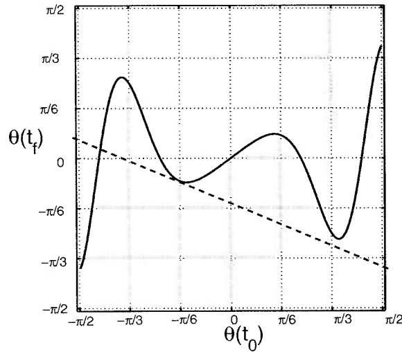
Figure 3-8: Pendulum angle at time t_f = 50 s as a function of initial angle. The function is computed by the nonlinear dynamics ( solid line ), and by the tangent linear model about the trajectory with initial angle, \theta(t_0) = -\pi/6 ( dashed line ).
