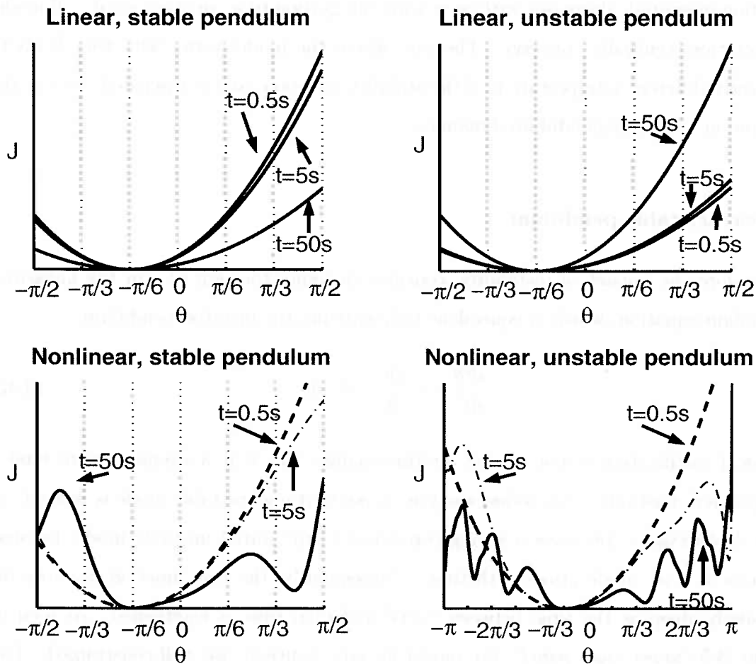
Figure 3-5: Cost function with respect to the initial pendulum angle. A synthetic observation was made from a model run with initial angle, \theta = -\pi/6 . The time between the initial state and the cost function evaluation is 0.5, 5, or 50 seconds. Upper left: Linear, stable pendulum. Upper right: Linear, unstable pendulum. Lower left: Nonlinear, stable pendulum. Lower right: Nonlinear, unstable pendulum. Notice the wider scale for \theta in the lower, right panel. The pendulum's dynamical regimes are further explained in the text.
