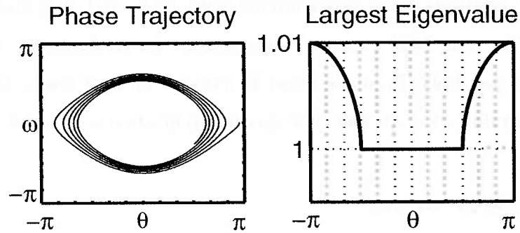
Figure 3-6: Characteristics of the nonlinear pendulum. Left: The nonlinear pendulum traces a damped quasi-periodic orbit in phase space. The pendulum was implemented with a timestep of 0.01\text{ s} and a damping coefficient of 0.01\text{ s}^{-1} . Right: The pendulum is unstable in the upper half plane where the magnitude of the greatest eigenvalue, |\lambda| , exceeds one. In the lower half plane, the pendulum is stable (nearly neutral) with the largest eigenvalue just less than one.
