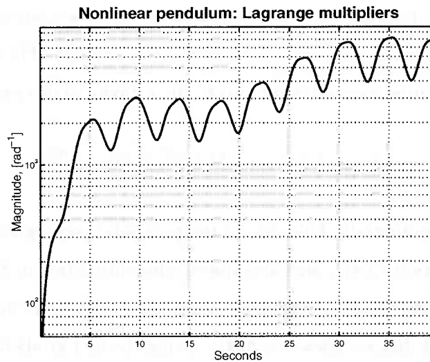
Figure 3-18: The evolution of the Lagrange multipliers of the nonlinear pendulum with reversed time. Here, the maximum Lagrange multiplier, \|\mu(t)\|_{\infty} , is plotted. The time evolution is not as steady as the GCM because no spatial averaging is possible with the nonlinear pendulum.
