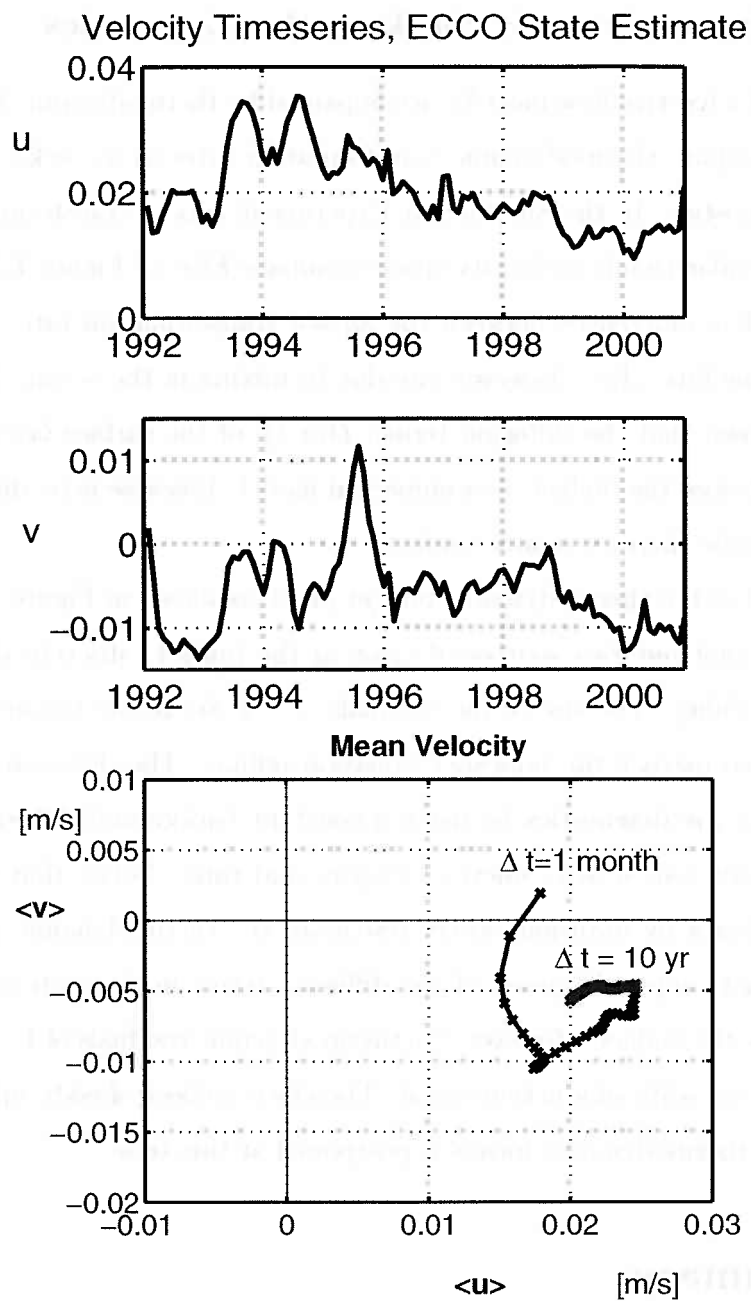
Figure 4-21: Characteristics of the ECCO 1^\circ state estimate velocity timeseries at ( 35^\circ N, 30^\circ W ). Top two panels: Time series of zonal and meridional velocity at 222 meters depth. Bottom panel: Mean velocity as a function of averaging interval, starting from one month and extending to the average of the entire timeseries, 10 years. These plots show that interannual variability is a dominant component of the time series, and stable means are only obtained after long averaging periods.
