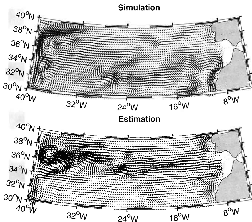
Figure 4-6: Velocity snapshot in the Azores Current subregion. Without any data constraint, the model simulation ( upper panel ) has an Azores Current that meanders south-eastward. The state estimate ( lower panel ) shows a tight, zonal current in accordance with the observations of 1991-93. The maximum velocity vector is 10 cm/s .
