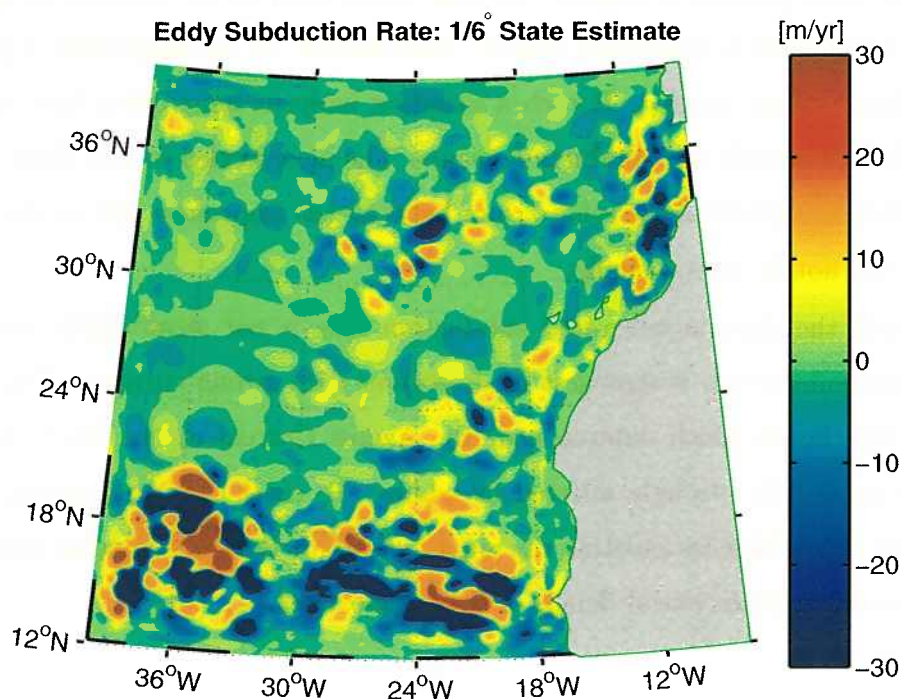
Figure 4-14: Eddy subduction rate, computed as the eddy-thickness flux across the time-variable mixed-layer base. Note the color scale ranges from -30 m/yr to 30 m/yr , a smaller range than Figure 4-12. Eddy subduction is largest in regions with enhanced eddy kinetic energy.
