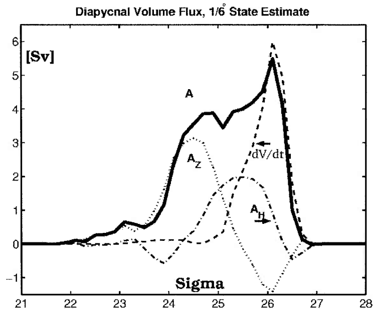
Figure 4-18: Diapycnal volume fluxes in the surface layer. All overbars have been dropped in the figure. Together, \overline{A}_H(\sigma) and \overline{A}_Z(\sigma) represent the Eulerian component of volume flux through the horizontal and vertical velocity fields. \overline{\partial V(\sigma)/\partial t} represents storage in an isopycnal which results from the net displacement of a density surface.
