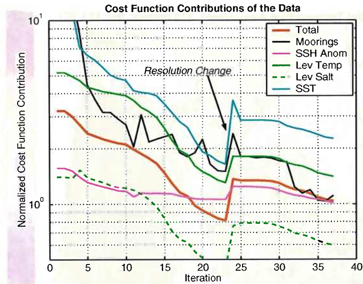
Figure 3-19: Normalized model-data misfit as a function of iteration of the search method for the coarse and eddy-resolving optimization. A value of 1 ( 10^0 ) is expected.
