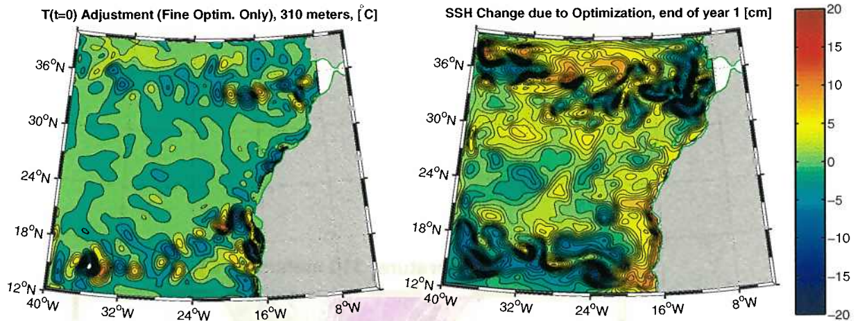
Figure 3-25: Left : Initial temperature adjustment from the optimization of the small-scale observational signal. Right : Rearrangement of the sea surface height field after one year by the initial temperature adjustment.
