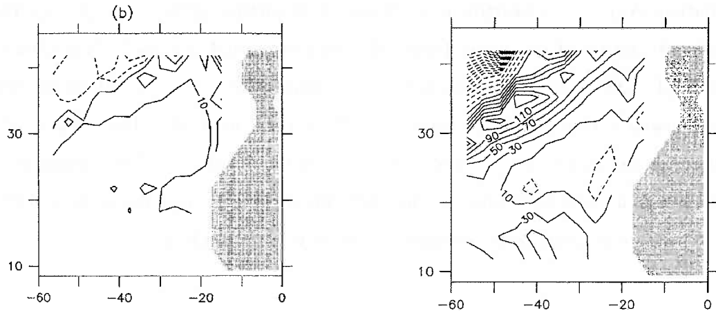
Figure 1-5: Left panel: Thermodynamic estimate of eddy-driven subduction [m/yr] by the diapycnal bolus transport of heat in the mixed layer. Right panel: Estimate of subduction by the mean flow [m/yr]. Both calculations were from a coarse-resolution numerical model with an eddy-parameterization scheme. From Spall et al. (2000).
