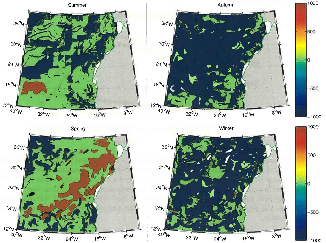
Figure 4-10: The seasonal cycle of detrainment from the mixed layer. The seasonal cycle proceeds clockwise. Blue areas represent large values of entrainment, w_* < -1000 \text{ m/yr} . Dark red areas represent large values of detrainment, w_* > 1000 \text{ m/yr} , and are potential sites of subduction. Green areas include all intermediate values of entrainment velocity. As the entrainment velocities are dominated by local values of \partial h/\partial t , the patterns are not associated with any frontal structures.
