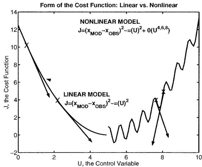
Figure 3-3: Schematic of the cost function with a linear versus nonlinear model. The linear model ( left ) gives a cost function with paraboloidal shape because of the least-squares formulation. A nonlinear model ( right ) potentially gives a much more complicated shape; discontinuities and multiple local minima are possible.
