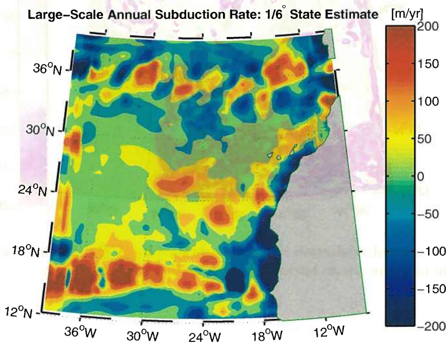
Figure 4-13: Large-scale, annual subduction rate s_{lrgscl} = -(\overline{w}_{H^*} + \overline{\mathbf{u}}_{H^*} \cdot \nabla H^*) , where a star indicates a field that has been coarse-grained. The domain-integrated subduction rate is not significantly altered by the coarse-graining.
