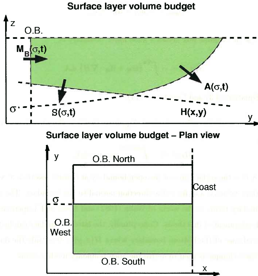
Figure 4-1: The shaded fluid is bounded by an isopycnal, the maximum mixed-layer depth, H(x, y) , the sea surface, and the regional boundary. These surfaces have areas \mathcal{A}_\sigma(\sigma, t) , \mathcal{A}_{th}(\sigma, t) , \mathcal{A}_S(\sigma, t) , and \mathcal{A}_B(\sigma, t) . The diapycnal volume flux through the isopycnal \sigma is A(\sigma, t) , the volume flux across H(x, y) into the interior of the ocean is S(\sigma, t) , and the open boundary volume flux is M_B(\sigma, t) .
