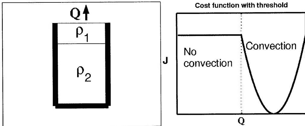
Figure 3-10: Left panel: Schematic of an oceanic water column with upper density, \rho_1 , and abyssal density, \rho_2 . Cooling, Q , is applied to the surface. Right panel: Data-model misfit as a function of cooling. Two dynamical regimes are present: a non-convective regime ( left half ), and a convective regime ( right half ), which greatly affect the cost function form.
