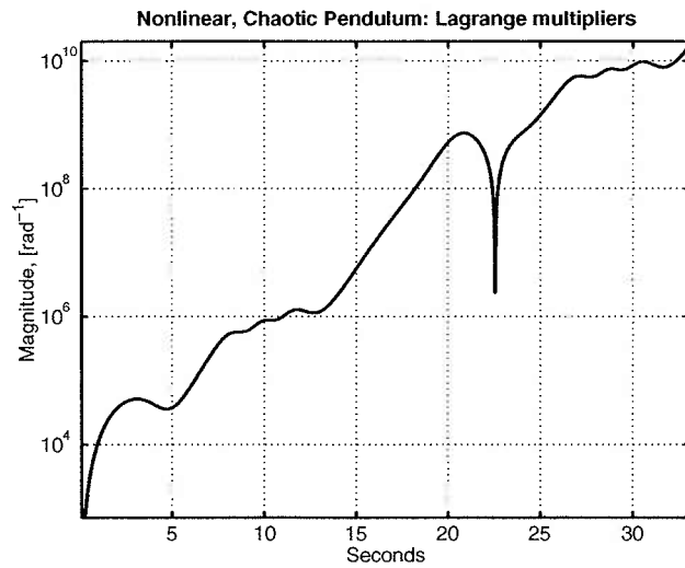
Figure C-2: The evolution of the Lagrange multipliers of the nonlinear, chaotic pendulum ( g = 1.15 ) with reversed time. The maximum Lagrange multiplier, \|\mu(t)\|_\infty , increases exponentially. Compare to Figure 3-18.
