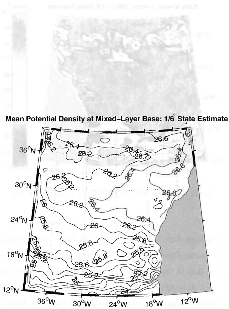
Figure 4-5: Mean potential density at the maximum mixed-layer depth. The spatial density structure serves as a new basis function to examine and understand subduction.
