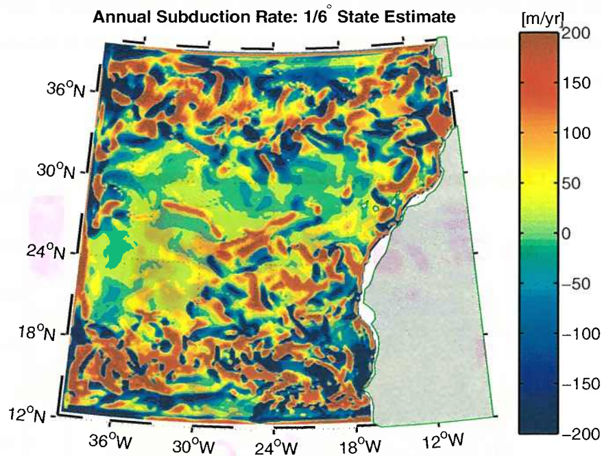
Figure 4-12: Annual subduction rate, s_{ann} = -(\bar{w}_H + \bar{u}_H \cdot \nabla H) . The small-scale, intense subduction rates are due to lateral induction by the mean circulation.
