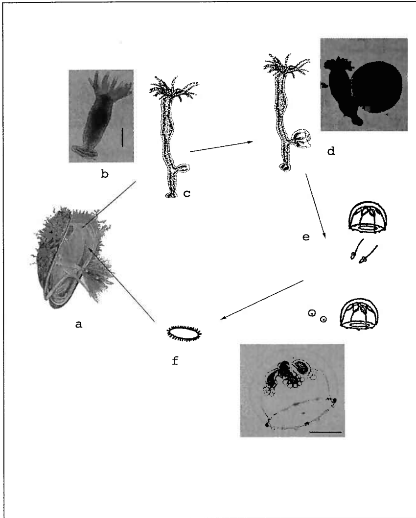
Figure 1. Life cycle of Eugymnanthea . Hydroids (a,b) inhabit bivalves, such as Mytilus galloprovincialis , and asexually produce medusoids (c,d). The medusoids, which are usually separate sexes, are released from the hydroid and produce gametes (e). The gametes fertilize and form planula larvae (f), which settle in a bivalve host (a) and become hydroids. Scale bars: polyp, 250 \mu\text{m} ; medusa, 500 \mu\text{m} .
