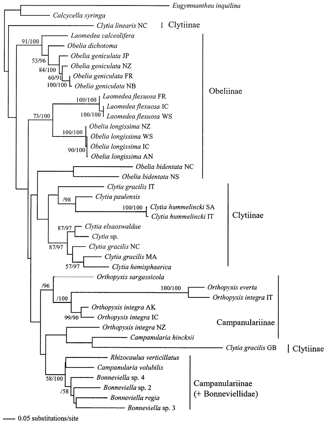
Figure 7. Maximum likelihood topology based on COI sequences alone. The best-fit model selected by Modeltest was GTR + I + G. The -\ln likelihood of the topology = 6877.61370. Numbers before the slash refer to parsimony bootstrap values and numbers after the slash refer to Bayesian posterior probabilities. Subfamily lineages are indicated. Location codes are as in Figure 2.
