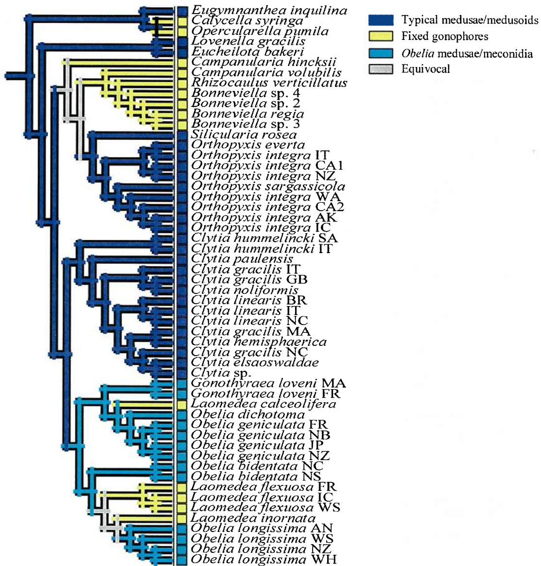
Figure 17. Ancestral state reconstruction on the modified maximum likelihood topology. Obelia bidentata is placed as the basal member of the Laomedea flexuosa , Laomedea inornata , and Obelia longissima clade. Life cycles are placed in 3 categories. Gains = losses = 1.0.
