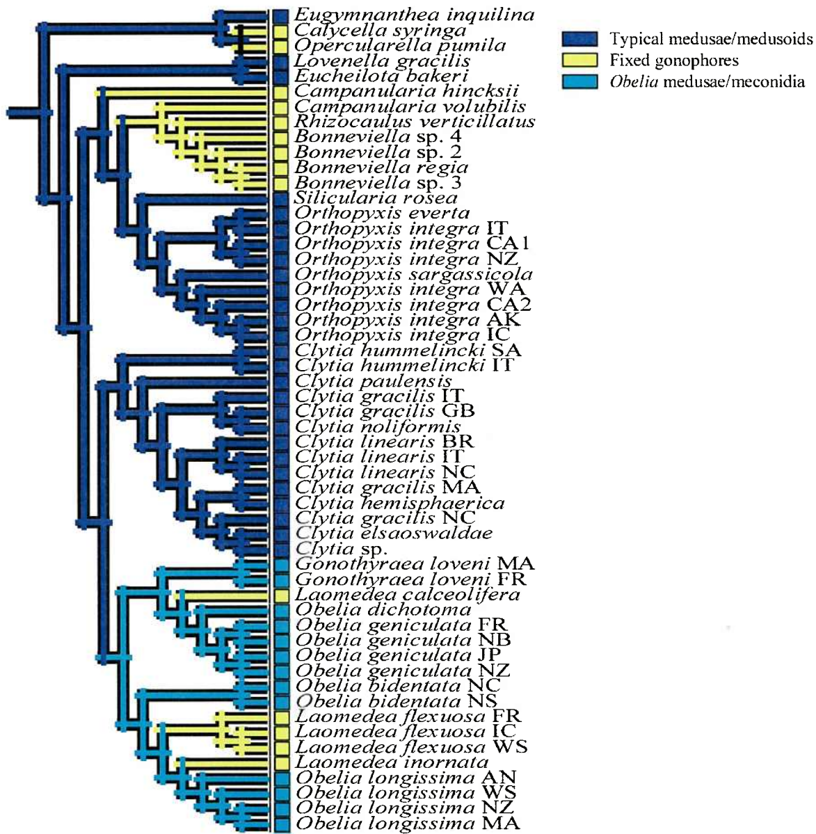
Figure 18. Ancestral state reconstruction on the modified maximum likelihood topology. Obelia bidentata is placed as the basal member of the Laomedea flexuosa , Laomedea inornata , and Obelia longissima clade. Life cycles are placed in 3 categories. Gains \geq 1.1. Losses = 1.0.
