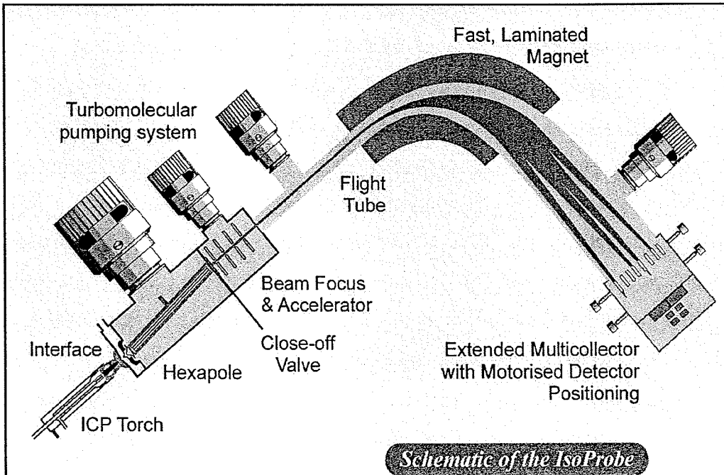
Figure 4.1: Schematic of the GV Instruments IsoProbe MC-ICPMS.
