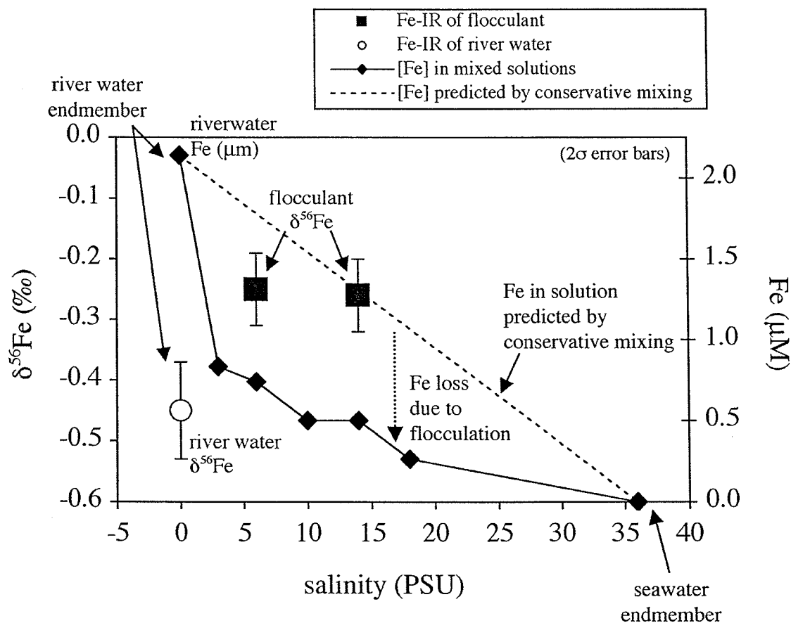
Figure 6.4: River water-seawater mixing experiment. The Fe (◆) concentration of the river water-seawater solutions after the flocculant was removed by filtration are shown with the solid line. The dashed line is the Fe concentration predicted if the river water and seawater were to mix conservatively. The Fe loss due to colloidal coagulation and flocculation is represented by the difference between the two lines. The river water \delta^{56}\text{Fe} (○) is shown for reference, -0.45 \pm 0.08\text{‰} ( 2\sigma , n=8 ). Specifically the sample of river water used for this experiment was Solimoes River sample 3, which had slightly higher dissolved Fe ( 2.1 \mu\text{M} ) compared with the other samples ( <1 \mu\text{M} ). This could be due to particle leak through during filtration or the variability of Fe that passes through a 0.4 \mu\text{m} filter in a river with high suspended load ( 226 \text{ mg/L} ). Despite the difference in concentration, the isotopic composition of the different Solimoes River samples were the similar. The flocculant (■) in this experiment was isotopically heavier than the river water Fe from which it was derived (6 PSU expt: -0.26 \pm 0.06\text{‰} ( 2\sigma , n=2 ); 14 PSU expt: -0.27 \pm 0.06\text{‰} ( 2\sigma , n=2 )). This implies that the remaining dissolved Fe must be isotopically light ( -0.9 to -1.1\text{‰} ) compared to the river water endmember. The Fe contribution from seawater is likely negligible in this experiment. The dissolved Fe in seawater endmember was 0.37 \text{ nM} ( <0.03\% contribution to the total Fe in the experiment), and would have to be > +70 \text{‰} to be responsible for the observed isotopic shift. Error bars are 2\sigma standard errors of replicate measurements.
