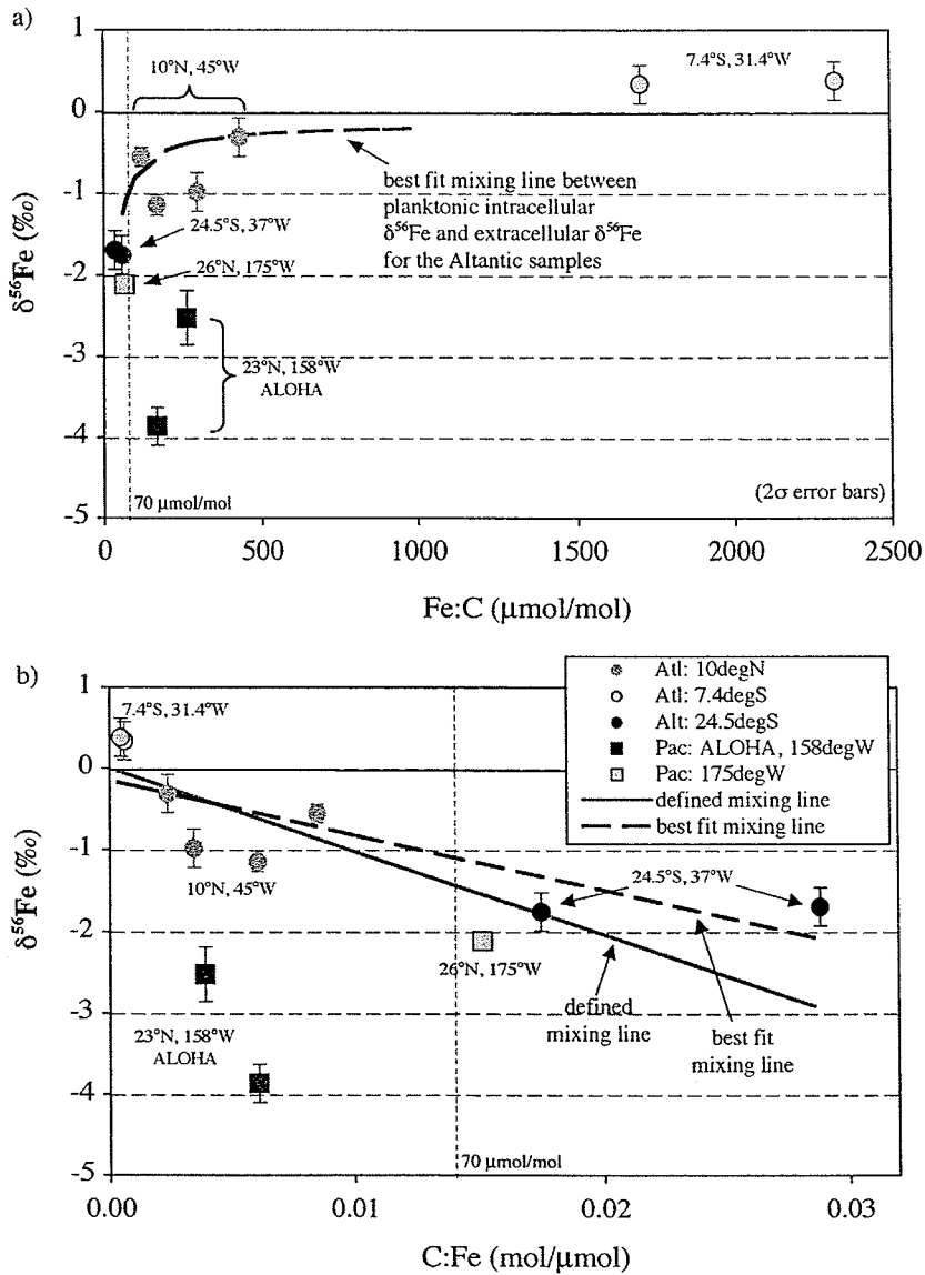
Figure 5.3: The \delta^{56}\text{Fe} measurements of plankton tow samples is plotted against their measured Fe:C ratios ( \mu\text{mol/mol} ) in Figure 5.3a and against C:Fe ( \text{mol}/\mu\text{mol} ) in Figure 5.3b. Hypothetical mixing lines are plotted for the Atlantic Ocean samples between an assumed planktonic intracellular endmember and an extracellular endmember (e.g., Fe/particles/colloids adsorbed to cell surfaces). It was assumed that all Fe in excess of a certain Fe:C ratio was extracellular. The best fit mixing line yielded an intracellular \delta^{56}\text{Fe} of -1.5\text{‰} , an extracellular endmember \delta^{56}\text{Fe} of -0.14\text{‰} , and a Fe:C threshold of 50 \mu\text{mol/mol} . A defined mixing line is also shown where the intracellular \delta^{56}\text{Fe} was set at -1.7\text{‰} (based on measurements of \delta^{56}\text{Fe} in plankton samples at 24.5^\circ\text{S} ) and the extracellular \delta^{56}\text{Fe} at 0\text{‰} (based on aerosol leachate measured in this study at 10^\circ\text{N}, 45^\circ\text{W} ). For the defined mixing line, it was assumed that all Fe in excess of a Fe:C ratio of 60 \mu\text{mol/mol} was extracellular. Error bars are 2\sigma standard errors of replicate measurements. If multiple measurements were not made within an analytical session, then a 2\sigma uncertainty of \pm 0.24\text{‰} is used based on the long-term external precision of a granite sample.
