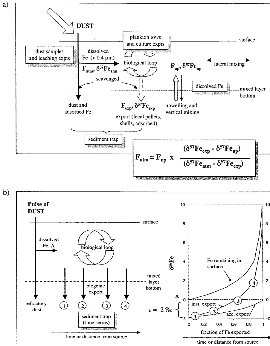
Figure 1.5: 1.5a) Hypothetical schematic of a steady state model for a Fe isotope application in the upper open ocean. The shadowed boxes highlight the type of samples that should be collected and measured for iron concentration and isotopic analysis. 1.5b) Hypothetical schematic of how Rayleigh fractionation could control the \delta^{56}\text{Fe} of different pools of Fe in the upper ocean. This model assumes a pulse of dust as the primary source of Fe to a region of the upper ocean. Iron is taken up by organisms and isotopically fractionated with an assumed fractionation of -2\text{‰} . As Fe is removed from surface waters over time by biologic export, the dissolved pool in the upper ocean becomes heavier. The graph shows the link between the fraction of the Fe from the pulse removed from the surface ocean and the \delta^{56}\text{Fe} of the remaining Fe in the mixed layer, the instantaneous export material, and the accumulated export. Material collected in sediment traps would reflect some combination of the instantaneous and accumulated products. This type of fractionation might also be observed as one moved laterally away from a source of iron (upwelling).
