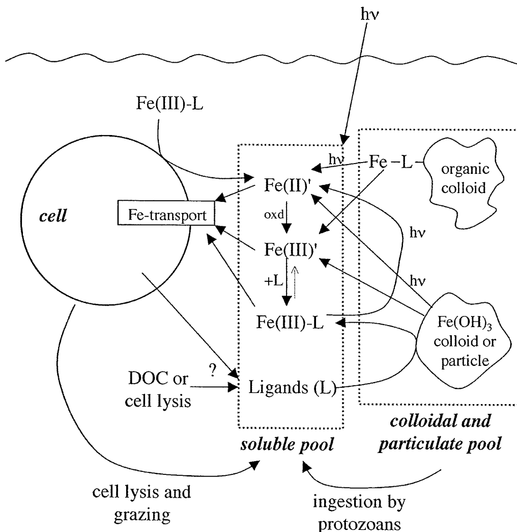
Figure 1.3: A schematic of potential pathways of biological utilization of various forms of Fe in seawater. The soluble pool of Fe includes the reactive inorganic species of Fe ( \text{Fe(II)'} and \text{Fe(III)'} ) along with organically bound Fe ( \text{Fe(III)-L} ) and excess dissolved ligand ( \text{L} ). Fe may also be bioavailable from the colloidal and particulate pools. Colloidal Fe may exist as either as inorganic colloids such as Fe oxyhydroxides or organic colloids. Fe may also be bioavailable in particulate forms such as amorphous Fe oxide coatings. Photochemical reduction of \text{Fe(III)} is noted by the pathways with \text{hv} next to the reaction arrow. The source and identification (?) of the ligands for Fe in seawater are not known, but they may be cell degradation products (e.g., porphyrin-type ligands) or be produced by organisms to specifically bind Fe (e.g., siderophore ligands). Not shown in this figure is the role of \text{Fe(II)} ligands, the various mechanisms for Fe transport across the cell membrane, or bacteria or colonies living on particles and creating micro-environments that enhance Fe solubilization. See text for more discussion. Reviews of the potential pathways for Fe utilization can be found in Sunda (2001) and Moffet (2001).
