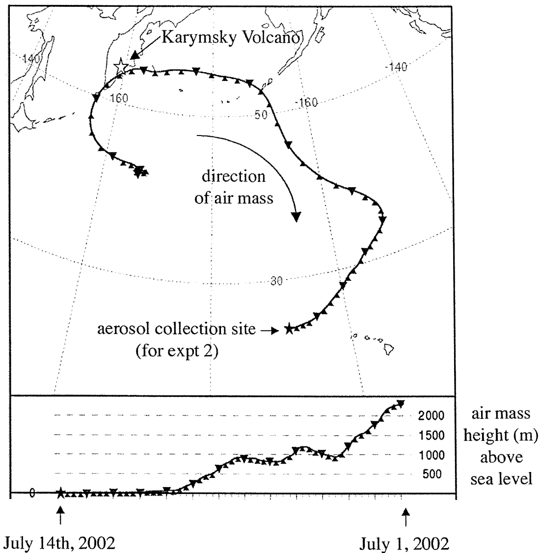
Figure 3.2: A two week modeled back trajectory for the aerosol sample used in the dissolution experiment #2. The aerosol sample was collected for 9 hours on July 14, 2002 by Y. Chen and R. Siefert (University of Maryland). The aerosol sample collection end point was 24.2°N, 168.6°W. Modeled back trajectories for the aerosol sampled used in experiment 2 were very similar (July 13 th ; 25.6°N, 173.4°W). Back trajectories were calculated by the HYSPLIT (HYbrid Single-Particle Lagrangian Integrated Trajectory) Model (DRAXLER and ROLPH, 2003). The author gratefully acknowledges the NOAA Air Resources Laboratory (ARL) for the provision of the HYSPLIT transport and dispersion model and/or READY website used in this publication ( http://www.arl.noaa.gov/ready/hysplit4.html ). The location of a volcano that was active just before the sampling period (June 28 to July 1, 2002) is also shown (Karymsky Volcano).
