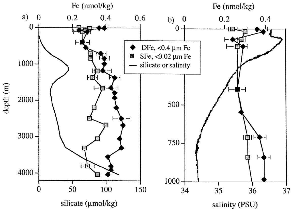
Figure 2.6: DFe and SFe profiles for the South Atlantic station at 24.5°S, 37°W occupied in March 2002. Figure 2.6a is the full Fe profile to 4000 m plotted along with silicate data measured on the same cruise. Figure 2.6b is a blow up of the upper 1000 m plotted along with CTD salinity data. Error bars are 1σ standard deviation of sample replicates (external reproducibility typically less than \pm 0.05 nmol/kg (1 SD) for Fe).
