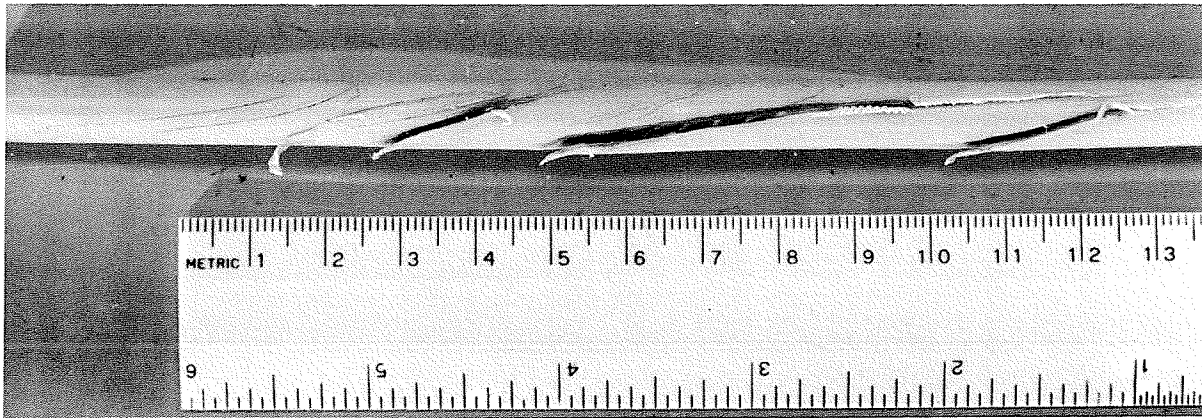
Figure 1.3 Fishbite on plastic jacket of steel wire rope (Prindle and Walden, 1975).
