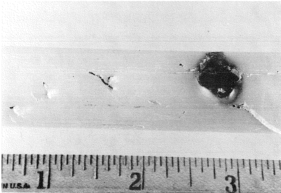
Figure 2.3 Shark teeth in heated polyethylene jacket. The black hole resulted from a short circuit.
