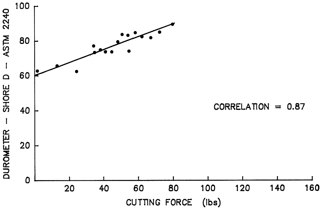
Figure 5.7 Durometer D versus cutting force.
