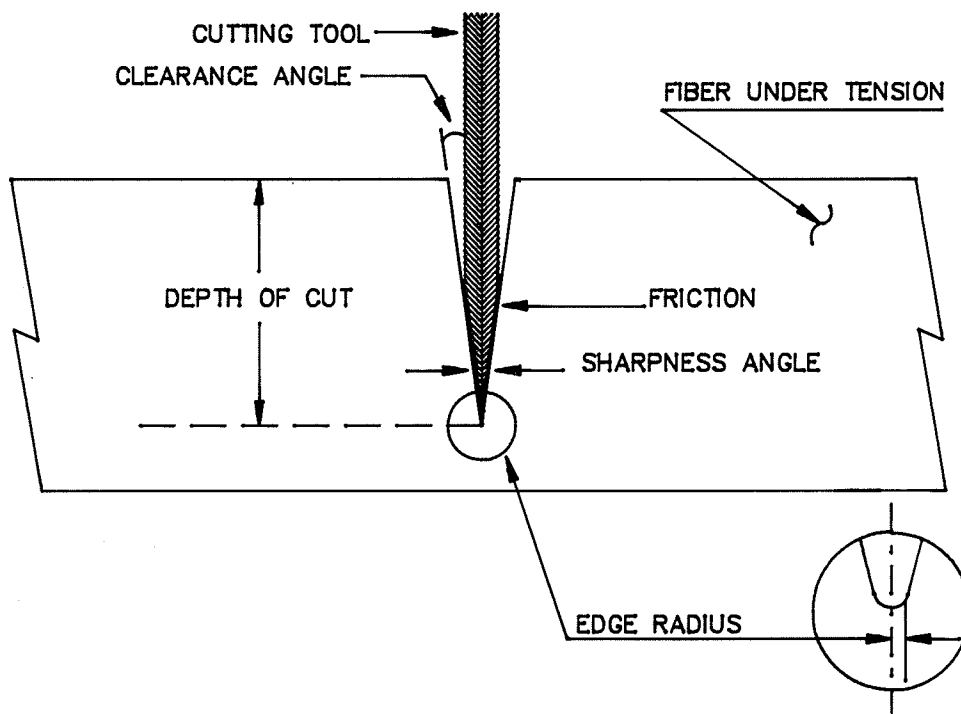
Figure 5.3 Mechanics of cutting (Barkas, et al., 1932).
