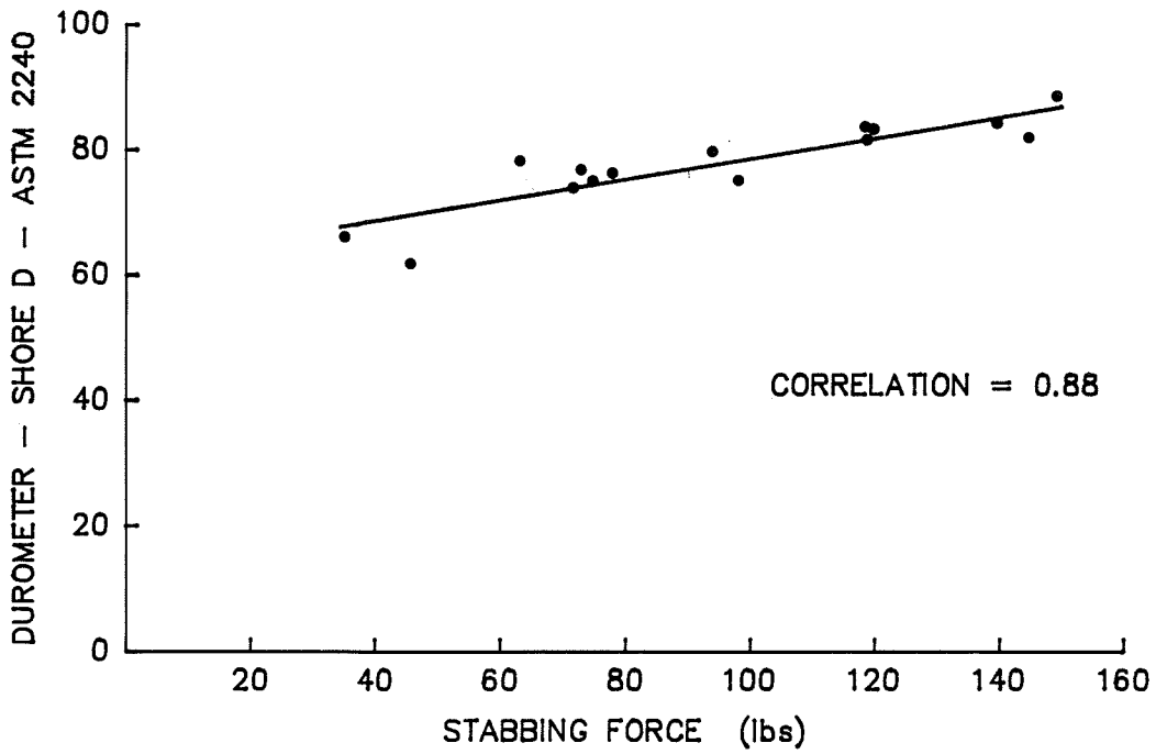
Figure 5.6 Durometer D versus stabbing force.
