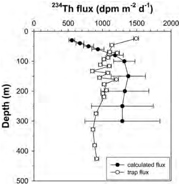
Figure 5.1. An example of fluxes calculated from water column ^{234}\text{Th} data in comparison to ^{234}\text{Th} fluxes measured by using free-drifting cylindrical traps on a single surface-tethered array in the subarctic Western Pacific during spring (May) 1998 (K. Harada, unpublished data). The traps slightly under-collect ^{234}\text{Th} in comparison to calculated fluxes, except just below the upper mixed layer ( \sim 25\text{m} deep during the experiment) where over-collection occurred. Error bars for the trap flux are from counting errors in the ^{234}\text{Th} analyses, whereas error bars for the calculated flux are derived from the error on the difference between total ^{238}\text{U} and ^{234}\text{Th} activities.
