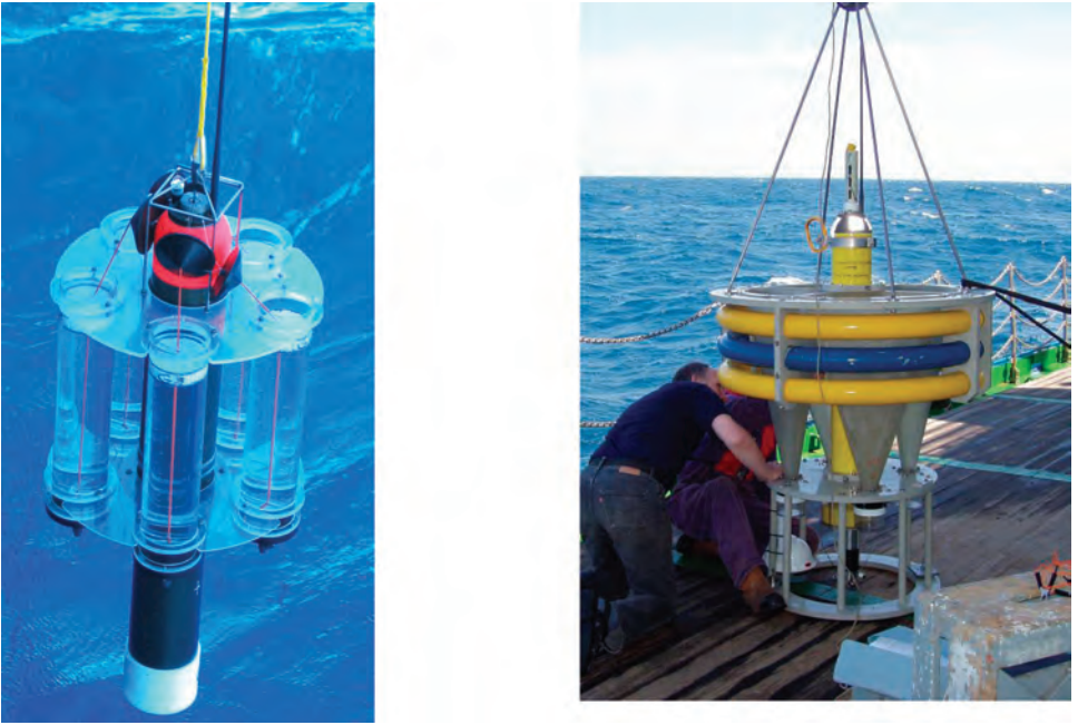
Figure 2.3. Photos of two neutrally buoyant traps used successfully to collect sinking particles in the ocean. (a) NBST (Valdes and Price, 2000; Valdes and Buesseler, 2006). (b) PELAGRA (Lampitt et al. , 2004).
